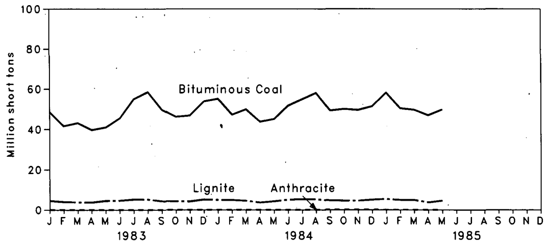
Coal Consumption
