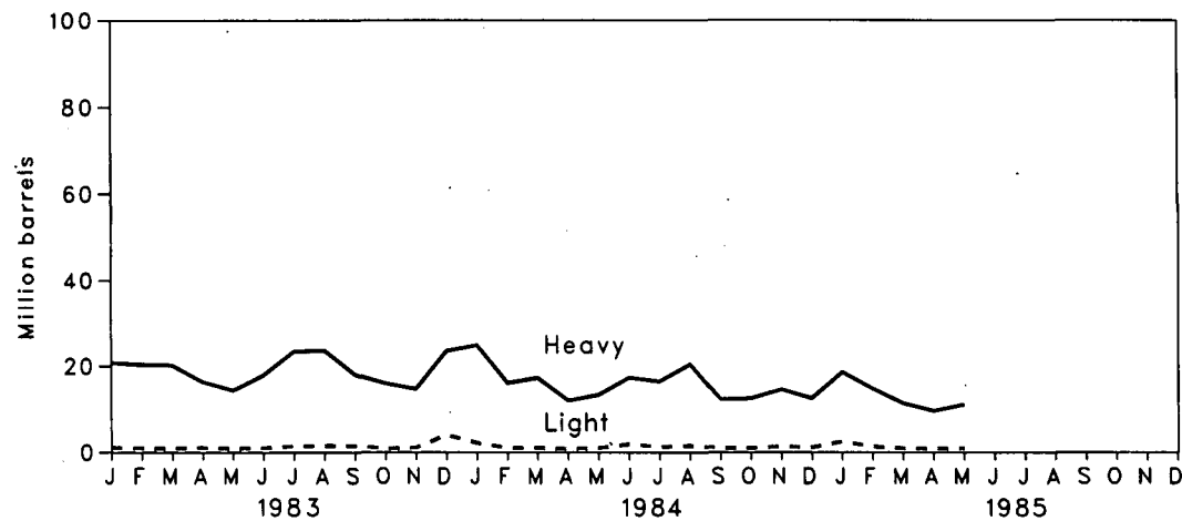
Petroleum Consumption
