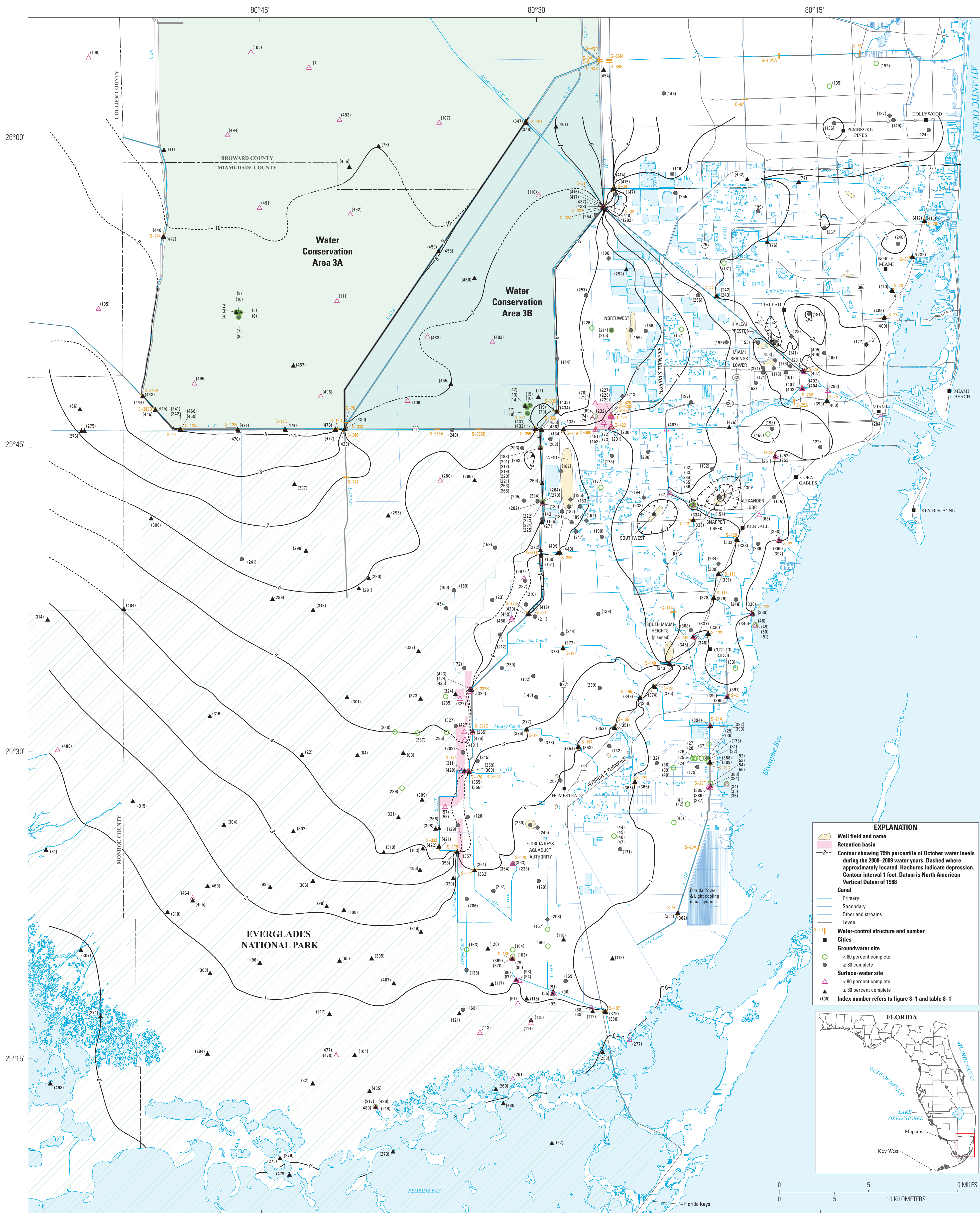
75th Percentile of October Water Levels During the 2000-2009 Water Years, Miami-Dade County, Florida
