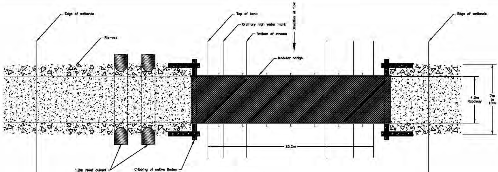
Top View
