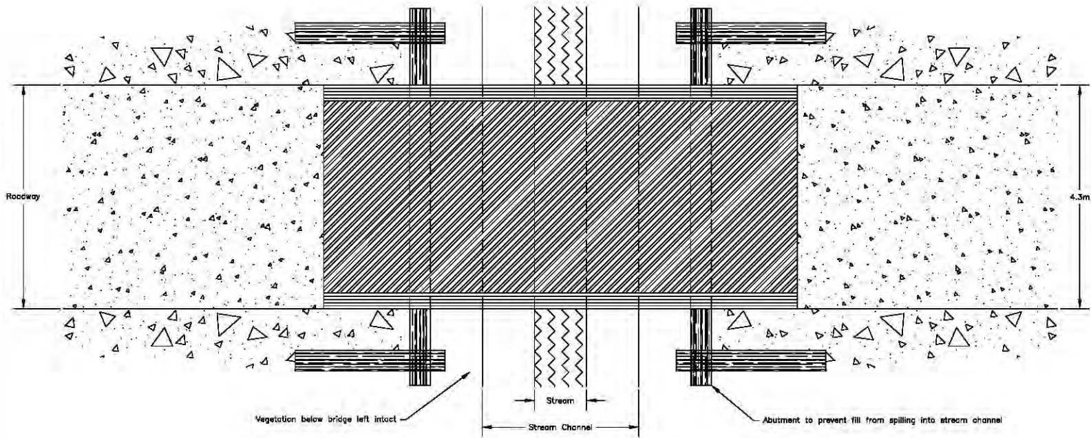
Top View
