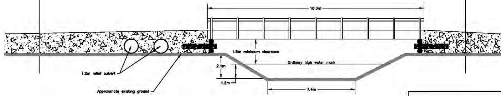
Front View
