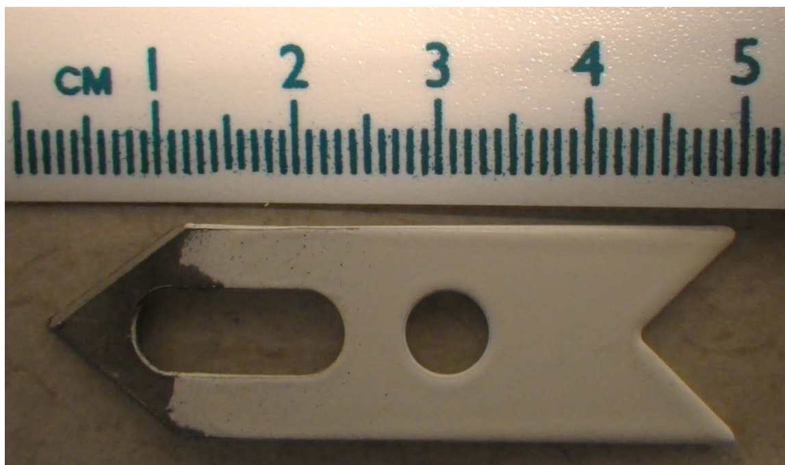
Figure 4. -- Photo of the stainless steel darheads used in Method 1. These darheads are 316L surgical grade stainless steel with sharpened edge 1 inch in length.
