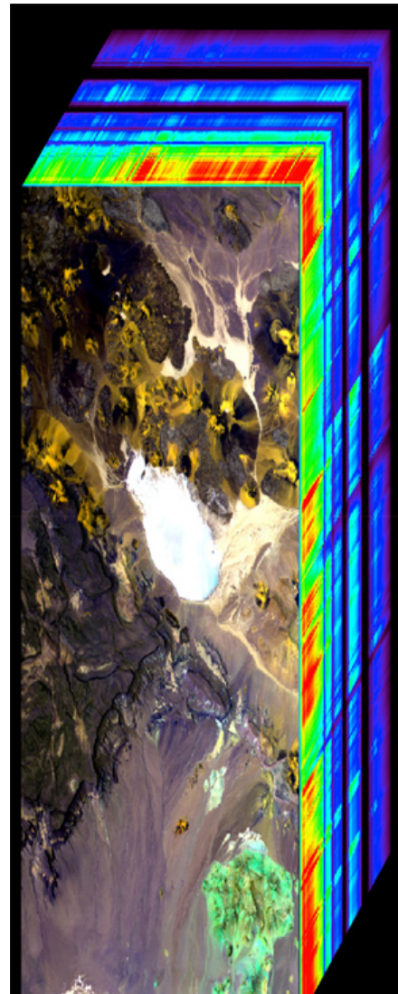
Figure 4: Lunar Lake, NV Calibration site measured by AVIRIS from 65,000 feet on August 19, 2009.
