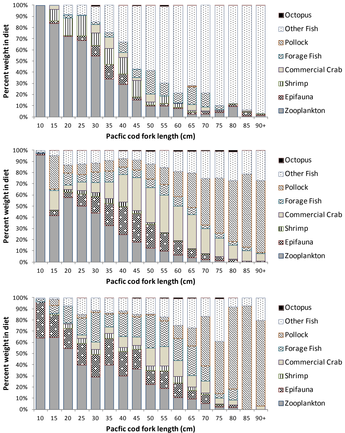
Figure 22.A1.3. Percent diet by weight in Pacific cod stomachs sampled in water <100m, all years and seasons, for Aleutian Islands (top panel), Bering Sea (middle panel), and Gulf of Alaska (bottom panel).
