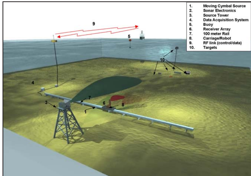
Depiction of the 100-m-long rail deployed in shallow water together with the source tower, data acquisition system, RF link to surface vessel, and scattering targets
