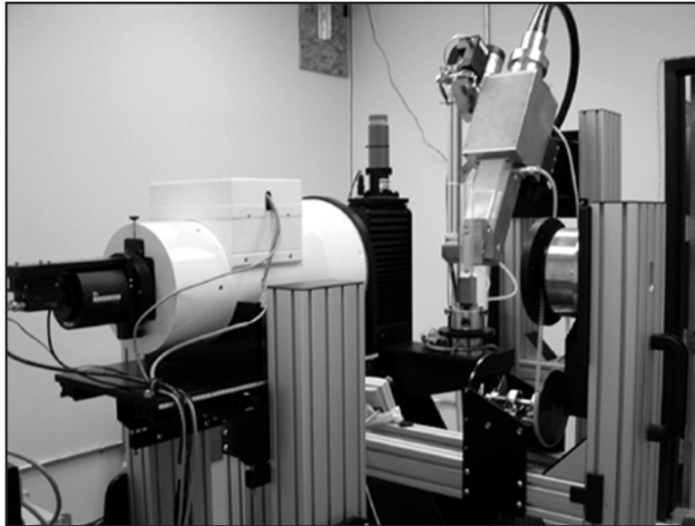
The X-ray system portion of the HD-500 Micro-CT System
