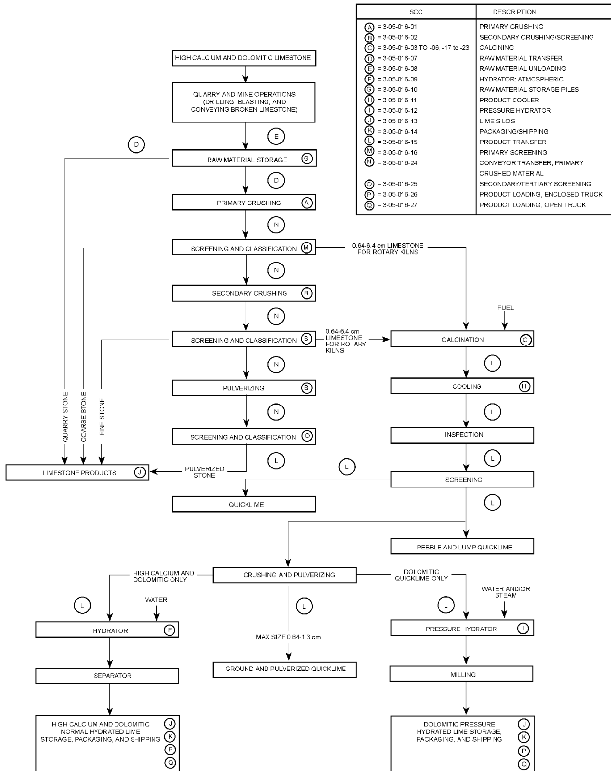
Figure 2-1. Process flow diagram for lime manufacturing. 4
