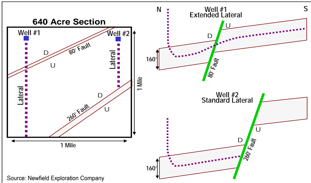
Figure 2-13. 3D Seismic Helps Design Extended vs. Limited Length Lateral Wells
