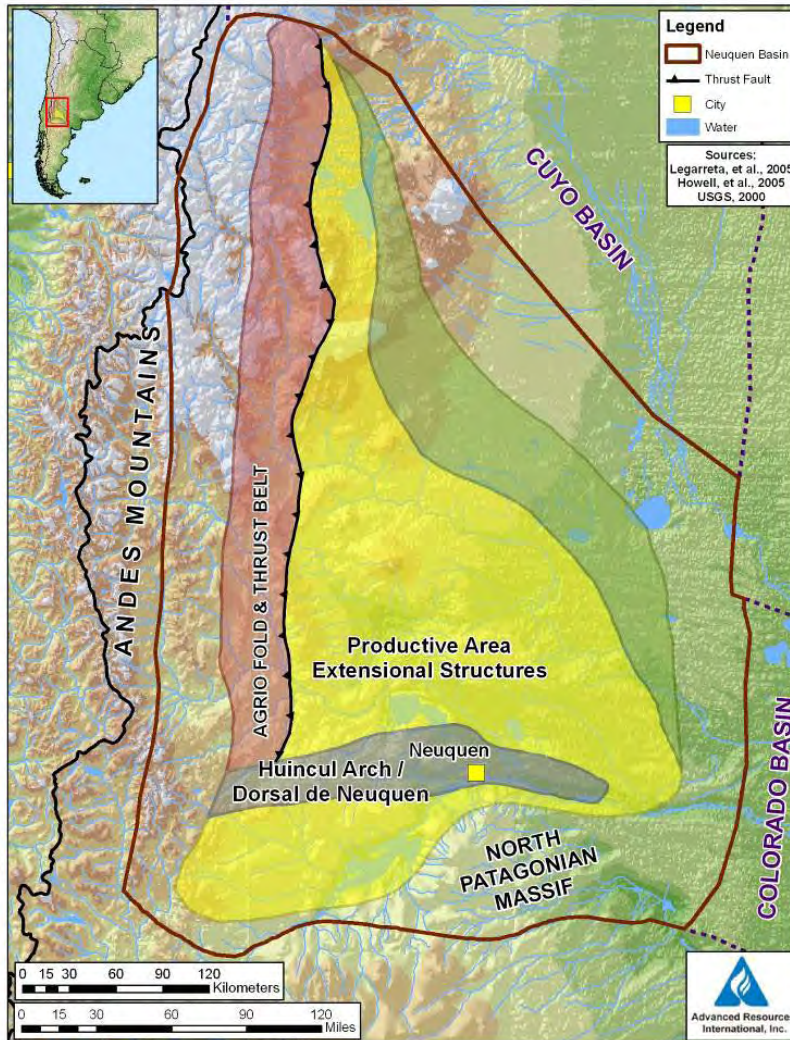
Figure IV-2. Neuquen Basin Shale Gas Prospective Area and Basemap
