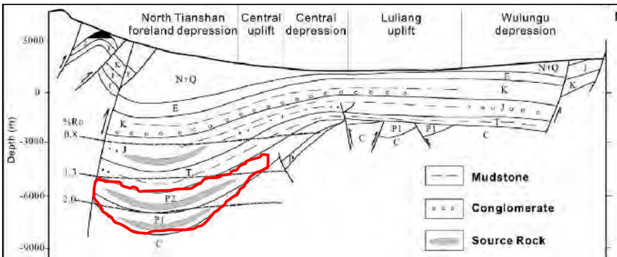
Figure XI-16. Junggar Basin Source-Rock Shales in the Jurassic and Permian
