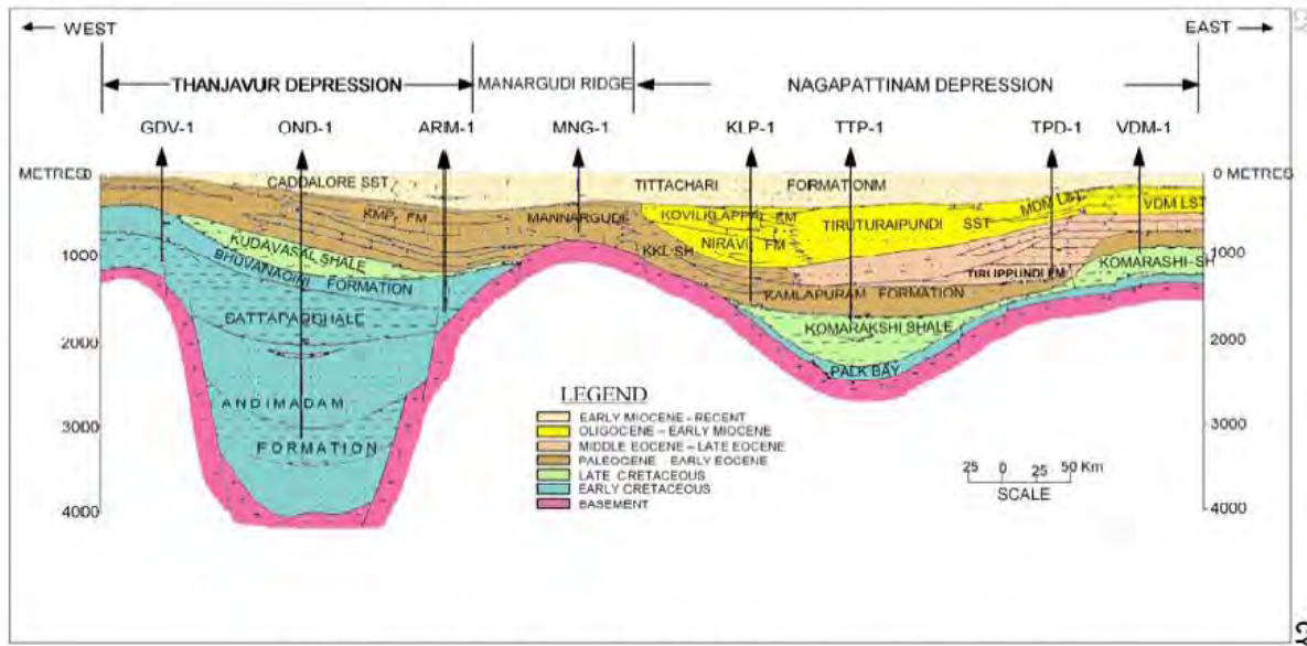
Figure XII-19. Thanjavur Sub-Basin and Geological Section Across Cauvery Basin.
