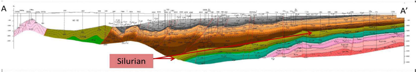
Figure VI-10. Lublin Basin Geology and Cross Section9
