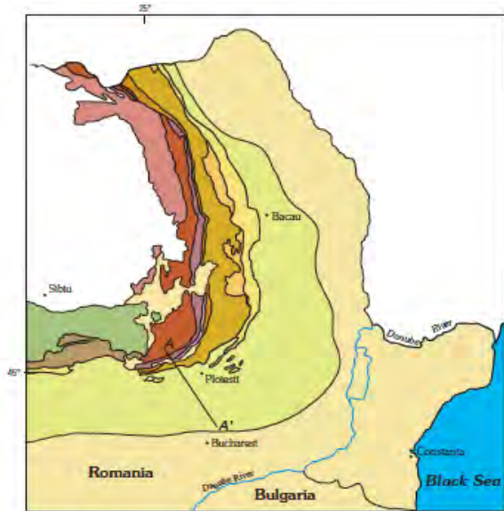
Figure VI-16. Carpathian-Balknian Basin Component Map 13
