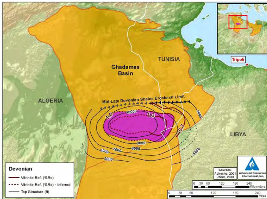
Figure VIII-5. Devonian Frasnian Vitrinite Reflectance
