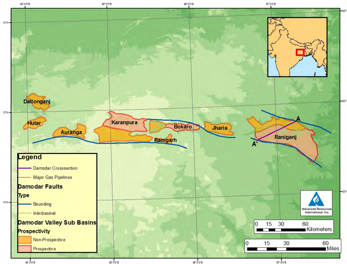
Figure XII-20. Damodar Valley Basin and Prospectivity for Shale Gas
