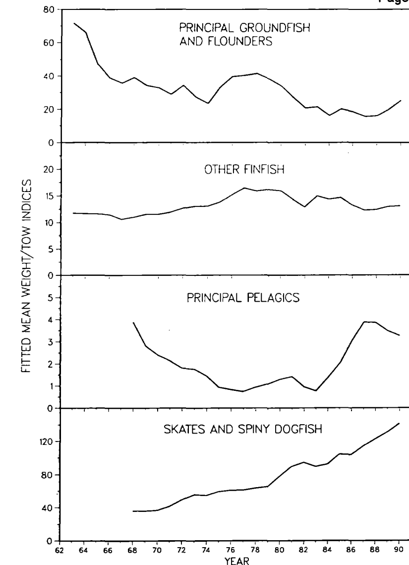
Figure 3. Trends in indexes of aggregate abundance (catch in weight per survey trawl haul) for four species groups, reflecting the major changes in fishery resources, 1962-1990.
