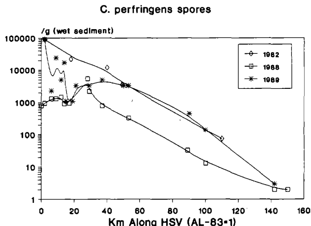
Figure 35. Trends in Clostridium perfringens spores along the Christiaensen Basin-HSV transect prior to (Cabelli and Pederson 1982), and after (1988-89), cessation in sludge disposal.
