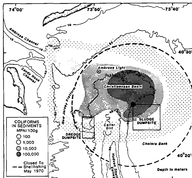
Figure 1. Location of the 12-mile dumpsite, dredge materials dumpsite, and area closed to commercial shellfishing in the NYB (after Verber 1976).
