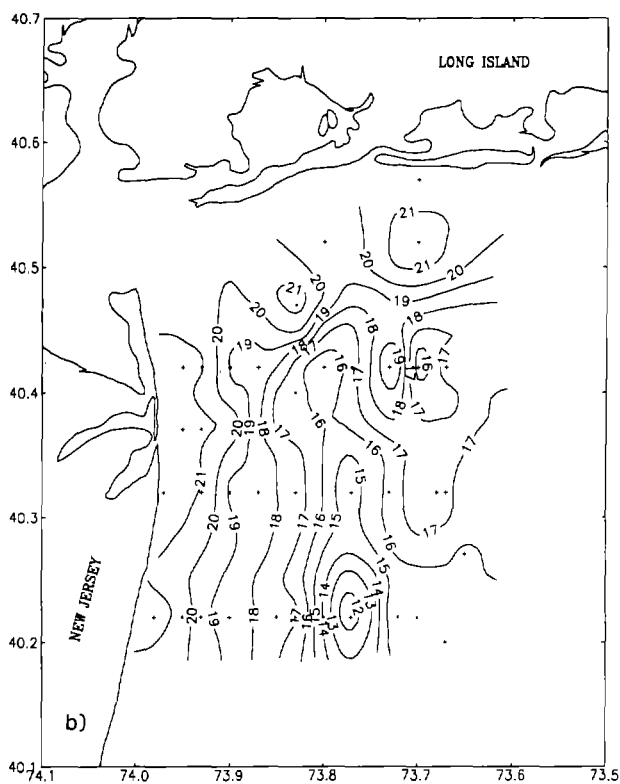
Figure 27. Surface (a) and bottom (b) temperature ( ^{\circ}\text{C} ) during the second survey of the inner NYB on cruise Oregon II 89-04, August 12-22, 1989.
