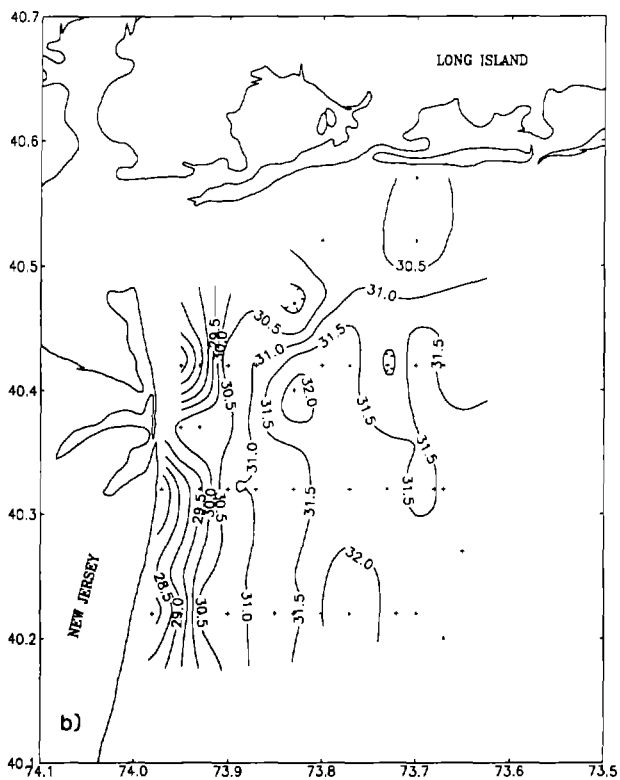
Figure 28. Surface (a) and bottom (b) salinity (PSU) during the second survey of the inner NYB on cruise Oregon II 89-04, August 12-22, 1989.
