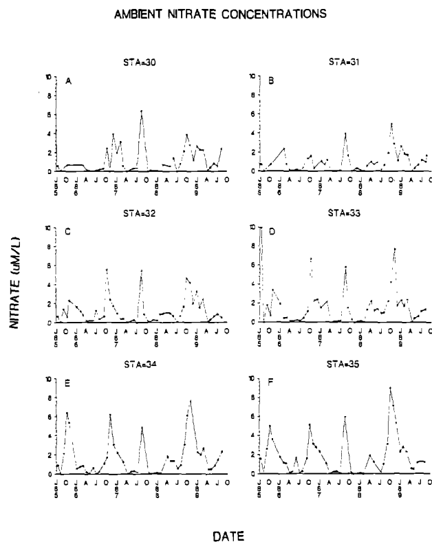
Figure 52. Concentrations ( \mu\text{M/l} ) of nitrate measured at 0.5 m depth at: (a) station 30, (b) station 31, (c) station 32, (d) station 33, (e) station 34, and (f) station 35 from July 1985 through August 1989.
