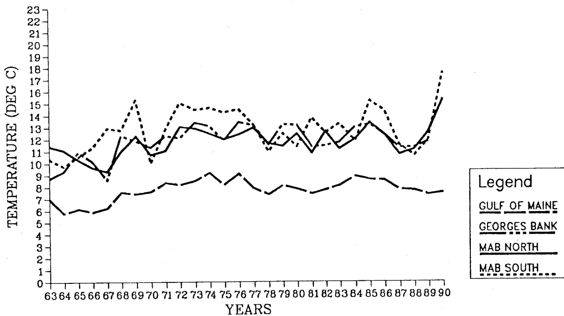
Figure 8. Average bottom temperature in the four regions of the shelf shown in Figure 1 of NEFC Reference Document 90-03 for the spring (top) and the fall (bottom). Additional data (1988-1990) are listed in Table 1.
