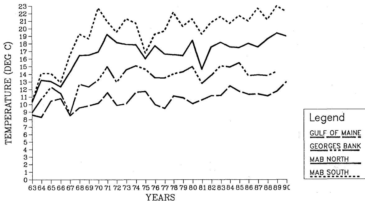
Figure 7. Average surface temperature in the four regions of the shelf shown in Figure 1 of NEFC Reference Document 90-03 for the spring (top) and the fall (bottom). Additional data (1988-1990) are listed in Table 1.
