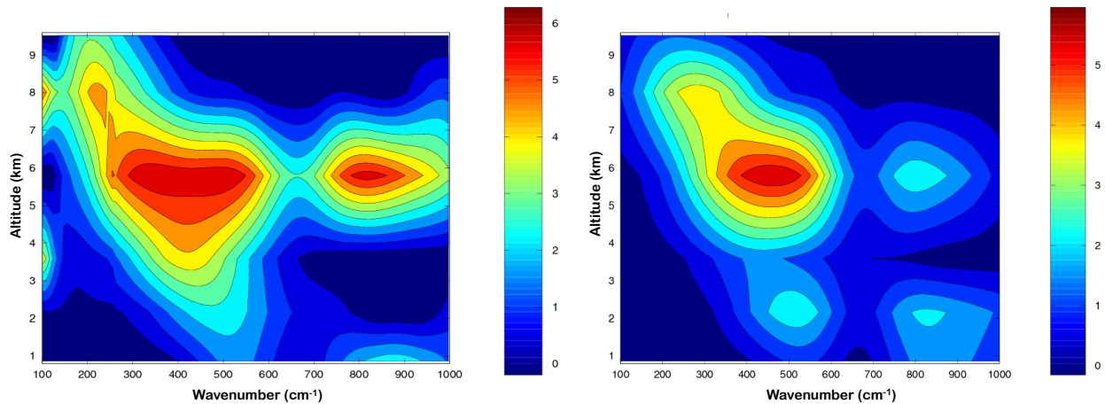
Figure 4.17: INFRARED COOLING RATE RESULTS FROM THE INFLAME TECHNOLOGY DEMONSTRATION FLIGHT IN JANUARY, 2010: CALCULATED INFRARED COOLING RATES ( \text{MK}/\text{DAY}/\text{CM}^{-1} ) (LEFT), AND MEASURED INFRARED COOLING RATES (RIGHT).
