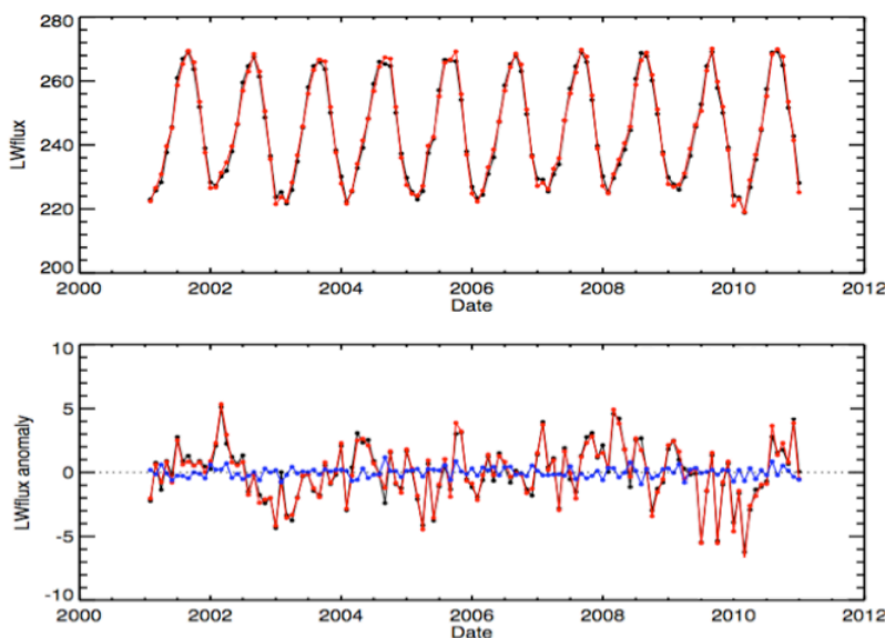
Figure 2.5: TOP: THE MONTHLY 2001 TO 2011 30^\circ TO 40^\circ ZONAL MEAN CERES (BLACK LINE) AND P90 SAMPLED (RED LINE) LW FLUX ( Wm^{-2} ). BOTTOM: THE ASSOCIATED CERES (BLACK LINE), P90 (RED LINE), AND SAMPLING ERROR (BLUE LINE) LW FLUX ANOMALY ( Wm^{-2} ) AFTER DE-SEASONALIZATION.
