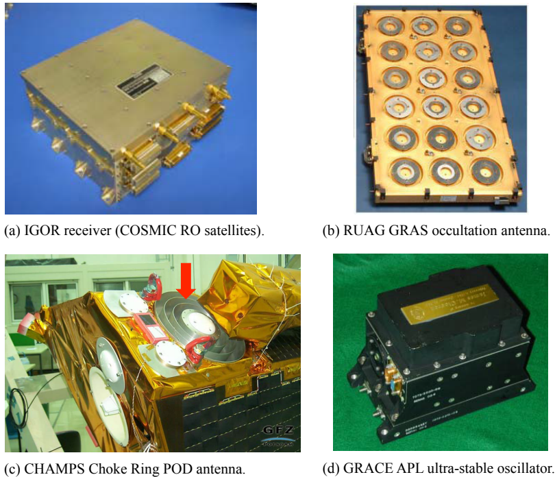
Figure 4.9: THE GNSS-RO SUITE COMPONENTS WITH HERITAGE: A) IGOR RECEIVER USED ON THE COSMIC RADIO OCCULTATION SATELLITES, B) GRASS OCCULTATION ANTENNA, C) CHOKE RING POD ANTENNA ON CHAMP OBSERVATORY, D) APL ULTRA-STABLE OSCILLATOR FOR GRACE MISSION.
