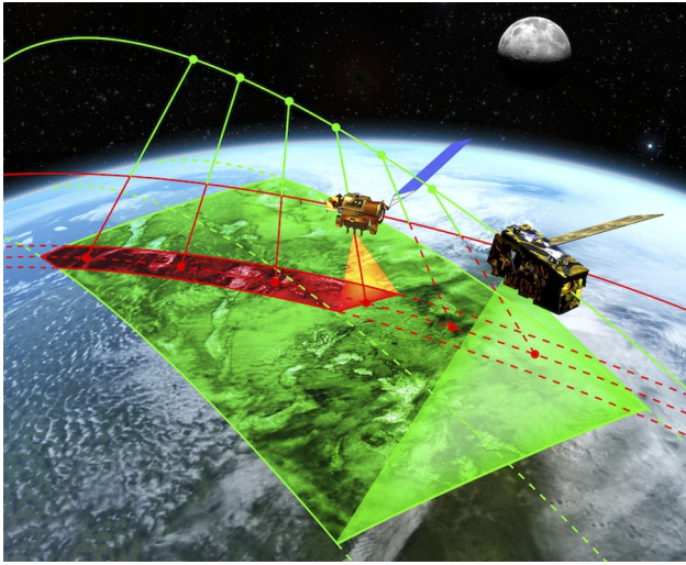
Figure 2.33: AS THE CLARREO ORBIT, AT 609 KM ALTITUDE (RED), CROSSES THAT OF A SATELLITE SUCH AS SUOMI NPP (GREEN) WITH AN OPERATIONAL SENSOR (E.G CERES, VIIRS), THE CLARREO REFLECTED SOLAR SPECTROMETER COLLECTS DATA MATCHED IN TIME, SPACE, AND VIEW ANGLES TO PROVIDE A REFERENCE INTER-CALIBRATION STANDARD FOR THE TARGET SENSORS. TO MATCH VIEWING ANGLES WITH THE TARGET INSTRUMENT, AND TO MAXIMIZE THE INTER-CALIBRATION SAMPLING, THE CLARREO REFLECTED SOLAR SPECTROMETER HAS 2-DIMENSIONAL POINTING ABILITY (ROLL OVER AZIMUTH GIMBAL).
