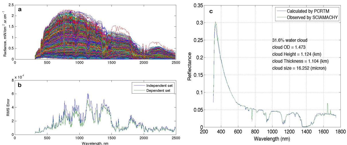
Figure B.3: a) SELECTED TOA RADIANCE SPECTRA UNDER DIFFERENT OBSERVATION GEOMETRY AND ATMOSPHERIC AND SURFACE CONDITIONS. b) THE RMS ERROR OF PCRTM CALCULATED RADIANCE SPECTRAL RELATIVE TO THOSE CALCULATED USING MODTRAN. c) COMPARISON OF A PCRTM CALCULATED TOA REFLECTANCE SPECTRUM WITH THAT OBSERVED FROM THE SCIAMACHY INSTRUMENT. THE ATMOSPHERIC AND SURFACE PROPERTIES USED BY THE PCRTM ARE DERIVED FROM THE CERES LEVEL-2 PRODUCTS.
