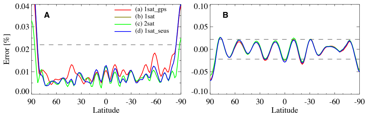
Figure 2.9: SUMMARY OF STATISTICS OF RADIO OCCULTATION SAMPLING ERROR. FOR EACH OF THE FOUR CONFIGURATIONS LISTED IN THE TEXT – (A) ONE CLARREO SATELLITE RECEIVING GPS SIGNALS ONLY, (B) ONE CLARREO SATELLITE RECEIVING GPS AND GALILEO SIGNALS, (C) TWO CLARREO SATELLITES RECEIVING GPS AND GALILEO SIGNALS, AND (D) ONE CLARREO SATELLITE TRACKING GPS AND GALILEO BUT SUBJECT TO SINGULAR EVENT UPSETS – BOTH THE RANDOM ERROR (A) AND SYSTEMATIC ERROR (B) ARE SHOWN. ALL STATISTICS ARE FOR ZONAL AVERAGE, WITH AN ANNUAL AVERAGE MICROWAVE REFRACTIVITY AT 18 KM GEOPOTENTIAL HEIGHT. THE DASHED LINES ARE THE LEVEL 1 REQUIREMENTS ON RANDOM SAMPLING ERROR FOR REFRACTIVITY AT 18 KM, WHICH IS 0.022%.
