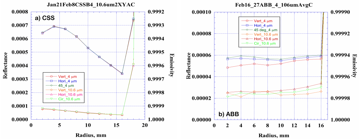
Figure 4.40: NIST CHILR CAVITY REFLECTANCE VERSUS POSITION AT A WAVELENGTH OF 10.6 μm PROVIDED TO NASA FOR (A) CSS AND (B) ABB. FOR REFERENCE, THE RIGHT HAND SCALE FOR EACH PLOT SHOWS EMISSIVITY COMPUTED FROM 1 – REFLECTANCE.
