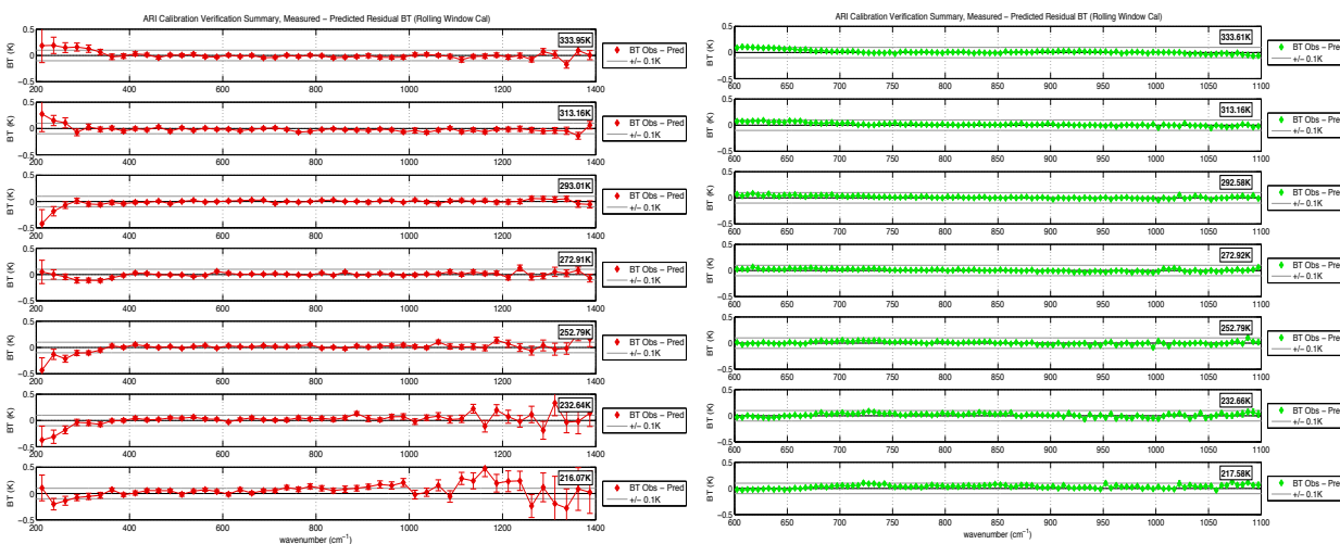
Figure 4.29: ARI CALIBRATION VERIFICATION. OBSERVED – PREDICTED OARS BRIGHTNESS TEMPERATURE RESIDUALS AVERAGED OVER 25 \text{cm}^{-1} FOR NOISE REDUCTION FOR THE DTGS DETECTOR (LEFT) AND AVERAGED OVER 5 \text{cm}^{-1} FOR THE MCT (RIGHT). THE DIFFERENCES GENERALLY FALL INSIDE THE \pm 0.1 K BOUNDARIES SHOWN. IN THE FARIR, FROM 200 – 300 \text{cm}^{-1} , THE LOW SIGNAL-TO-NOISE DUE TO THE LESS THAN OPTIMUM BEAMSPLITTER COATING CAUSES A SMALL BIAS. THE COLDEST SHORTWAVE REGIONS ALSO SHOW SOME SMALL BIASES DUE TO LOW SIGNAL-TO-NOISE (THE NOISE LEVEL OF THE TESTS IS A FACTOR OF 4 LARGER THAN THE ON-ORBIT NOISE SPECIFICATION DUE TO SHORTER DWELL TIMES).
