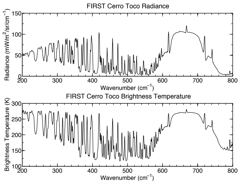
Figure 4.13: FIRST RADIANCE RECORDED AT CERRO TOCO, CHILE UNDER EXCEPTIONALLY LOW PRECIPITABLE WATER VAPOR CONDITIONS ( PW < 1 MM).
