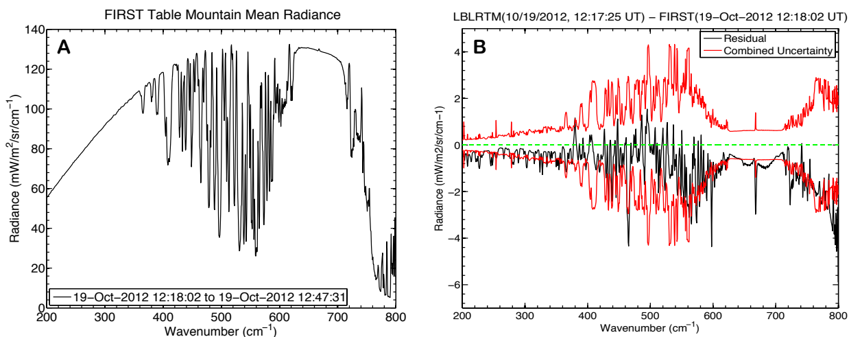
Figure 4.14: A) FIRST RADIANCE SPECTRUM RECORDED AT TABLE MOUNTAIN ON 19 OCTOBER 2012. PRECIPITABLE WATER VAPOR AMOUNTS WERE 0.28 CM. B) DIFFERENCE BETWEEN FIRST MEASUREMENTS AND RADIATIVE TRANSFER CALCULATIONS (RESIDUAL, BLACK CURVE) AND THE UNCERTAINTY IN THE DIFFERENCE (COMBINED UNCERTAINTY, RED CURVE), FOR SPECTRA RECORDED AT TABLE MOUNTAIN CALIFORNIA, OCTOBER, 2012.
