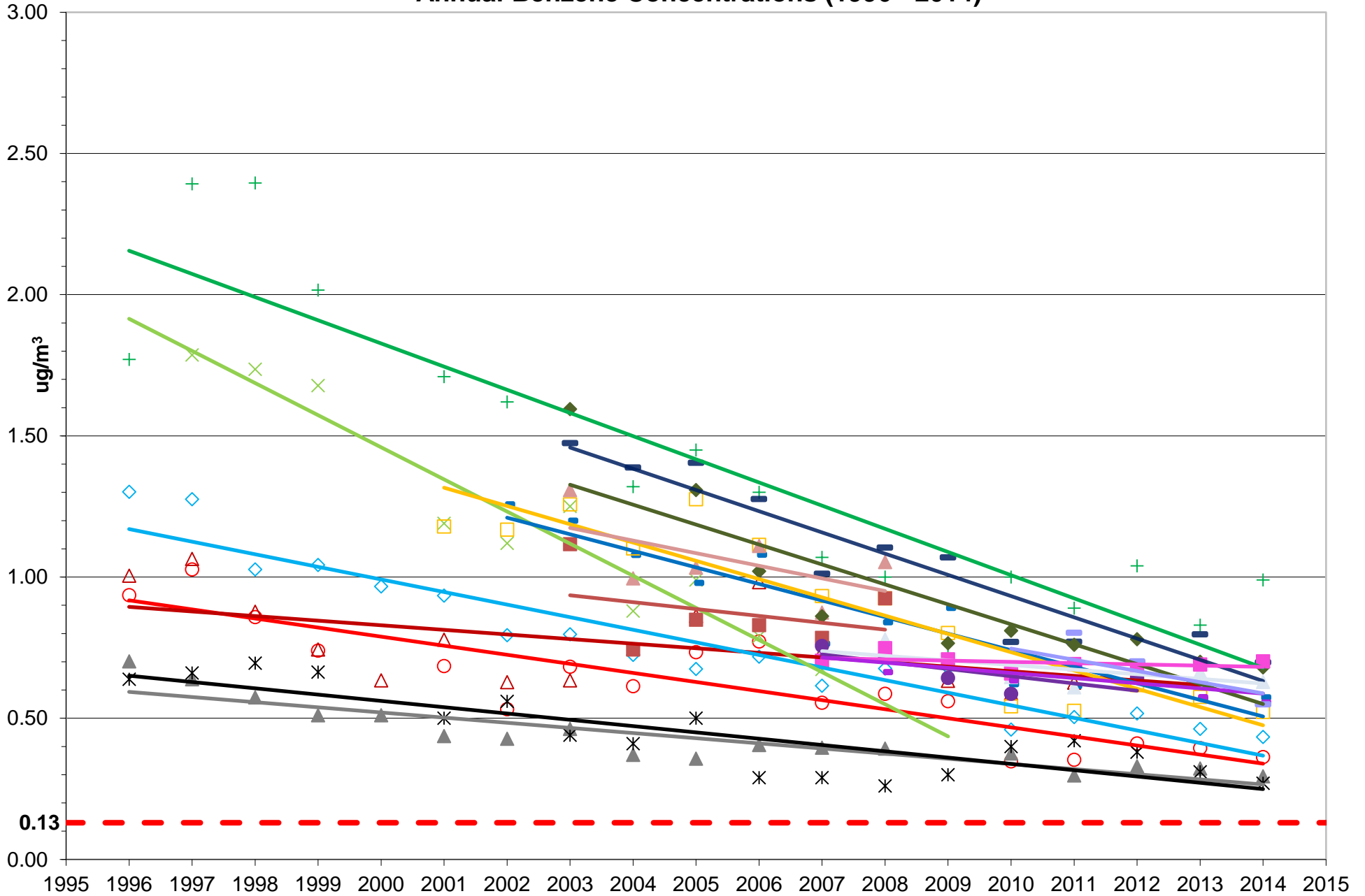
Annual Benzene Concentrations (1996 - 2014)
