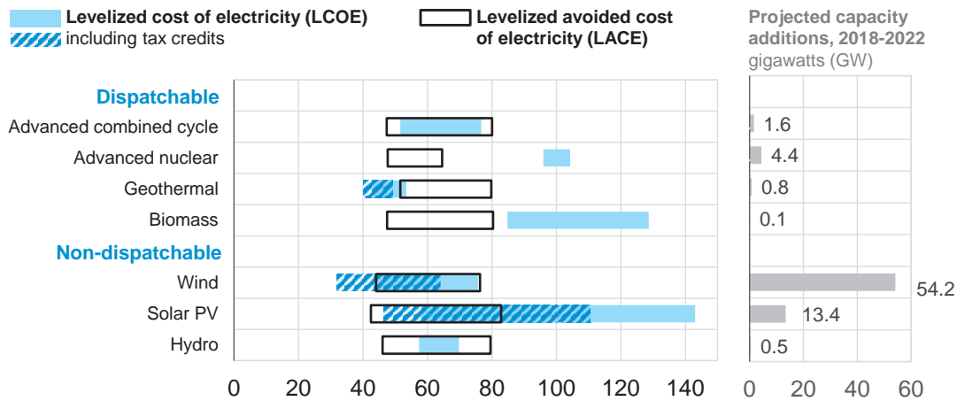
Levelized cost projections by technology, 2022 2016 dollars per megawatthour
