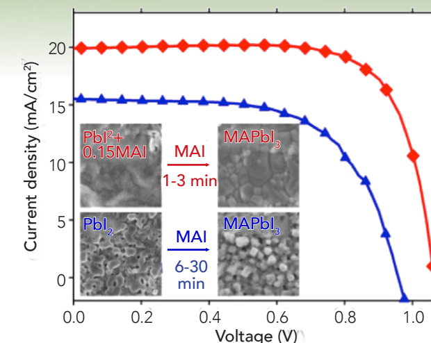
Demonstration of morphology control, faster phase formation, and increased efficiency by controlling the precursor chemistry of the perovskite films (T. Zhang, et al., 2015)
