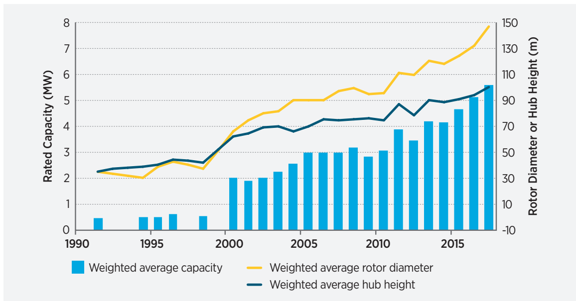
Figure 2-31. Average turbine size, rotor size, and hub height for commercial offshore wind parks
