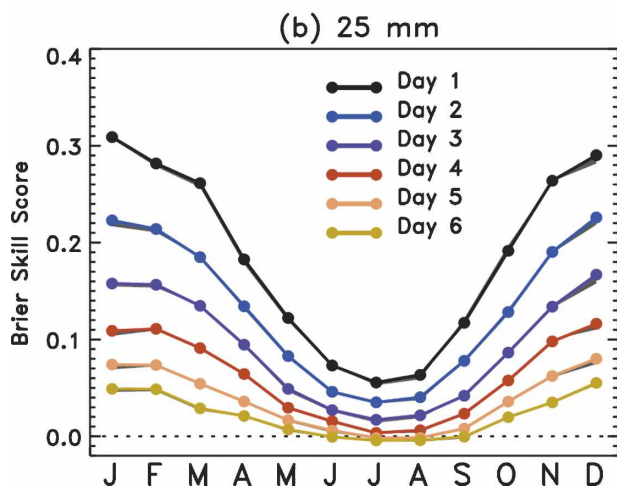
FIG. 11. Monthly BSS of the basic technique including precipitable water, with skill again compared via shading relative to the basic analog technique in Fig. 8.
