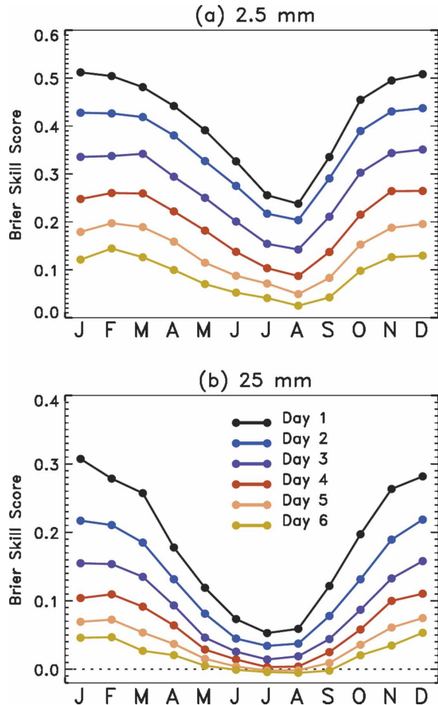
FIG. 8. BSS of the basic analog technique as a function of the month and the lead time of the forecast: (a) Skill at 2.5 mm and (b) skill at 25 mm.
