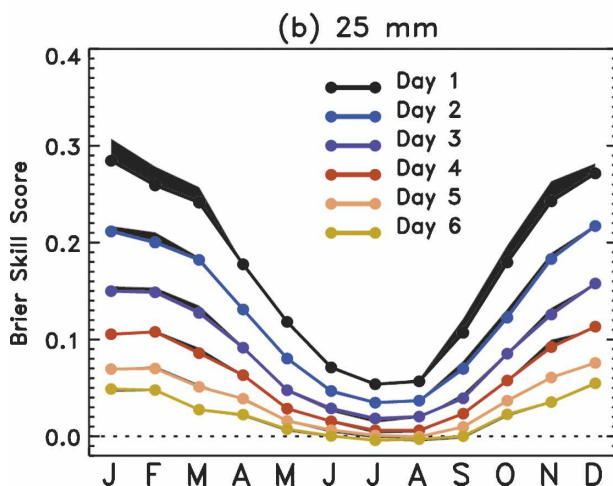
FIG. 12. Monthly BSS of the basic technique including 2-m temperatures and 10-m winds, with skill again compared via shading relative to the basic analog technique in Fig. 8.
