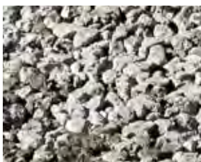
Pervious concrete
