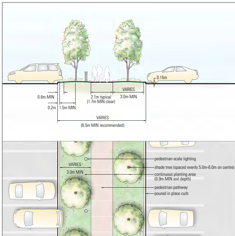
Design concept for pedestrian pathway with double row of shade trees (See 4.3 Pedestrian Access and Circulation)
