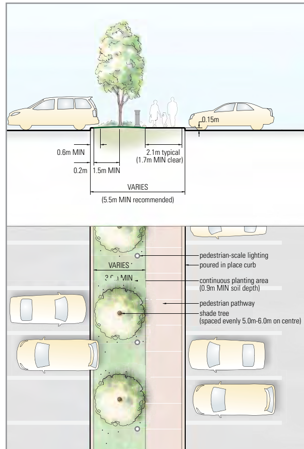
Design concept for pedestrian pathway with single row of shade trees. Note: See 5.2 Additional Diagrams for further design options
