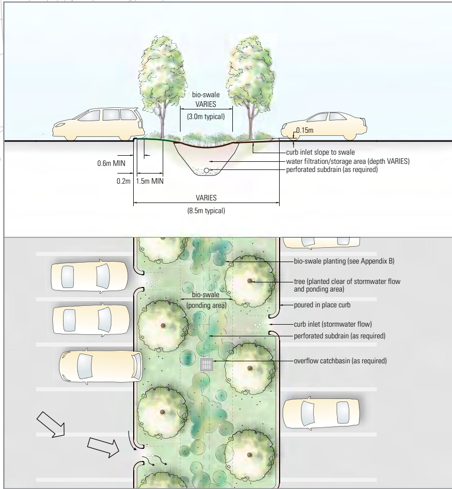
Design concept for bio-retention swale with double row of trees (See 4.5 Stormwater Management)
