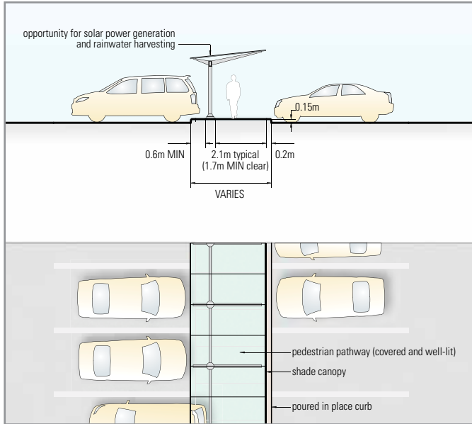
Design concept for pedestrian pathway with shade structure (See 4.3 Pedestrian Access and Circulation)
