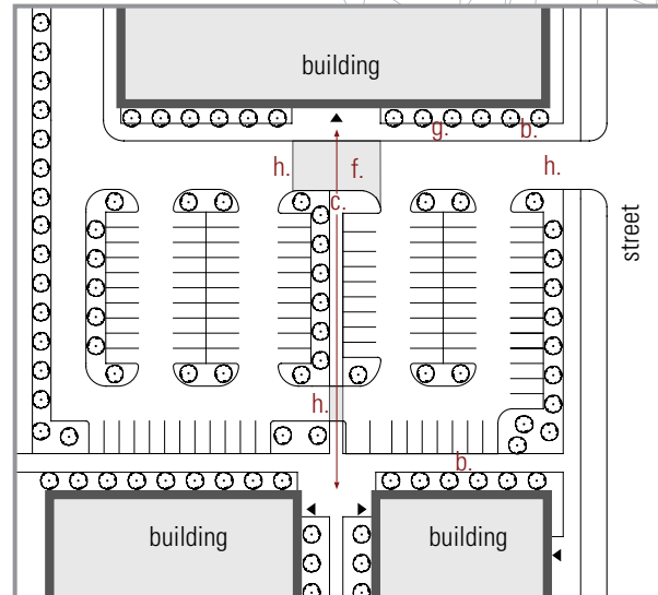
Conceptual pedestrian access and circulation scheme Note: Letters correspond to guidelines in sub-section 4.3
