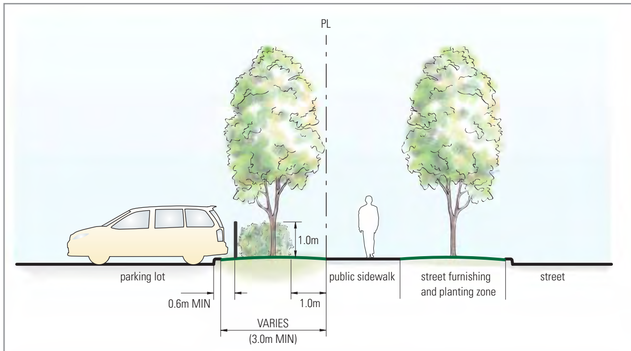
Design concept for street facing parking lot edge
