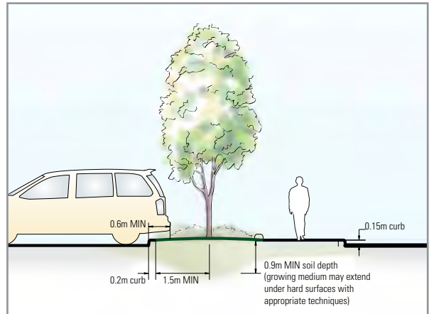
Design concept for pedestrian pathway with single row of shade trees. Note: See 5.2 Additional Diagrams for further design options.
