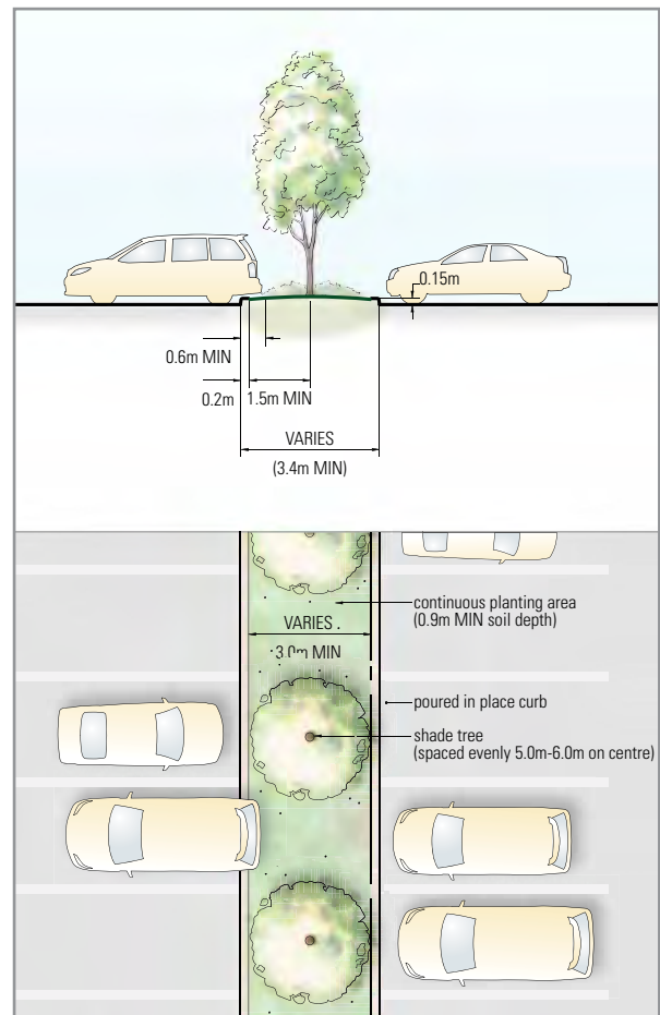
Design concept for landscaped median with shade trees
