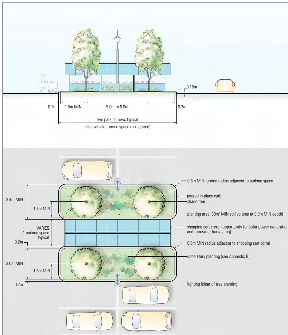
Design concept for mid-row landscaped islands and shopping cart corral (See 4.1.4 Other Site Elements and 4.4.3 Internal Landscaping)
