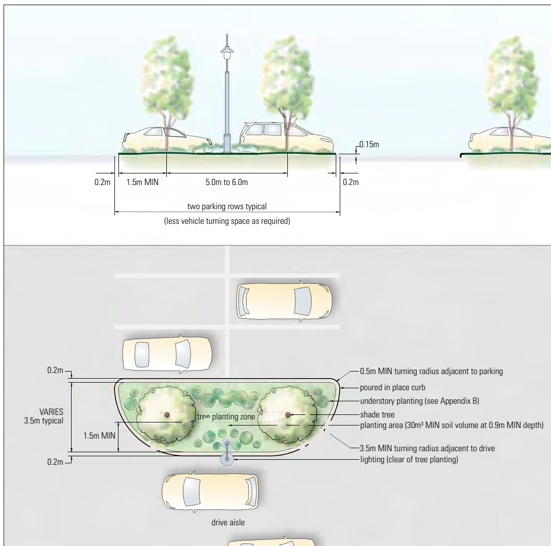
Design concept for end-of-row island with shade trees and understory planting
