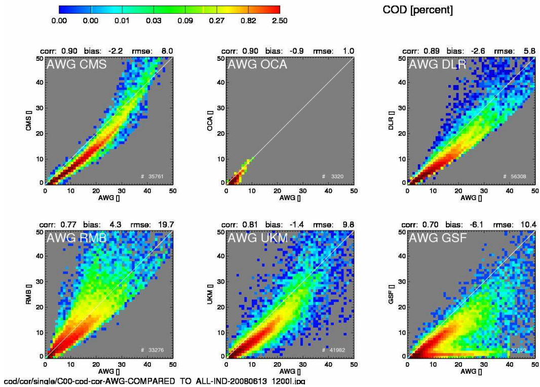
Figure 15 Comparison of DCOMP-COD Ice phase with six other groups.
