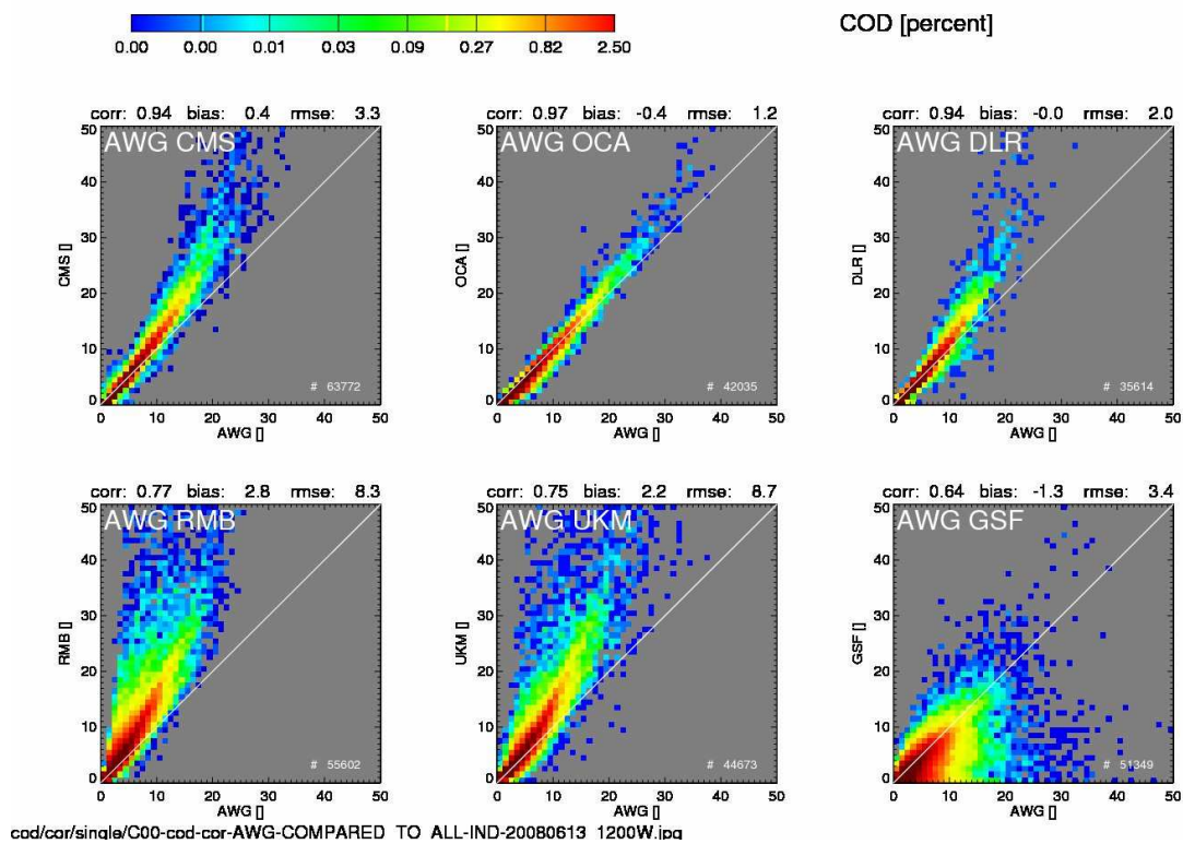
Figure 14 Comparison of DCOMP-COD for liquid water clouds algorithm (AWG) to six other groups.
