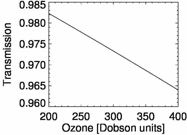
Figure 10 Ozone transmission as a function of absorber amount
