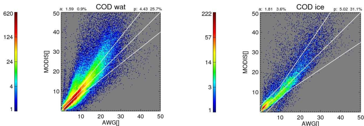
Figure 18 Comparison of Cloud Optical thickness for Days 230-239 in 2006 derived from MODIS (MYD06 and MOD06) products and from DCOMP algorithm. Left image shows results for water phase, right image for ice phase. Accuracy and precision of the comparison are shown in the figures. Specs ranges are added as white lines in the figures.
