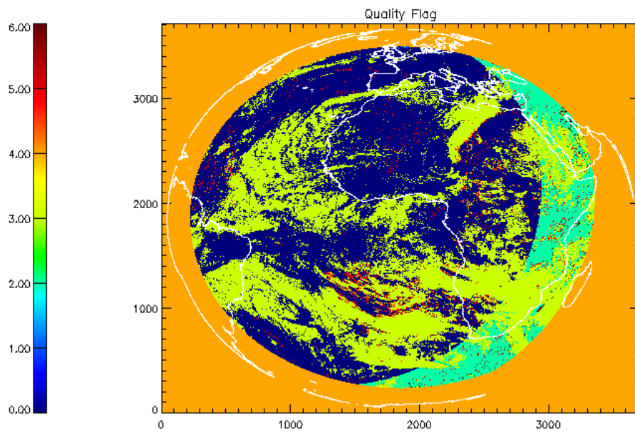
Figure 13 Example for Quality Flag information for SEVIRI scene on day 238 at 12 Z in 2006.
