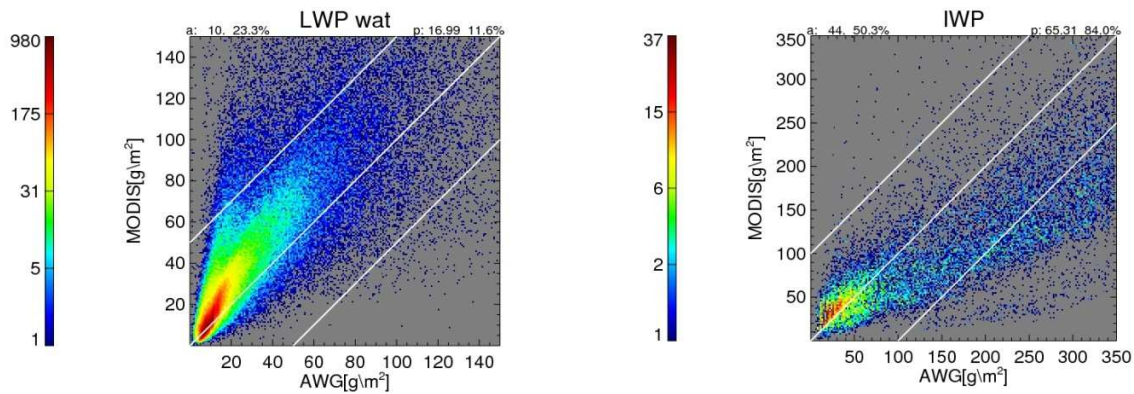
Figure 20 Comparison of Water Path for Days 230-239 in 2006 derived from MODIS (MYD06 and MOD06) products and from DCOMP algorithm. Left image shows results for water phase (LWP), right image for ice phase (IWP). Accuracy and precision of the comparison are shown in the figures. Specs ranges are added as white lines in the figures.
