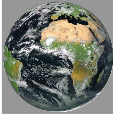
Figure 11 Full disk false color image from SEVIRI 13UTC on 1 August 2006.
