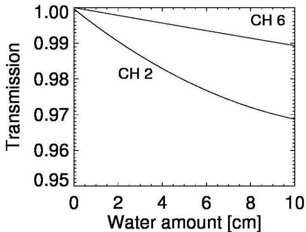
Figure 9 Water vapor transmission as a function of absorber amount.
