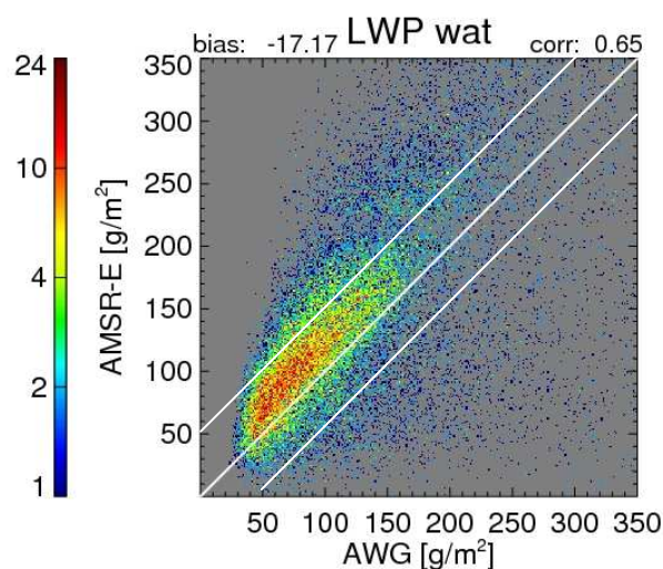
Figure 21 Comparison of AWG-DCOMP Liquid water product to AMSR-E for a two-day period (24-25 August 2006) as a 2D histogram.
