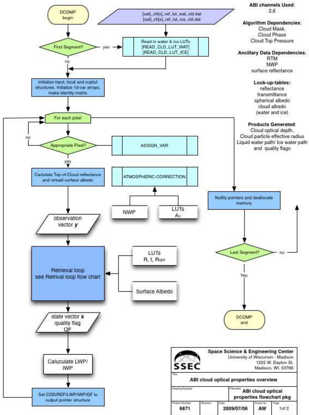
Figure 2 High-level flowchart of the COP/CPS algorithm.
