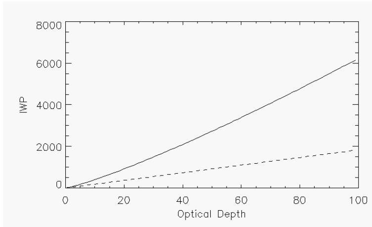
Figure 4 Comparison of Heysmsfield method to a traditional method (dashed line) of calculating the ice water path from optical depth.
