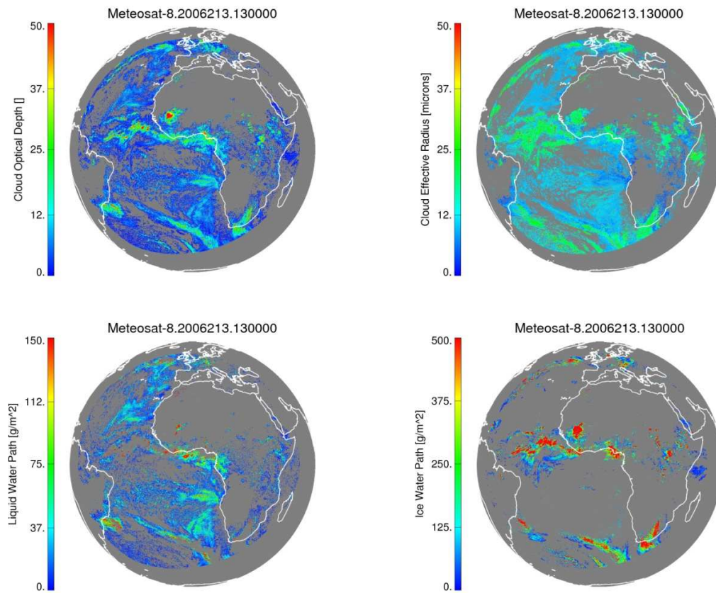
Figure 12 Results of the retrieval for 1 August 2006 13:00UTC for SEVIRI. Upper panel shows optical depth (left) and effective radius (right). Lower panel shows liquid water path (left) and ice water path (right).
