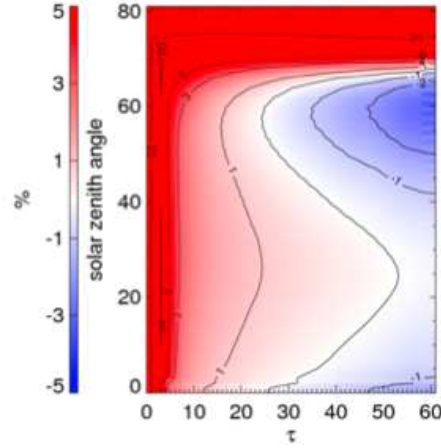
Figure 8 Potential error in percent if Rayleigh correction is not applied as a function of \tau_c and solar zenith angle. Observation angle is 43 degrees and effective radius is 8 \mu m .
