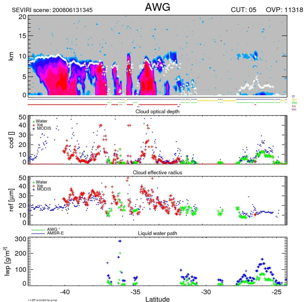
Figure 17 Integrative comparison of ABI products. Upper panel shows CloudSat radar reflectivities with ABI cloud height (white crosses). Second panel shows comparison of DCOMP cloud optical depth of ice (red) and liquid water (green) with MODIS. Third panel shows same, but for effective radius. Bottom panel illustrates comparison of DCOMP liquid water path with AMSR-E.
