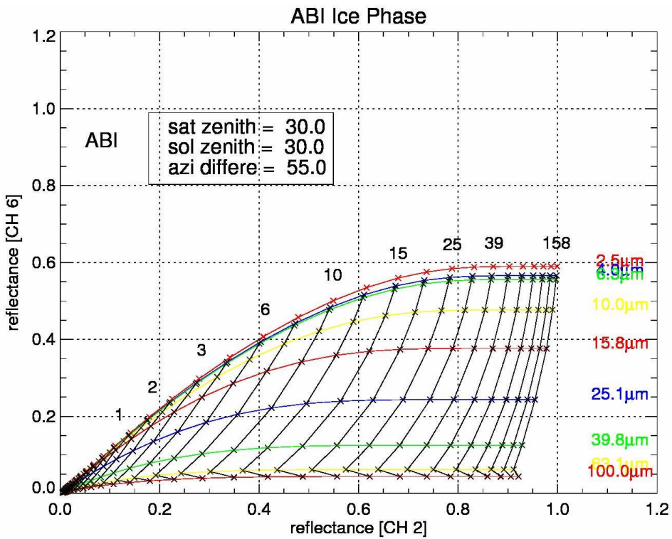
Figure 7 Same as Figure 6 , but for ice clouds.
