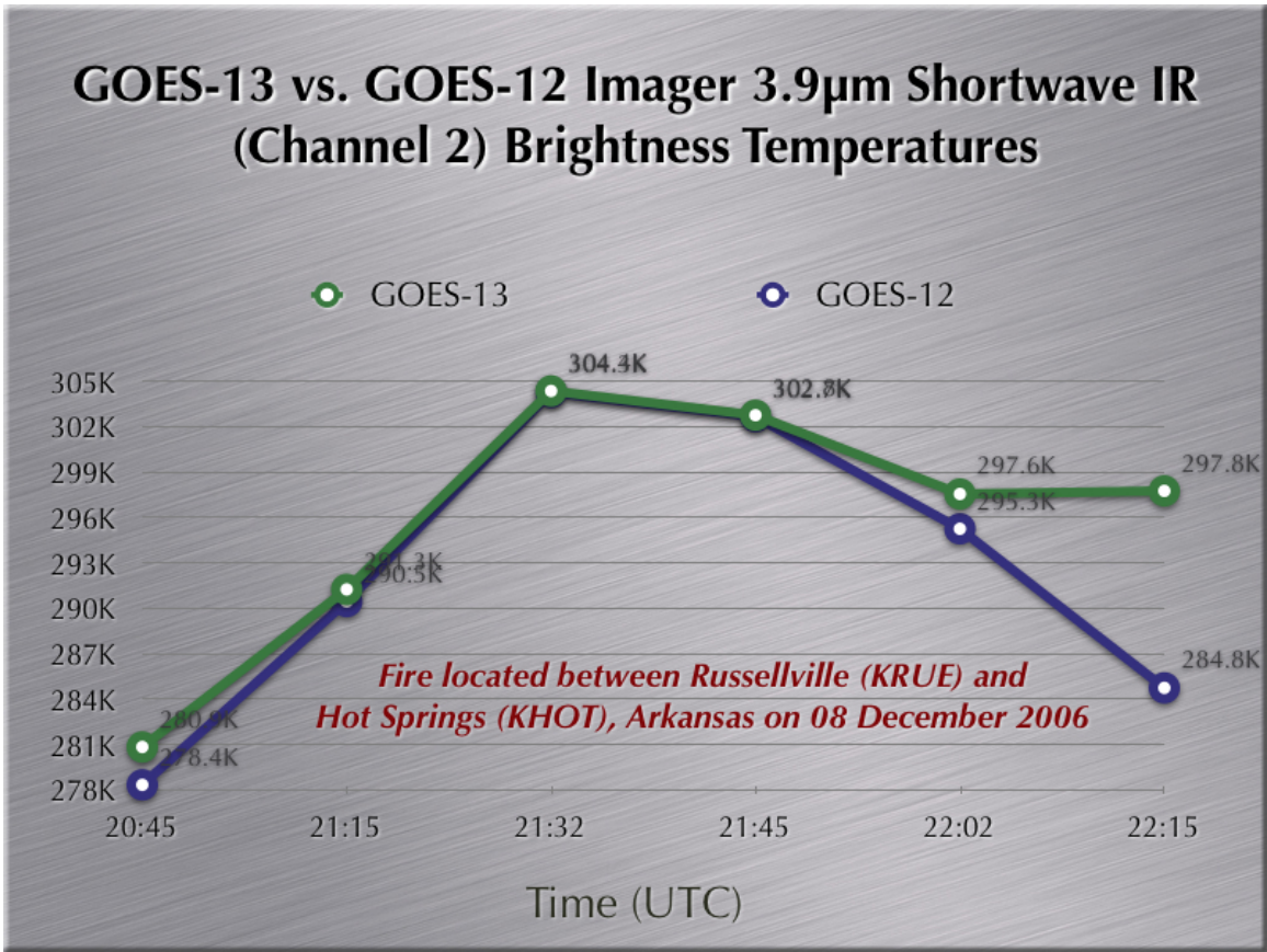
Figure 5.25: GOES Imager 3.9 \mu m time series from GOES-13 and GOES-12.
