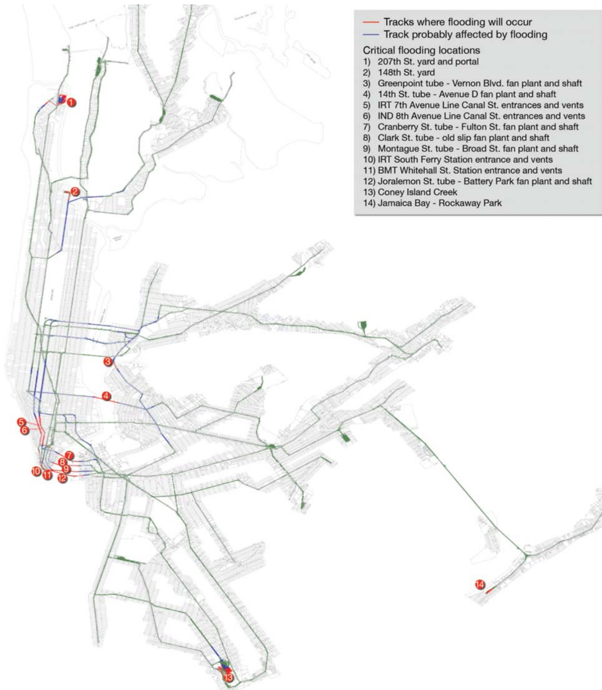
Figure 9.14 MTA subway flooding map for a category-1 hurricane based on surge heights listed in USACE (1995)
