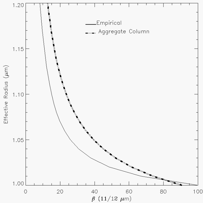
Figure 8 Variation of the 11 and 12 \mu\text{m} \beta values as a function of the ice crystal radius for both the Empirical model and Aggregate Column model. This relation is used in the retrieval to produce an estimate of cloud particle size from the final retrieved \beta values.
