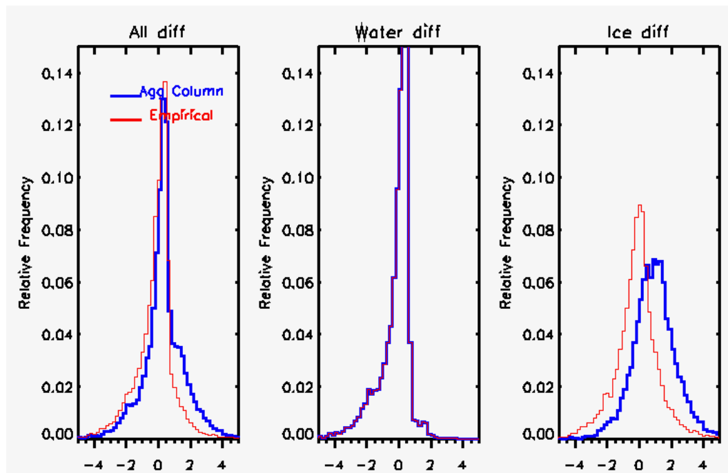
Figure 9 Histogram showing differences between ACHA and CALIPSO cloud top height, using two ice models. One day of MODIS 5km data (06/30/2010) are run at mode 5 to simulate VIIRS output.
