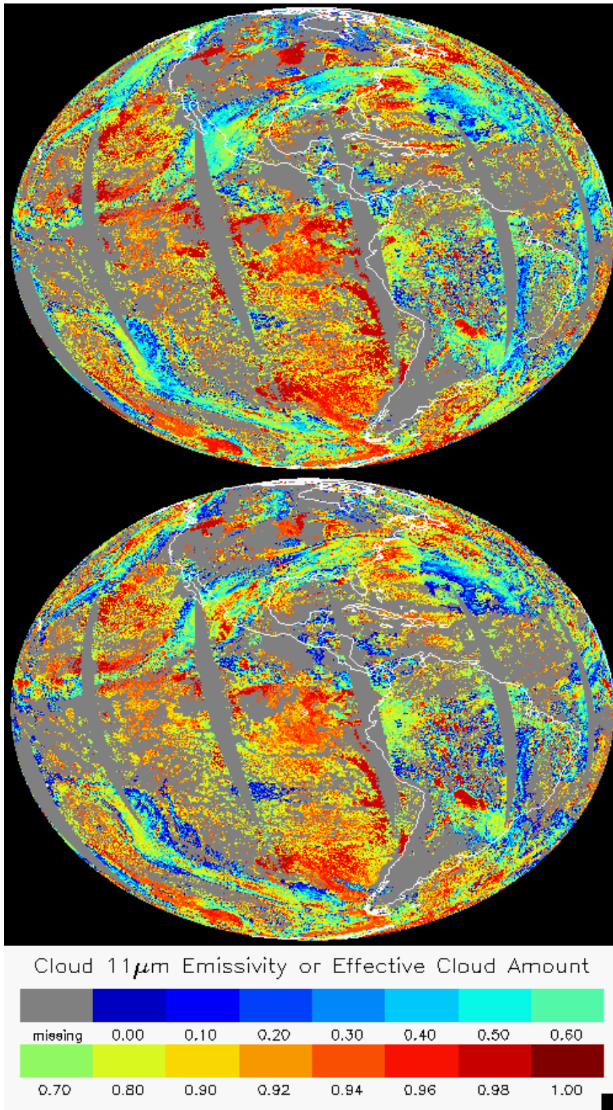
Figure 17 Example ACHA output of 11\mu\text{m} cloud emissivity derived from MODIS proxy data for VIIRS (top) and MODIS (bottom) on January 1, 2013.
