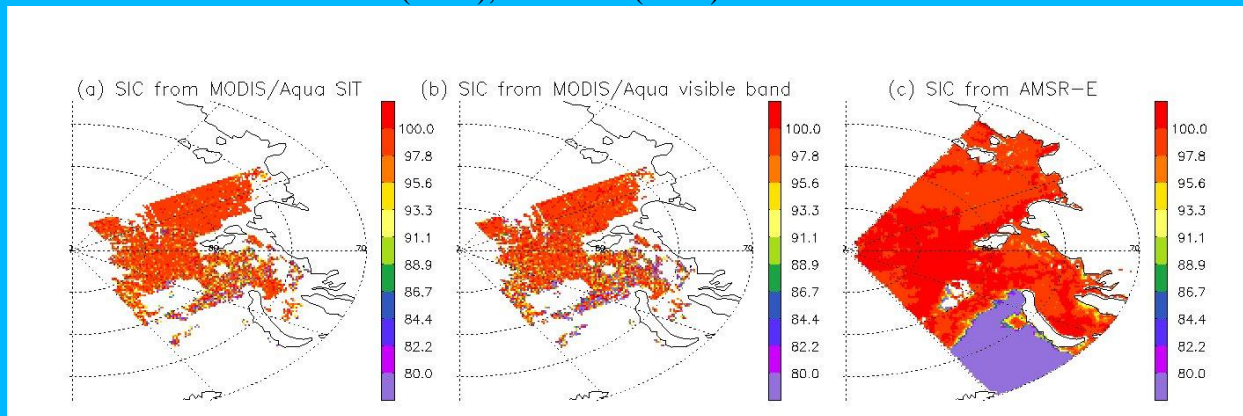
Figure 6. Sea ice concentration (SIC) (%) retrieved from (a) MODIS Sea Ice Temperature (SIT), (b) MODIS visible band reflectance, and (c) from Advanced Microwave Scanning Radiometer - Earth Observing System (AMSR-E) Level-3 gridded daily mean from NSIDC on March 31, 2006.
