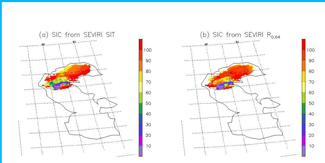
Figure 5. Lake ice concentration (%) retrieved from (a) SEVIRI Surface Ice Temperature (SIT), (b) SEVIRI visible band reflectance ( 0.64\ \mu\text{m} ) on January 27, 2006.
