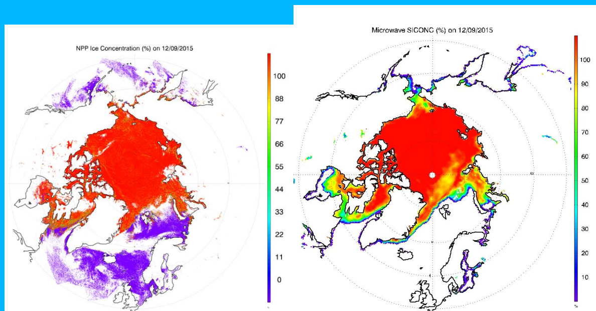
Figure 13. Ice concentration for daily ice concentration composite from VIIRS (left) and from microwave using NASA team algorithm (right) over the Arctic on December 9, 2015.
