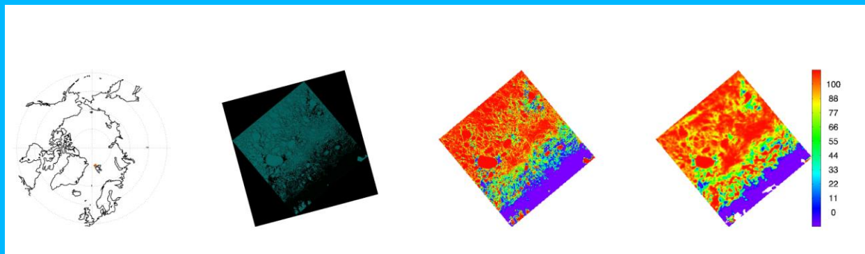
Figure 14. (from left to right) location of the scene shown; true color image of Landsat; Landsat sea ice concentration; and S-NPP VIIRS ice concentration at 12:09 UTC on May 27, 2013.
