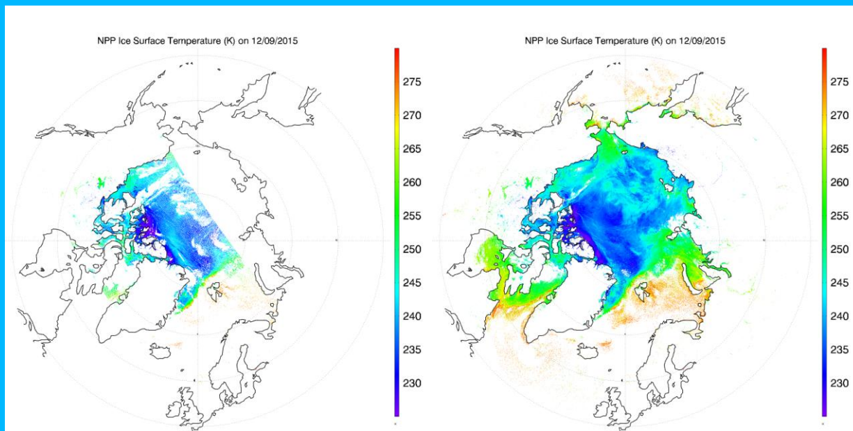
Figure 9. (left) Ice surface temperature (IST) for VIIRS overpass over the Arctic from 10:57 to 11:15 UTC on December 9, 2015; (right) daily IST composite over the Arctic on December 9, 2015.
