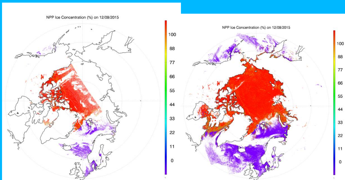
Figure 10. (left) Ice concentration for VIIRS overpass over the Arctic from 10:57 to 11:15 UTC on December 9, 2015; (right) daily ice concentration composite over the Arctic on December 9, 2015.
