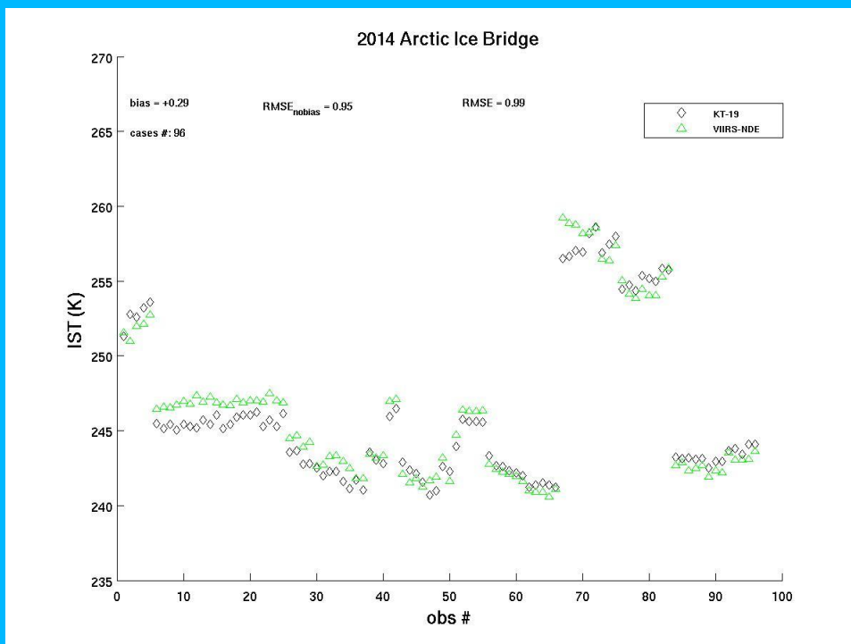
Figure 12. VIIRS IST (green) and KT-19 IST (black) for all coincident IceBridge flights with cloud-free observations over the Arctic (March-May 2014).
