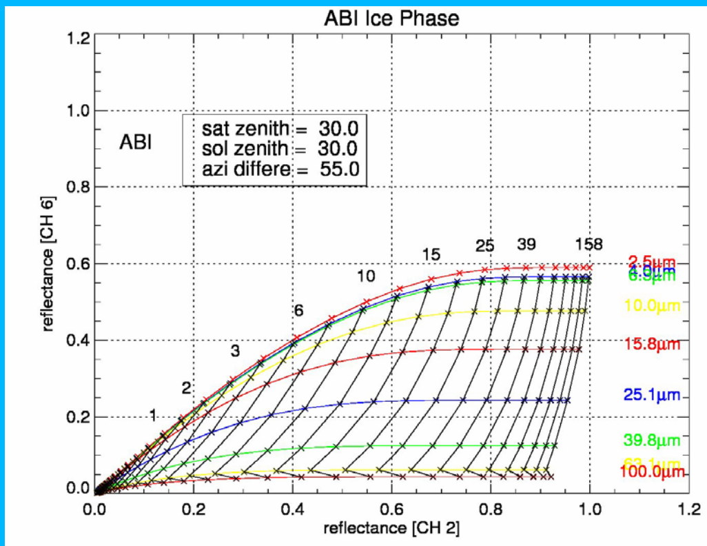
Figure 8 Same as Figure 6, but for ice clouds.
