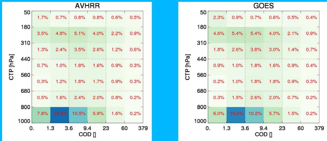
Figure 18 Comparison of level2b data from the AVHRR PATMOS-x data set ( left) and a similar level-2b data set derived by GOES-EAST satellite
