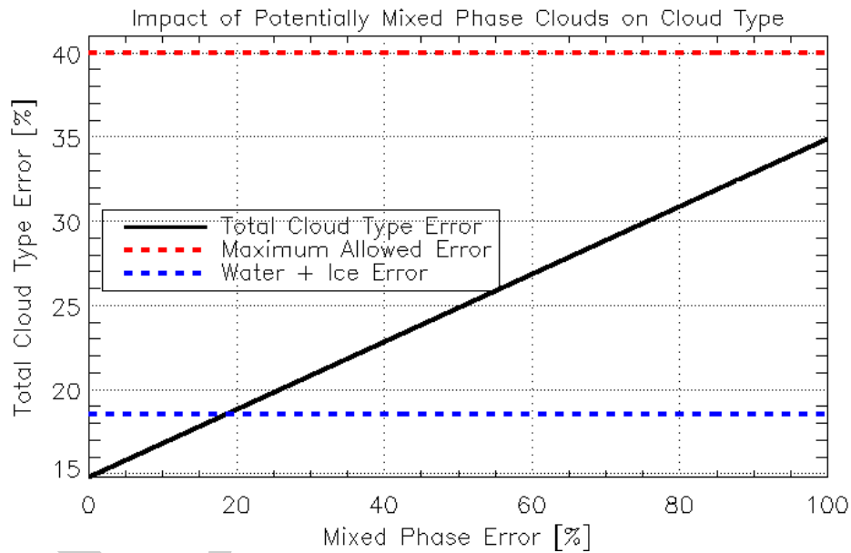
Figure 20: Same as Figure 19, except for cloud type.
