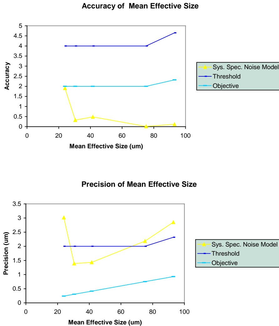
Figure 42. Accuracy (top) and Precision (bottom) of Retrieved Effective Particle Size from the Cirrus Solar Algorithm for US Standard Atmosphere based on the 0.672-2.25µm Correlation, Sensor at Nadir.
