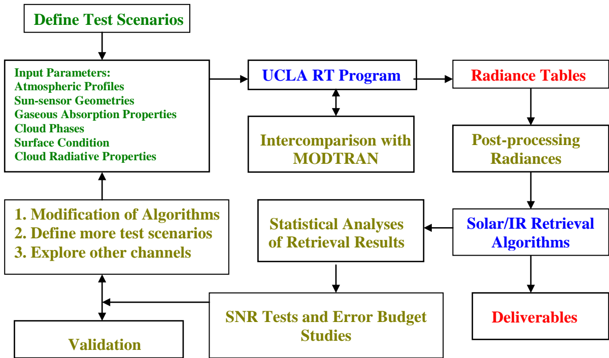
Figure 3. A High-Level Flow Diagram depicting the Processing Outline of the Data Flow of the VIIRS Channel Radiance in the Development of VIIRS Cloud EDR Retrieval Algorithms.
