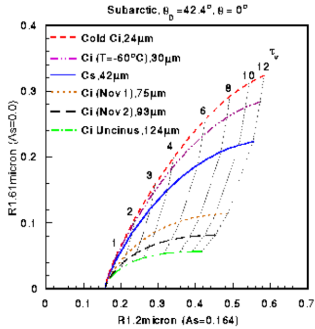
Figure 30. Display of the 1.2-1.61 \mu m Reflectance Correlations for Cirrus Cloud in Sub-Arctic Atmosphere, Sensor at Nadir.
