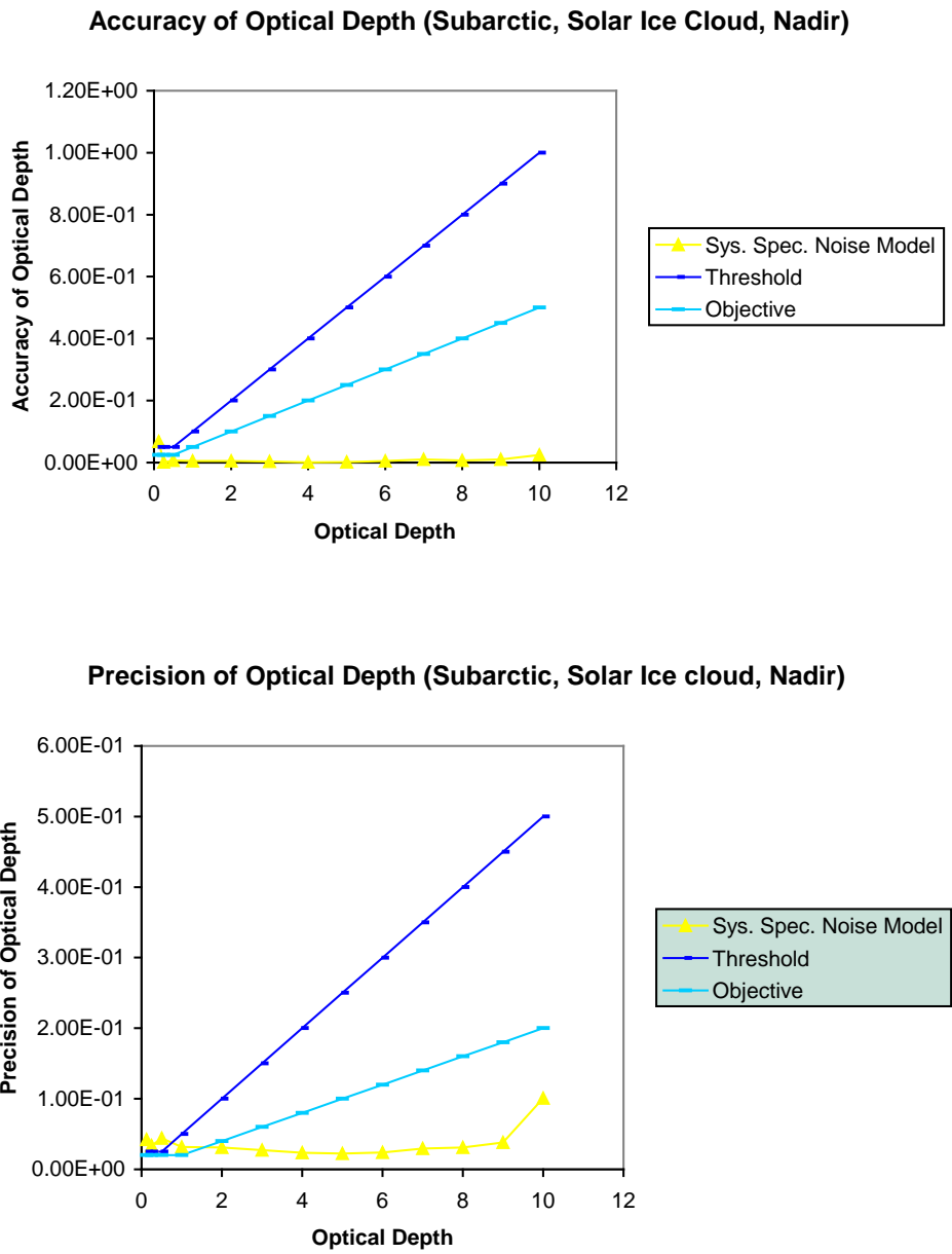
Figure 31. Accuracy (top) and Precision (bottom) of Retrieved Optical Depths from the Solar Algorithm for Cirrus Cloud in Sub-Arctic Atmosphere, Sensor at Nadir.
