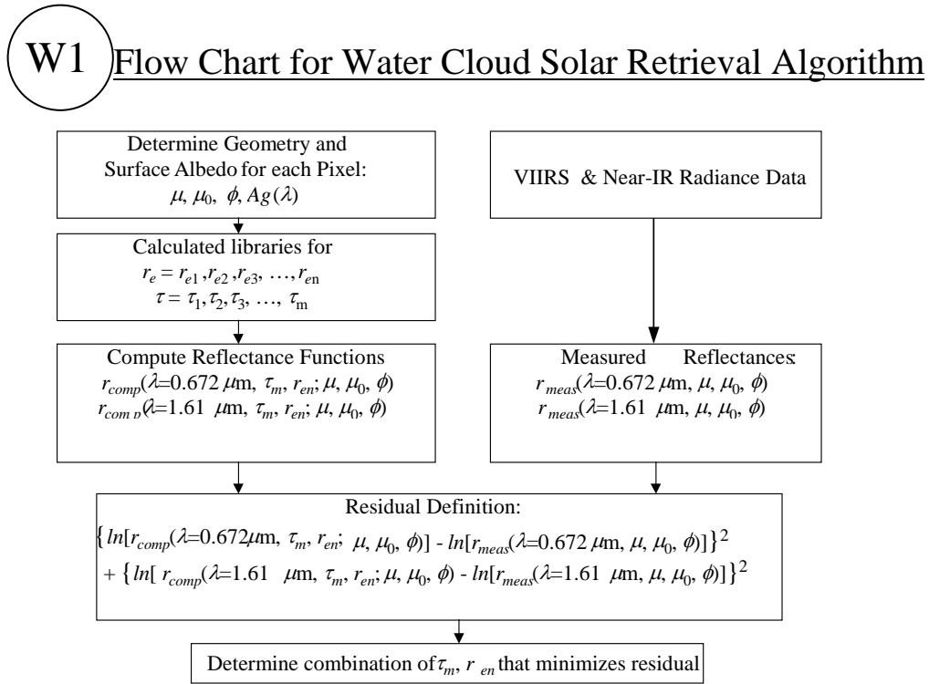
Figure 19. Flow Chart for the Solar Water Cloud Retrieval Algorithm.
