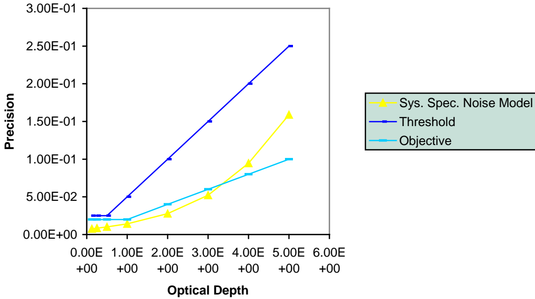
Figure 37. Accuracy (top) and Precision (bottom) of Retrieved Optical Depths from the IR Algorithm for Cirrus Cloud in US Standard Atmosphere, Sensor pointing Off-Nadir.
