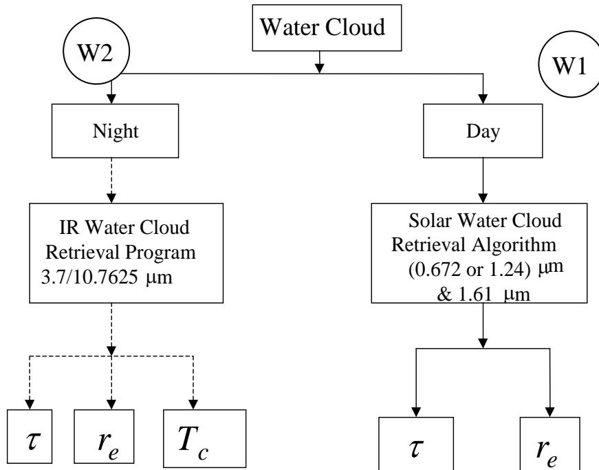
Figure 18. Flow Chart for the Water Cloud Retrieval Program.
