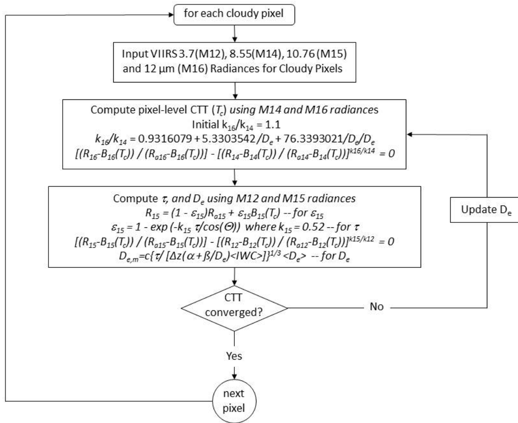
Figure 14. Flow Chart for the Nighttime IR Cirrus Retrieval Algorithm.
