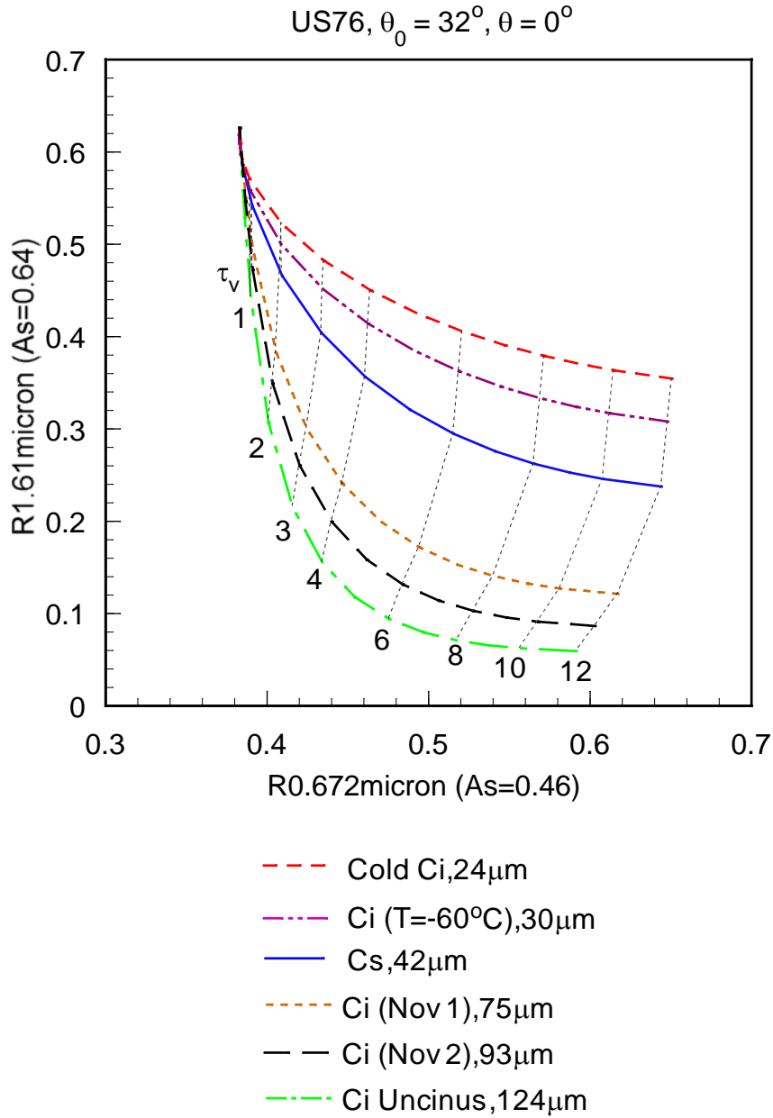
Figure 32. Display of the 0.672-1.61 \mu\text{m} Reflectance Correlations for Cirrus Cloud in Desert Atmosphere, Sensor at Nadir.
