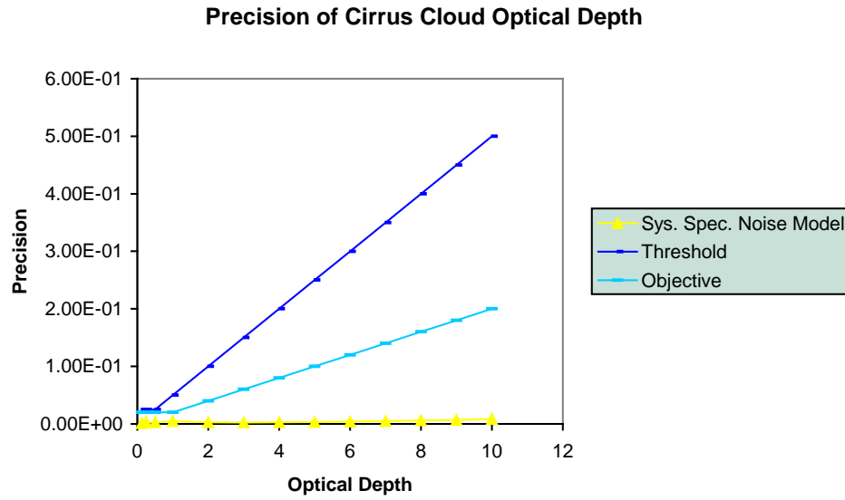
Figure 23. Accuracy (top) and Precision (bottom) of Retrieved Optical Depths from the Cirrus Solar Algorithm for US Standard Atmosphere based on the 0.672–2.25 \mu\text{m} Correlation, Sensor at Nadir.
