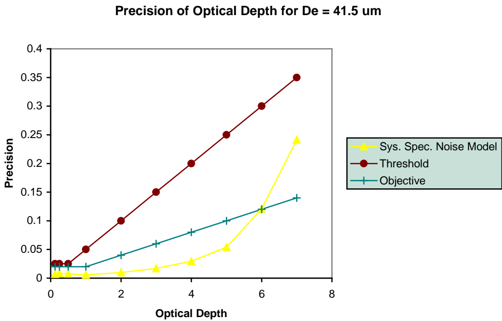
Figure 36. Accuracy (top) and Precision (bottom) of Retrieved Optical Depths from the IR Algorithm for Cirrus Cloud in US Standard Atmosphere, Sensor at Nadir.
