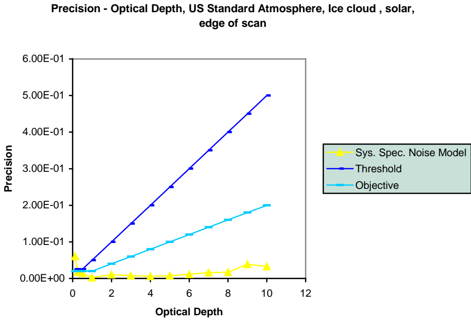
Figure 27. Accuracy (top) and Precision (bottom) of Retrieved Optical Depths from the Solar Algorithm for Cirrus Cloud in US Standard Atmosphere, Sensor at Edge-of-Scan.
