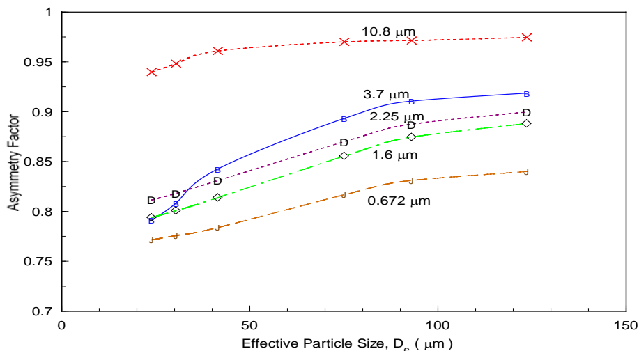
Figure 6b. Asymmetry factors for the six size distributions and for the five VIIRS cloud retrieval channels.
