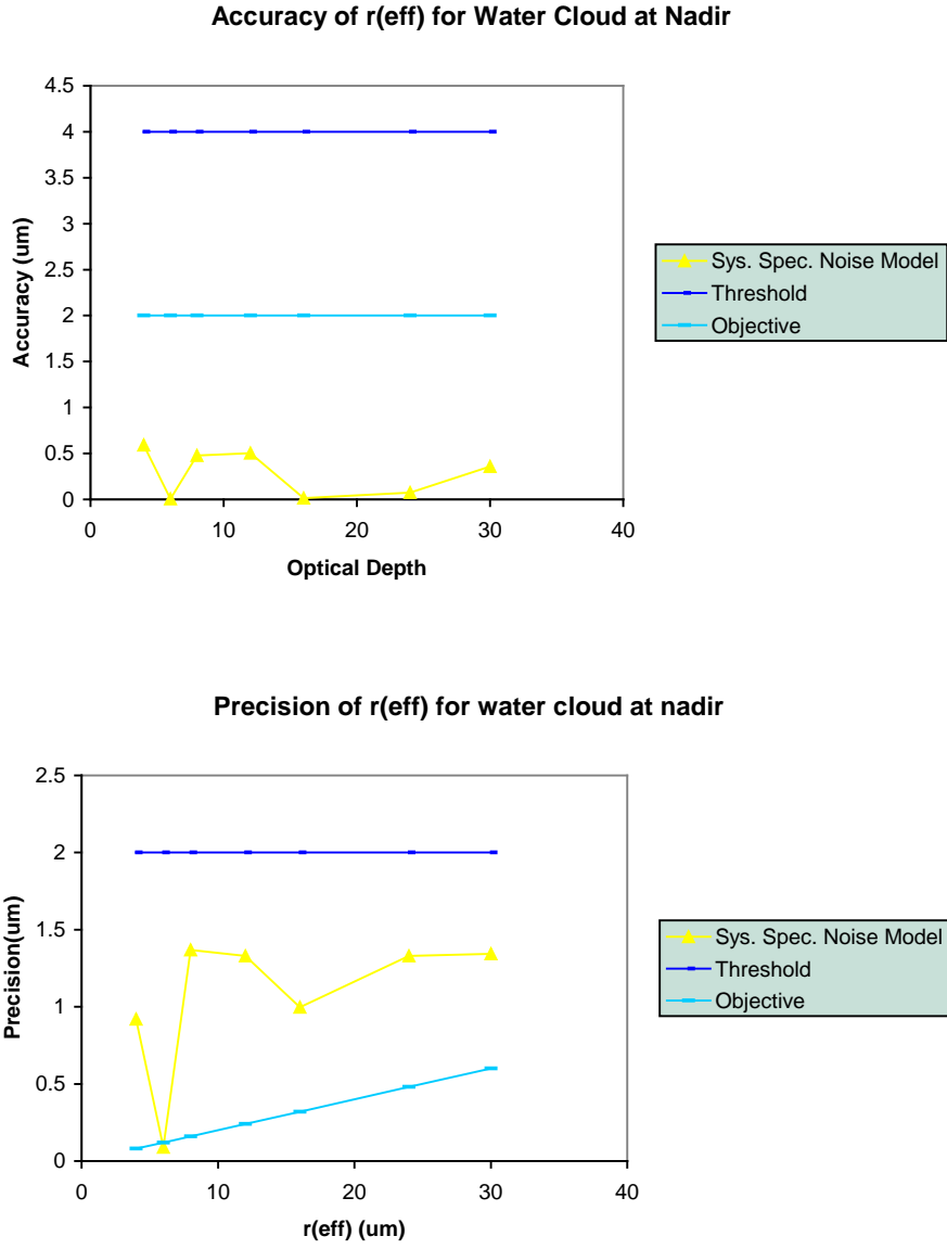
Figure 48. Accuracy (top) and Precision (bottom) of Retrieved Effective Particle Size from the Water Cloud Solar Algorithm for US Standard Atmosphere based on the 0.672-1.61µm Correlation, Sensor at Nadir.
