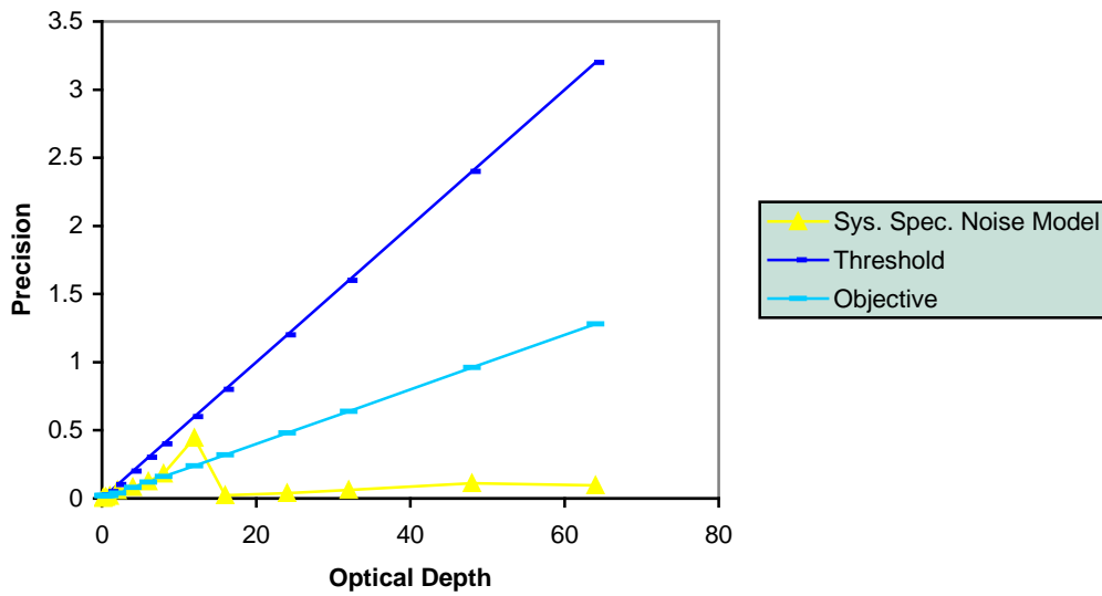
Figure 35. Accuracy (top) and Precision (bottom) of Retrieved Optical Depths from the Solar Algorithm for Water Cloud in US Standard Atmosphere, Sensor at Nadir.
