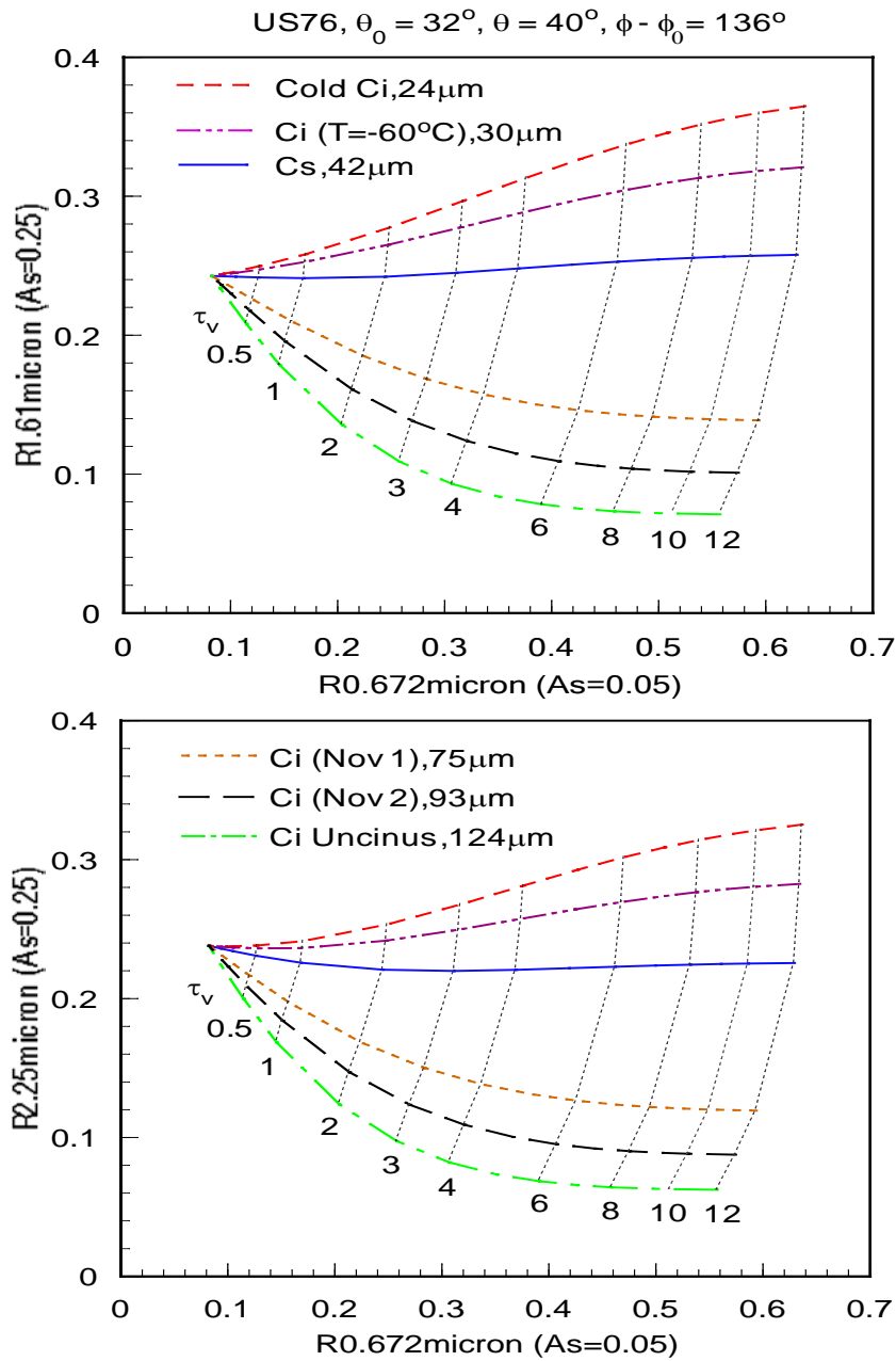
Figure 24. Display of the 0.672-1.61µm (top) and 0.672-2.25µm (bottom) Reflectance Correlations for Cirrus Cloud in US Standard Atmosphere, Sensor pointing Off-Nadir.
