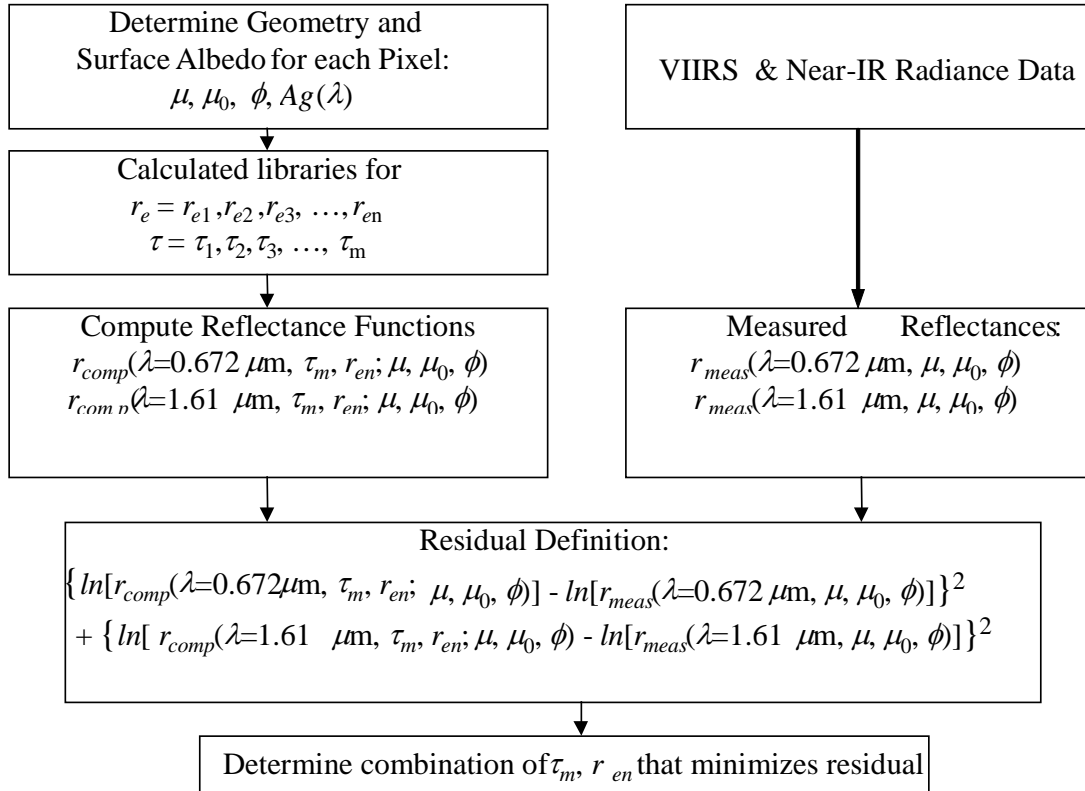
Figure 16. Flow Chart for the solar Cirrus Retrieval Algorithm
