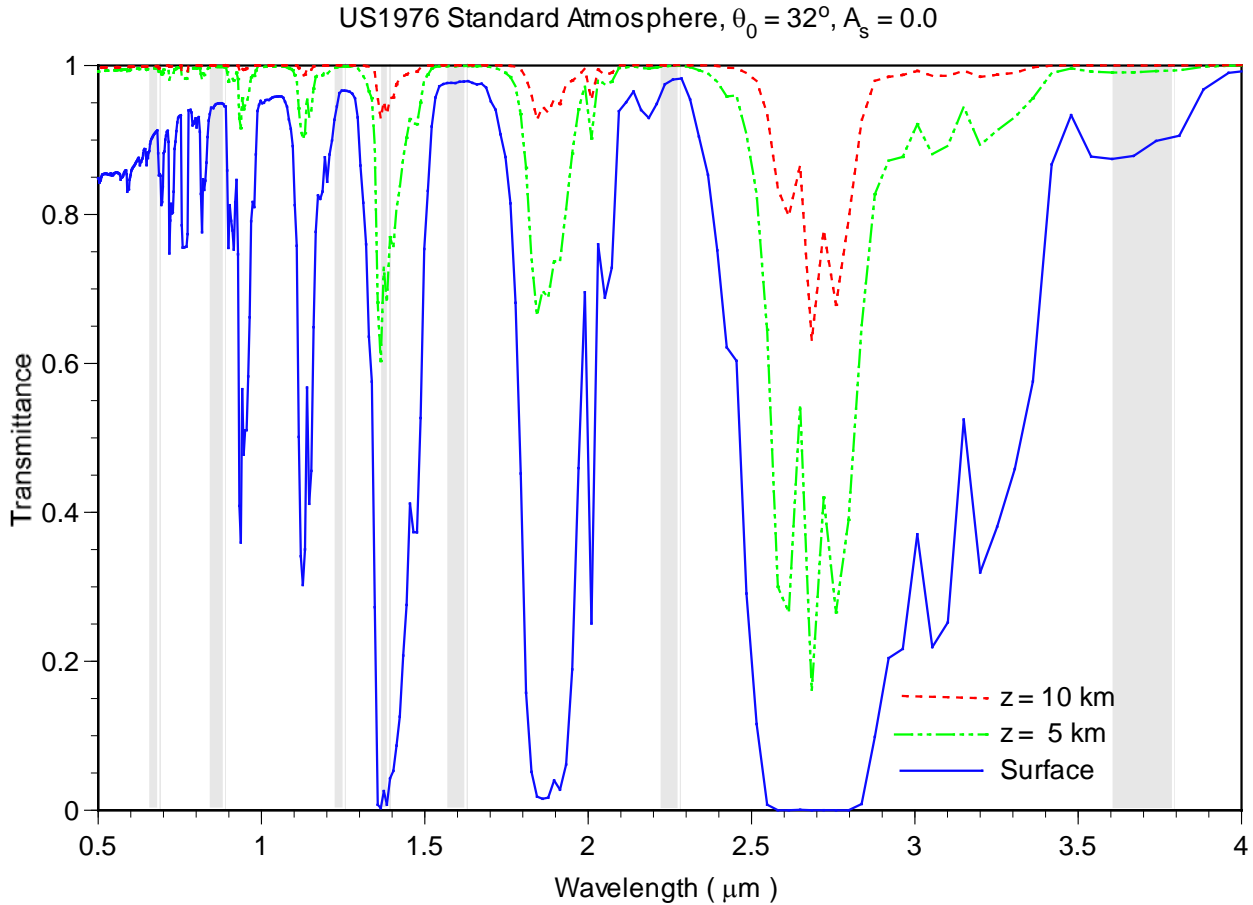
Figure 1. Transmittance Characteristics of Seven VIIRS Solar Channels centered at 0.672, 0.865, 1.24, 1.378, 1.61, 2.25 and 3.7 \mu\text{m} . The atmospheric zenith transmittances are calculated from the LBLE model for three levels at 10 km, 5 km and the surface based on the US Standard Atmosphere at a 32 ^\circ solar zenith angle.
