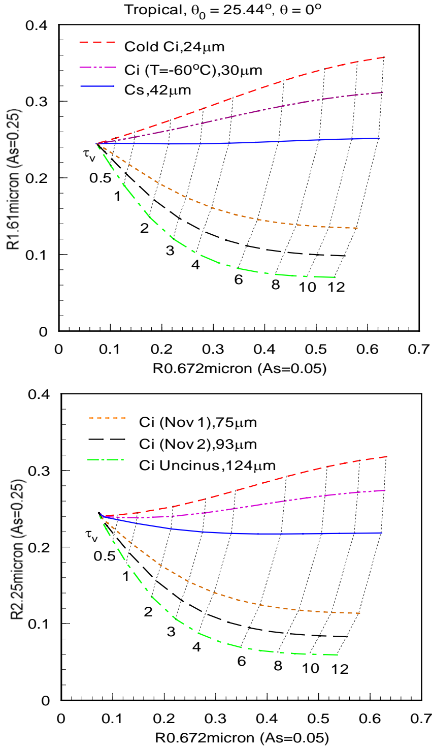
Figure 28. Display of the 0.672-1.61µm (top) and 0.672-2.25µm (bottom) Reflectance Correlations for Cirrus Cloud in Tropical Atmosphere, Sensor at Nadir.
