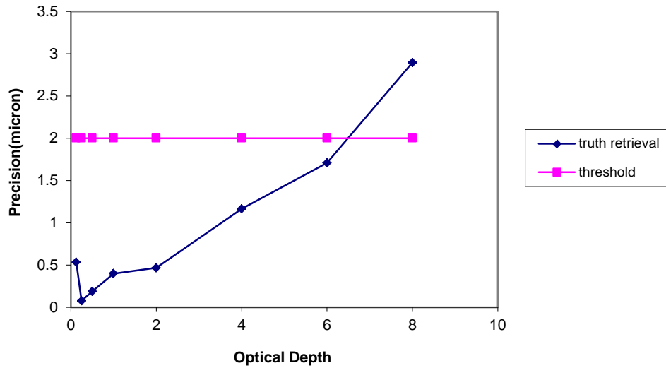
Figure 57. Accuracy (top) and Precision (bottom) of Retrieved Effective Particle Size from the IR Algorithm for Water Cloud, US Standard Atmosphere, No-Noise Retrievals, Sensor at Nadir.
