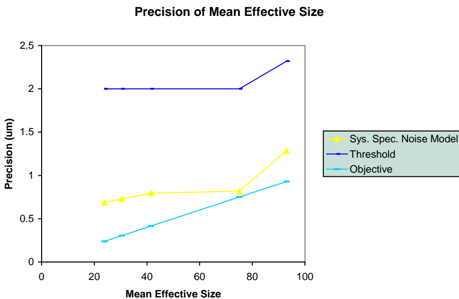
Figure 41. Accuracy (top) and Precision (bottom) of Retrieved Effective Particle Size from the Cirrus Solar Algorithm for US Standard Atmosphere based on the 0.672-1.61µm Correlation, Sensor at Nadir.
