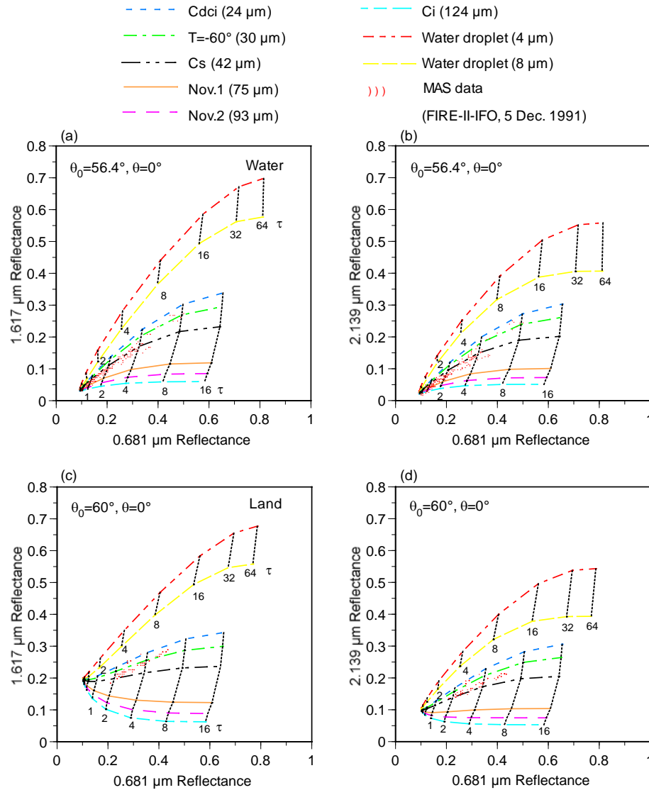
Figure 15. Display of the Correlation of MAS 0.681-1.617 \mu\text{m} Reflectances Based on Radiative Transfer Calculations and MAS Data taken from FIRE-II IFO over Both Land and Water Surfaces. The calculations were performed for the six ice crystal size distributions presented in section 3.3.1.1 and for two water clouds with mean effective radii of 4 and 8 \mu\text{m} . The optical depth ( \tau ) ranges from 0.5 to 64 for water cloud and 0.5-16 for
