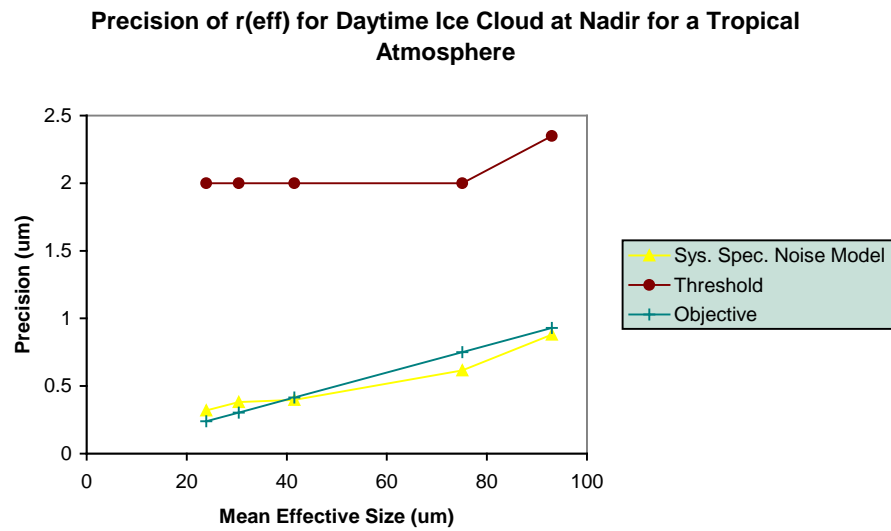
Figure 45. Accuracy (top) and Precision (bottom) of Retrieved Effective Particle Size from the Cirrus Solar Algorithm for Tropical Atmosphere based on the 0.672-1.61 \mu\text{m} Correlation, Sensor at Nadir.
