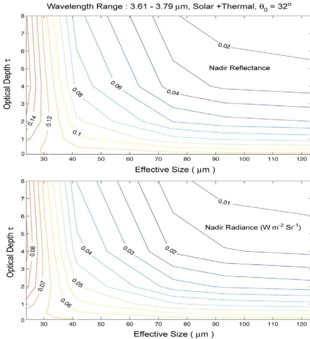
Figure 10. Contour Plot of the 3.7 \mu\text{m} Total (Solar + Thermal) Reflectance (above) and Radiance (below) for the Same Combinations of Cirrus Cloud Optical Depths and Mean Effective Sizes for High-Sun Angle ( \theta_0=32^\circ ) and Nadir Viewing.
