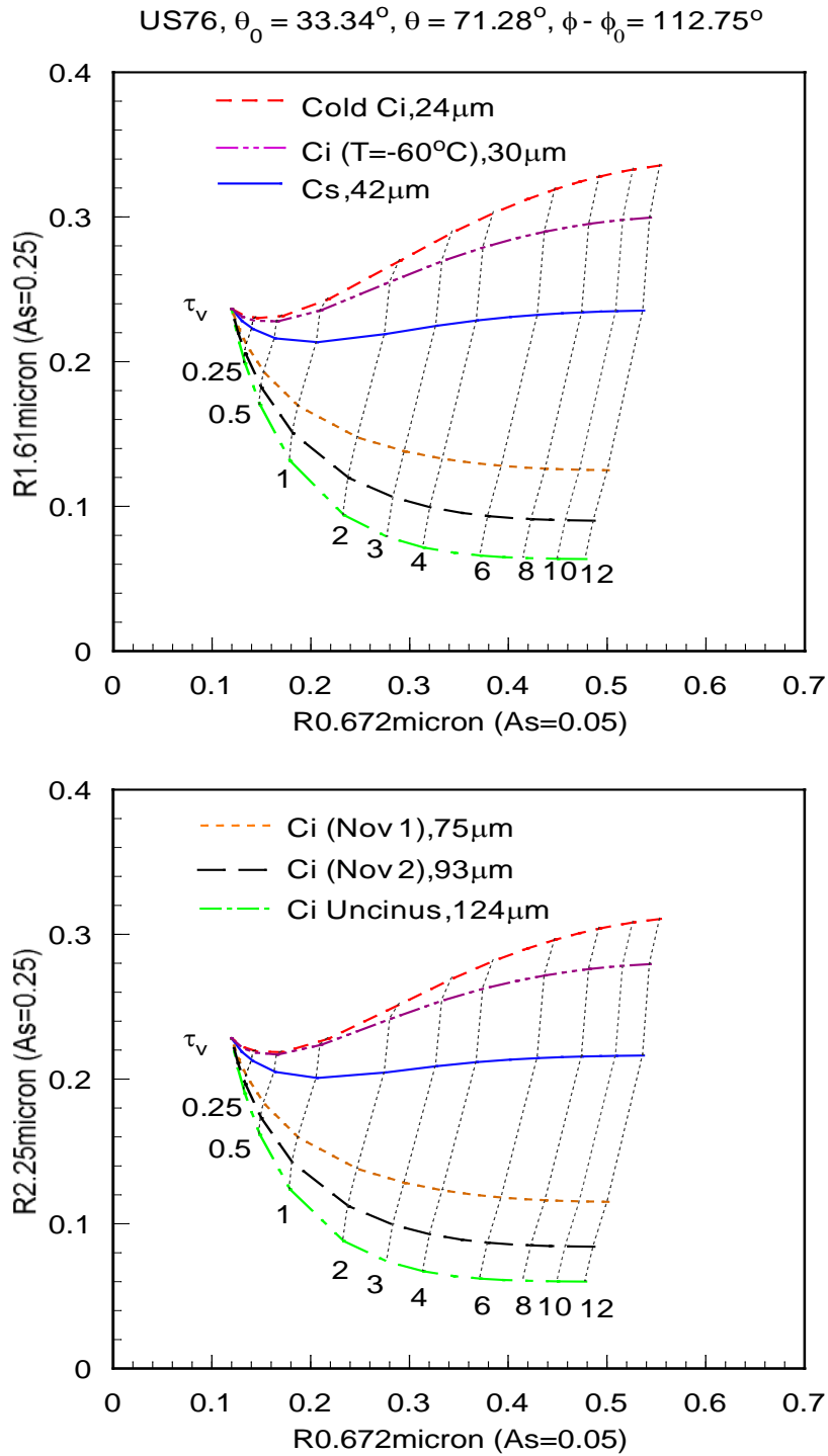
Figure 26. Display of the 0.672-1.61µm (top) and 0.672-2.25µm (bottom) Reflectance Correlations for Cirrus Cloud in US Standard Atmosphere, Sensor at Edge-of-Scan.
