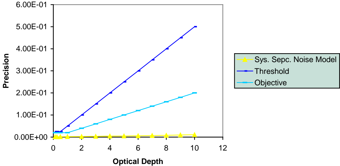
Figure 22. Accuracy (top) and Precision (bottom) of Retrieved Optical Depths from the Cirrus Solar Algorithm for US Standard Atmosphere based on the 0.672–1.61µm Correlation, Sensor at Nadir.
