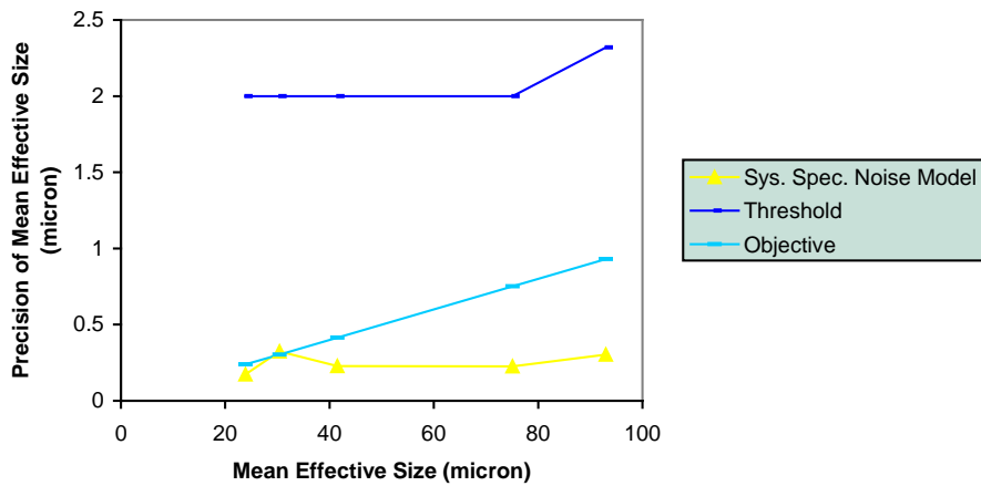
Figure 46. Accuracy (top) and Precision (bottom) of Retrieved Effective Particle Size from the Cirrus Solar Algorithm for Sub-Arctic Atmosphere based on the 1.2-1.61µm Correlation, Sensor at Nadir.
