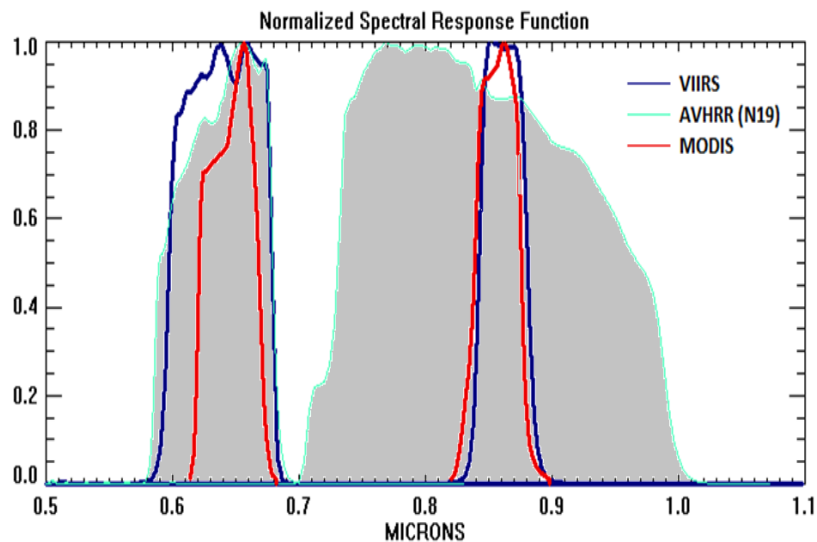
Figure 3-9 Normalized spectral response functions of VIS and NIR bands
