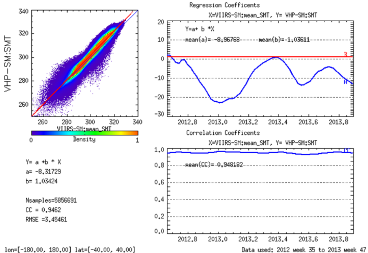
Figure 3-14 Relationship between VIIRS/BT and AVHRR/BT.
