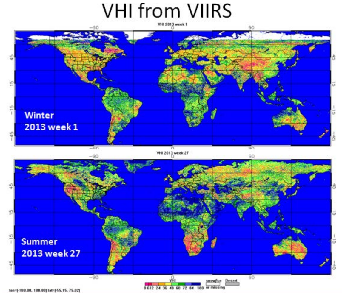
Figure 3-17 Vegetation Health maps produced by the VIIRS-VH algorithm
