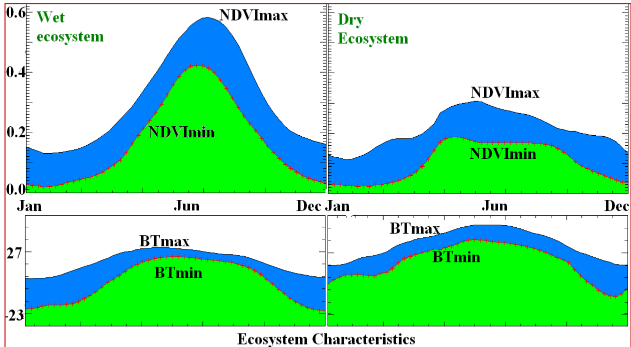
Figure 3-4 NDVI & BT Carrying Capacity Central USA
