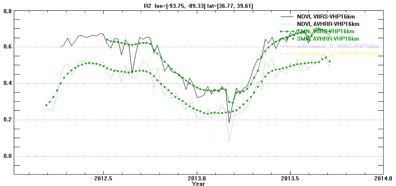
Figure 3-8 NDVI and smoothed NDVI derived from AVHRR and VIIRS
