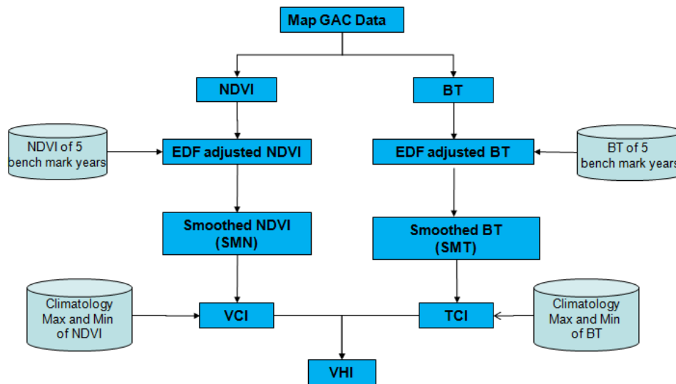
Figure 3-1 Data flow chart of AVHRR-VH
