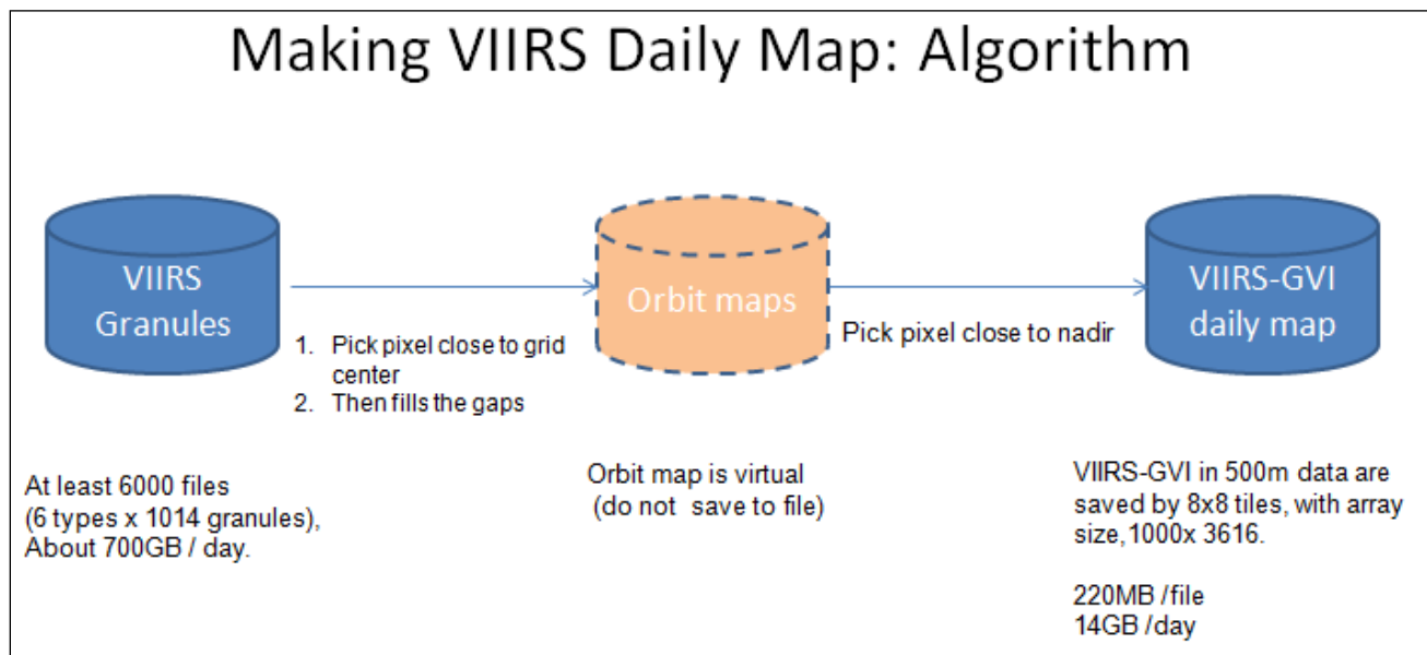
Figure 3-6 Concept of the algorithm of making VIIRS daily map.
