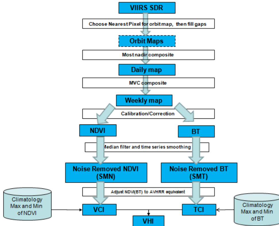
Figure 3-2 Data Flow chart for VIIRS VH
