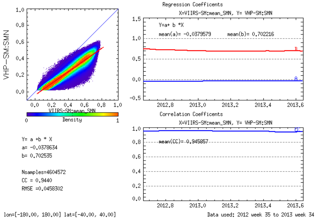
Figure 3-11 Relationship between VIIRS/NDVI and AVHRR/NDVI
