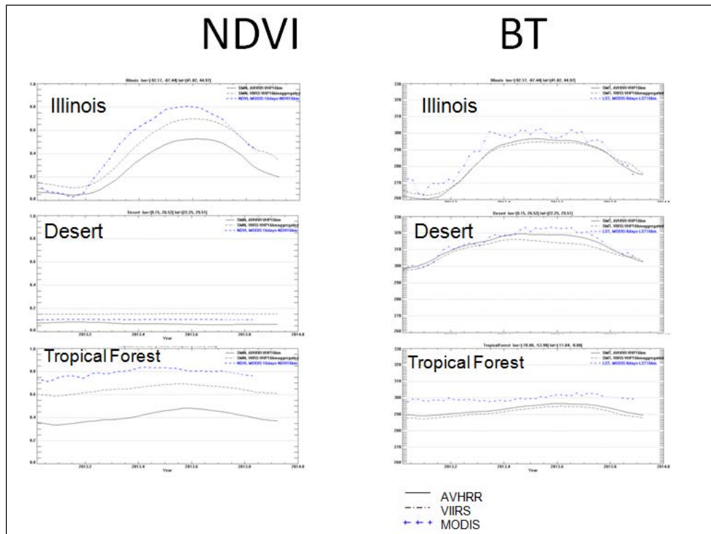
Figure 3-10 Time Series of NDVI and BT derived from AVHRR, VIIRS and MODIS (Before Adjustment).
