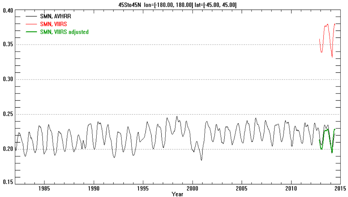
Figure 3-12 Time series of VIIRS/NDVI and AVHRR/NDVI Red line: VIIRS NDVI without adjustment Green line, VIIRS NDVI after adjustment Black line: AVHRR NDVI
