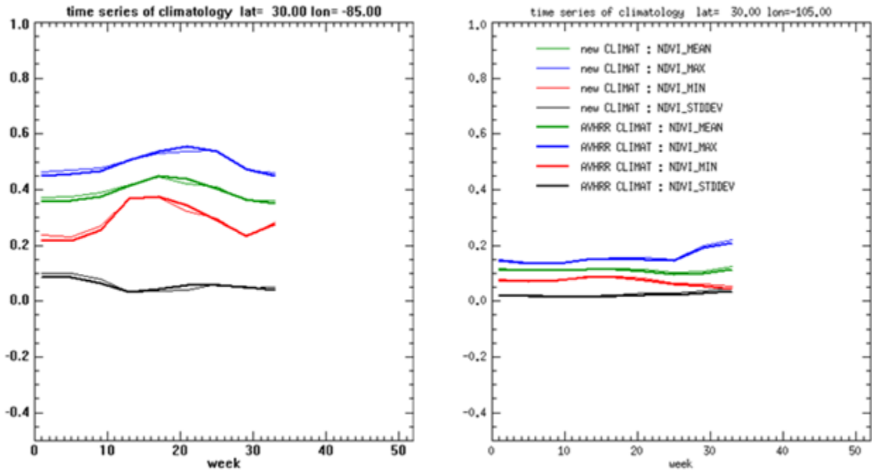
Figure 3-16 New and AVHRR-based NDVI climatology
