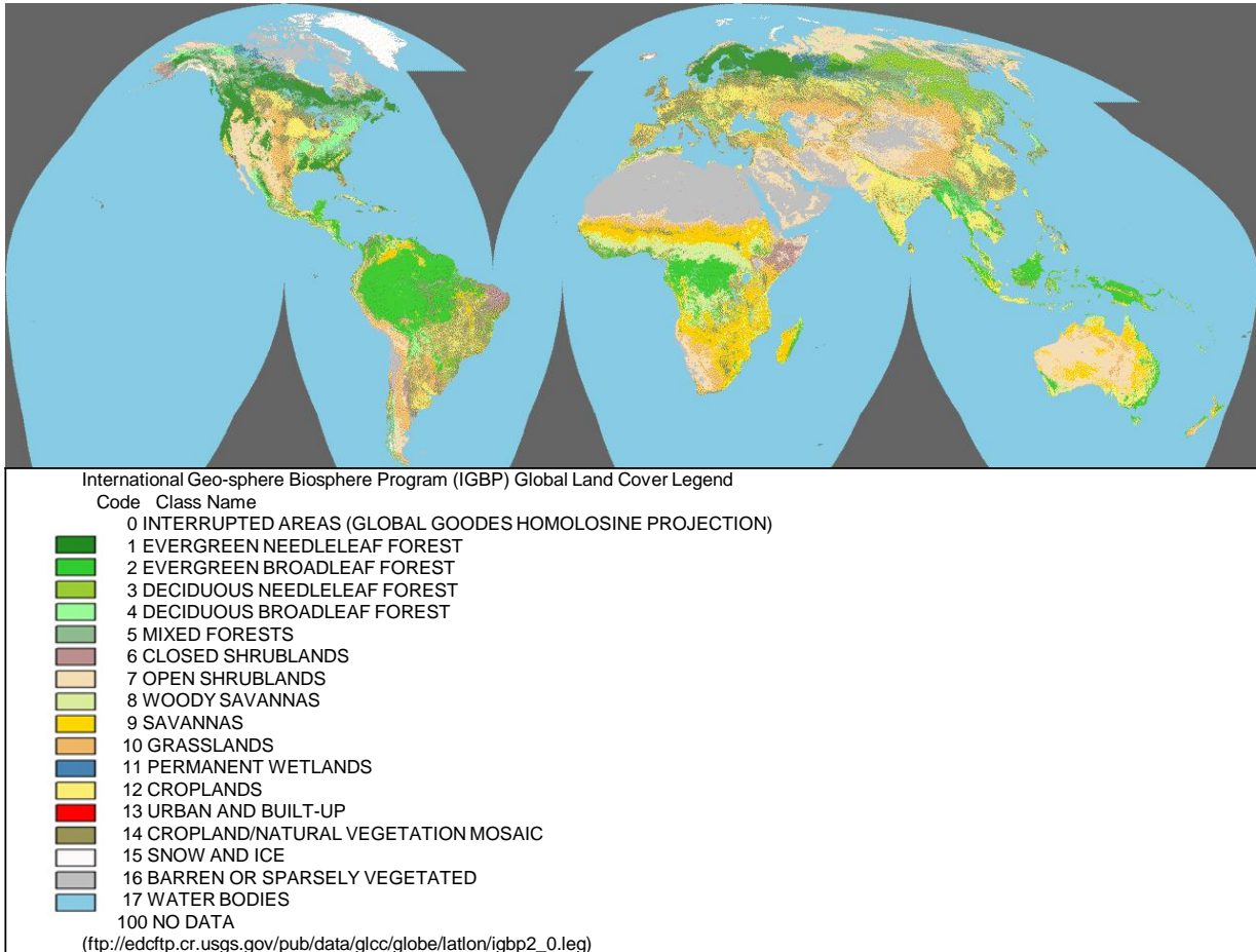
Figure 3-3 IGBP Land Cover Map
