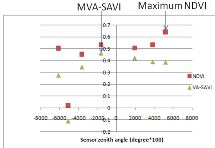
Figure 7. Comparison of the maximum value compositing and the maximum view angle adjusted SAVI compositing.
