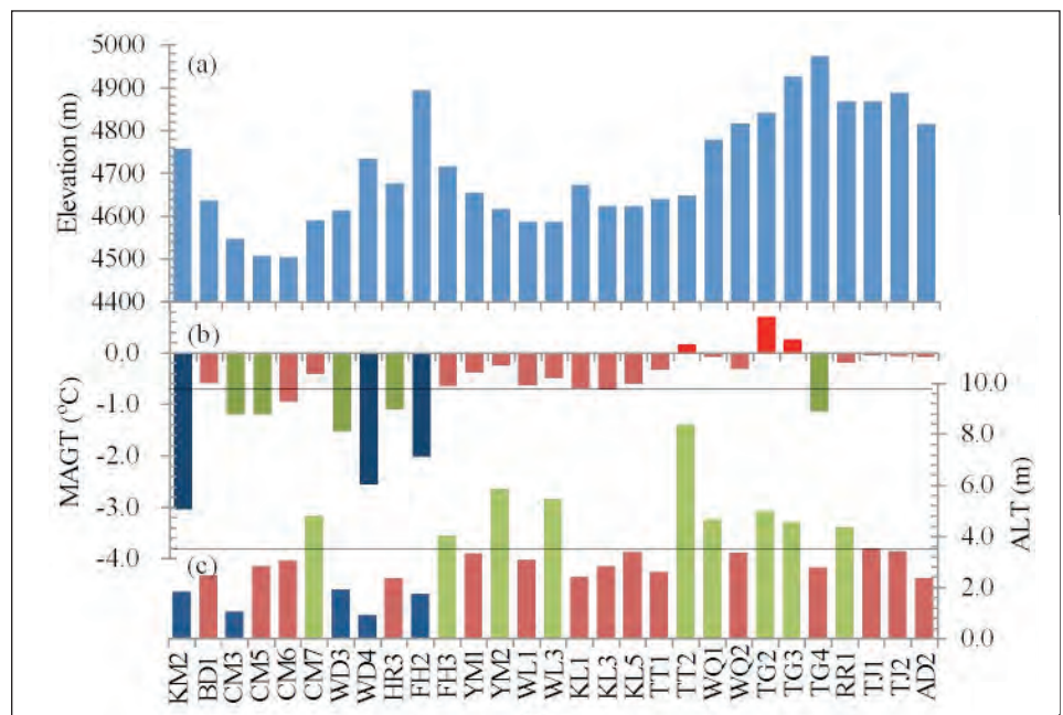
Figure 1: (a) Site elevation; (b) mean annual ground temperature (MAGT) at depth of zero amplitude; and (c) active layer thickness (ALT) along the Qinghai-Xizang (Tibet) Railroad.
