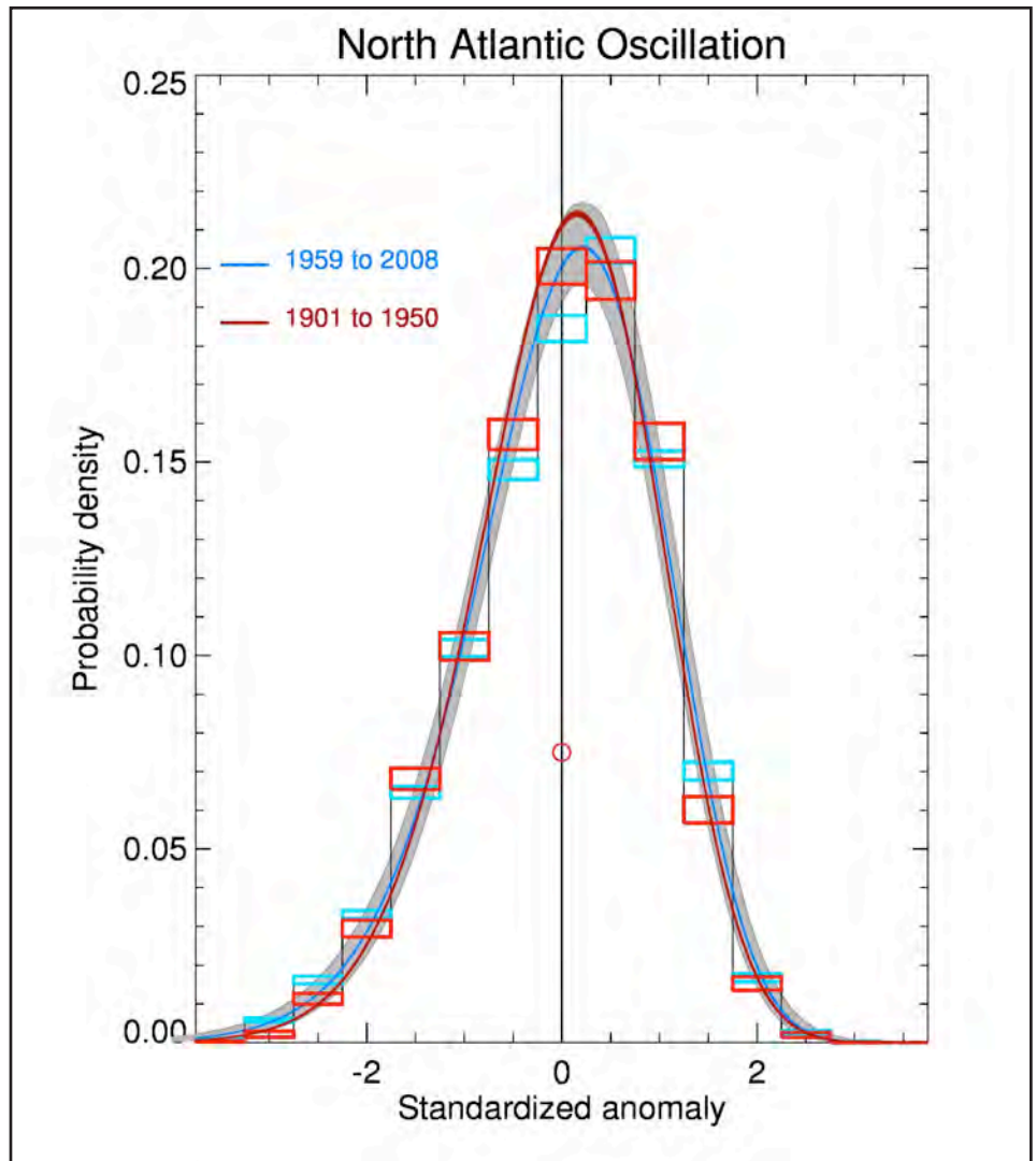
Probability Density Functions (PDFs) of standardized daily anomalies of the North Atlantic Oscillation (NAO) index in northern winter, based on the sea level pressure difference between Azores and Iceland. The PDFs are estimated for two 50-year periods, 1901 to 1950 (red) and 1959 to 2008 (blue), both as raw histograms (rectangles) and continuous PDFs (curves) belonging to a class of skewed and heavy-tailed PDFs identified by Sardeshmukh and Sura ( J. Climate , 2009) as being especially relevant in the atmosphere. The results are derived using each one of the 56 members of the 20th Century Reanalysis ensemble (Compo et al, 2011) as a possible realization of the atmosphere within observational error bounds. There are actually 56 red and 56 blue curves in the plot, obtained from each of these 56 possible realizations, and the red and blue rectangles actually show the range of counts obtained in each anomaly size bin. The gray swath indicates 95% confidence intervals on the PDFs associated with estimating them from limited 50-year records. Thus, the spread among the red and blue curves and boxes indicates observational uncertainty, whereas the gray swath indicates sampling uncertainty. The figure shows there is not only no difference in the mean of the NAO index in the first and second periods (indicated by the completely overlapping red and blue circles at the center of the plot), but also that there is no statistically significant difference in the entire PDF.
