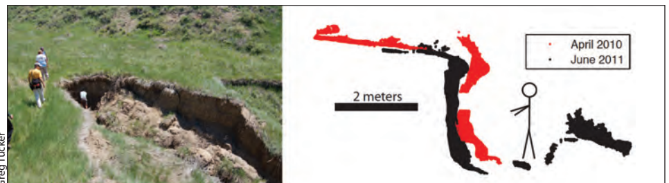
Left: A typical gully head near the West Bijou Escarpment. Right: Cross-sections of the gully head obtained with a ground-based laser scanner, showing morphologic change over a 14-month period
