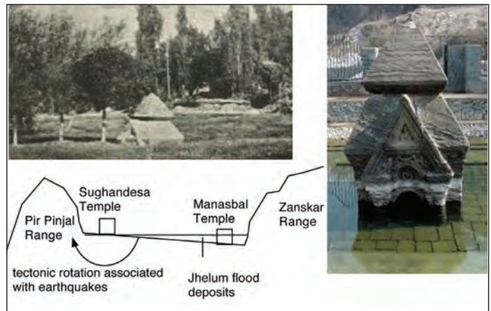
Temples on the southwest side of the Kashmir Valley have been raised and those on the southeast side lowered by tectonic processes. Annual floods of the Jhelum form a horizontal flood plane that has drowned the Manasbal Temple at an average rate of 3.3 millimeters per year since its construction in 750–830 AD. Photos show it submerged beneath fields in 1950 and excavated with its base in a pond of water in 2011.
