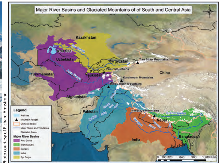
Major river systems, mountain ranges, and glacier cover across High Asia
