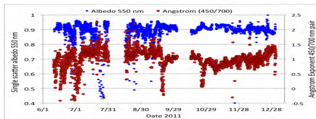
Aerosol scattering coefficient at 550nm (top frame) and aerosol single scatter albedo and Angstrom exponent (bottom frame) from 6/2011 to 12/2011 from Nainital, India.
