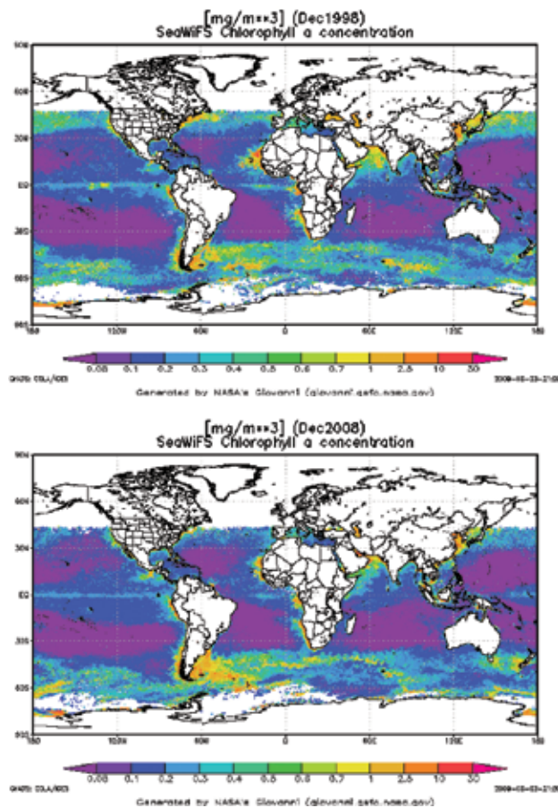
Two examples of monthly averaged chlorophyll a concentration for the month of December from SeaWiFS. Chlorophyll a concentration will be used as a measure for primary production. Note the apparent differences in surface area of oligotrophic habitat shown by the change in the surface area of depleted chlorophyll A concentrations between December 1998 and December 2008.
