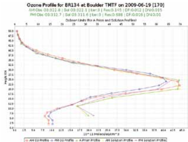
Web-based daily Brewer ozone profiles from Boulder, CO.
