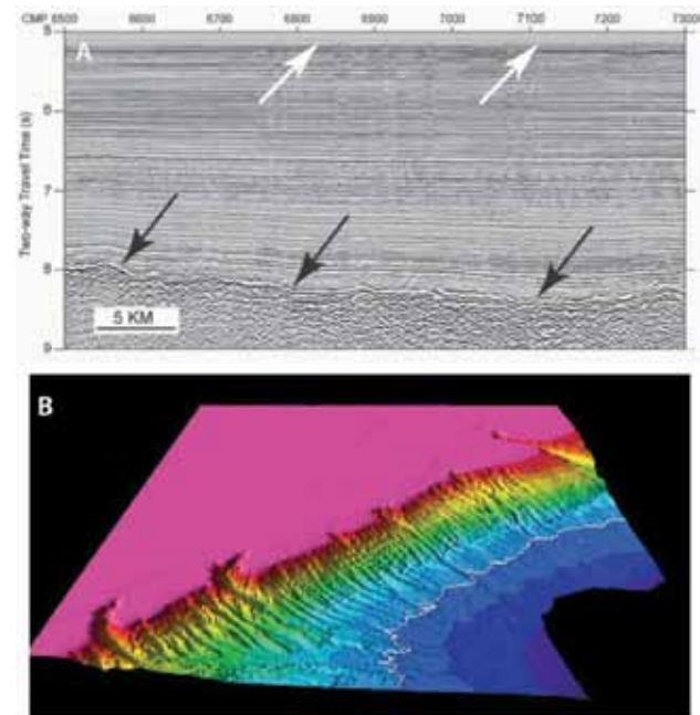
Figure 1: Examples of marine geophysical data archived and disseminated by NGDC for use in determining the extent of the U.S. ECS. a) A seismic-reflection profile across a U.S. continental margin reveals approximately 2,200 meters of visible sediment overlying oceanic basement (black arrows; seafloor indicated by white arrows). Sediment thickness is a key component in determining the extent of the U.S. ECS. b) Color, shaded-relief image of multibeam swath sonar data collected along the continental margin off New Jersey. The white line represents the 2,500-m depth contour, an important formula line used in ECS analysis. Note the morphologic detail revealed by the modern multibeam sonar survey.
