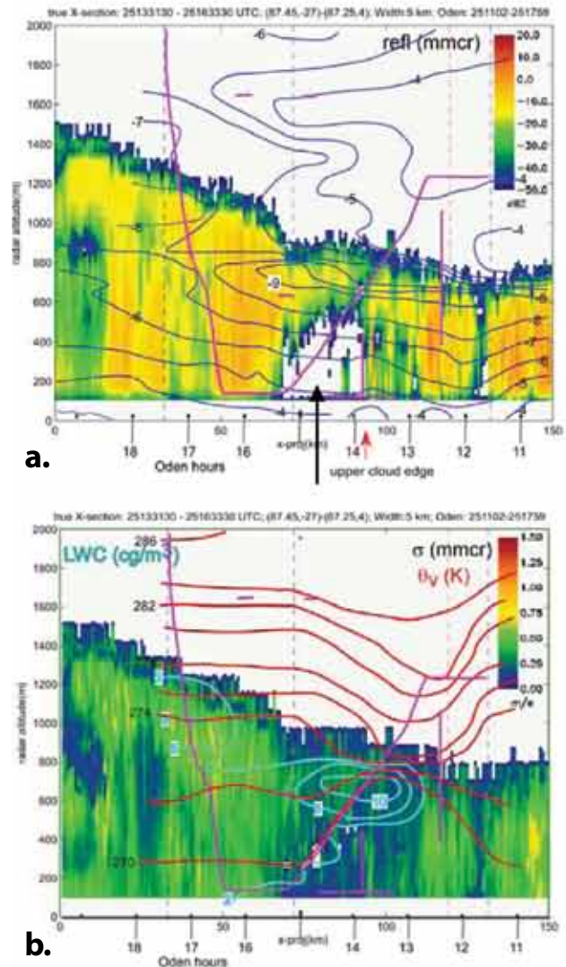
Figure 2: Time-height cross-sections of a) radar reflectivity and temperature and b) radar spectral width and liquid water content on Aug. 25, 2008. The radar data are from the Ka-band cloud radar on the Oden and the analyses are derived from the aircraft dropsondes and in situ data.
