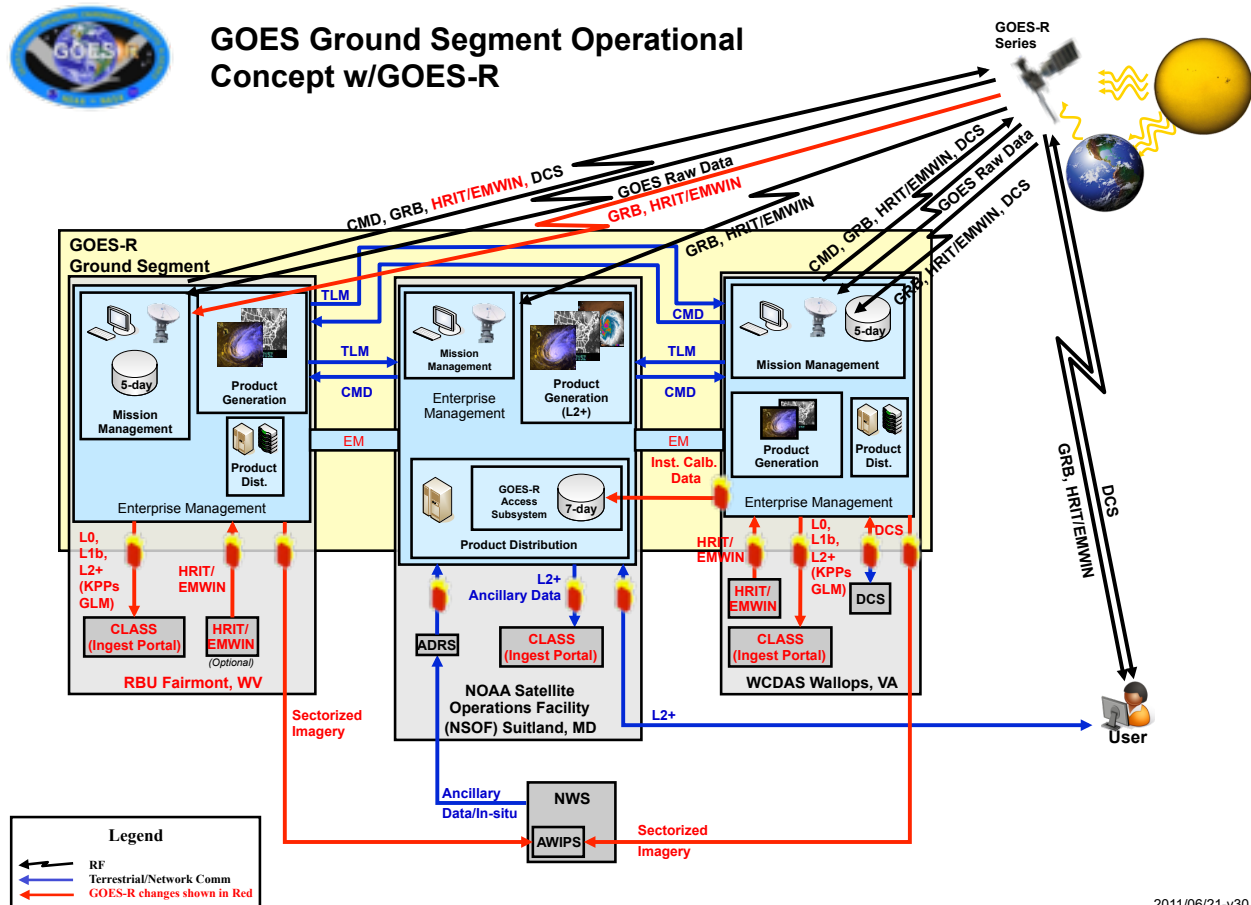
Figure 1: GOES-R Ground Segment Overview (CCR01457, CCR01661, CCR02089)
