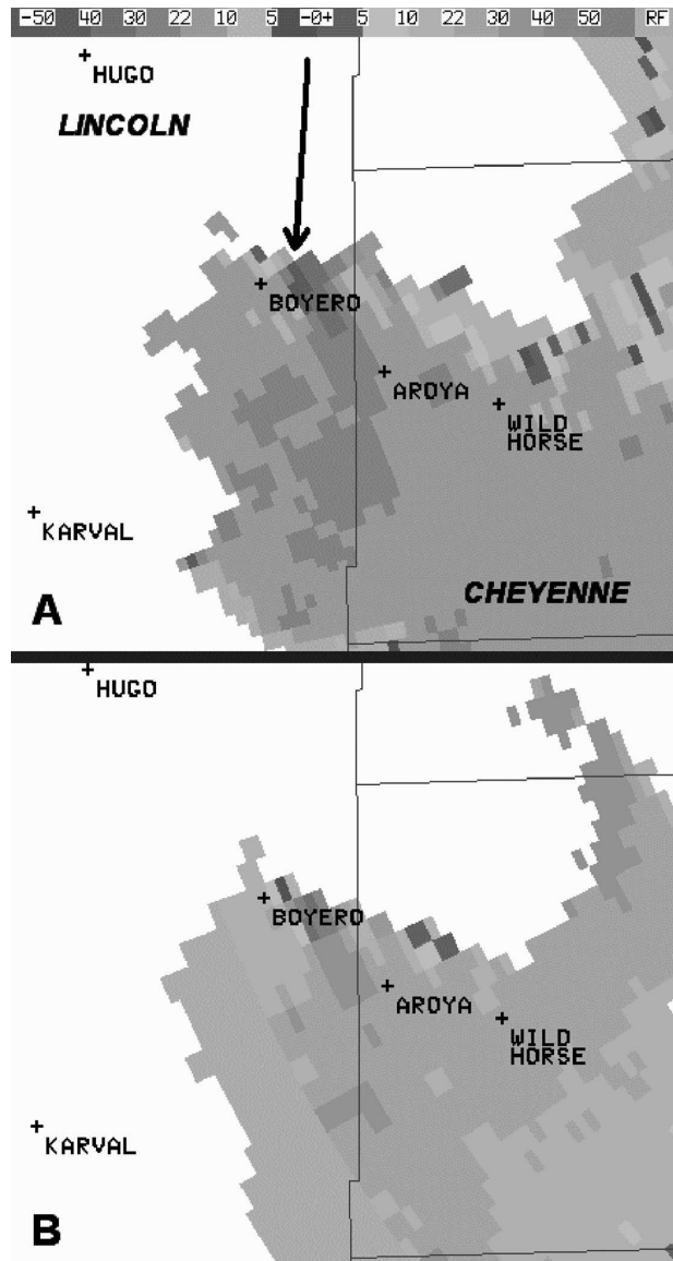
FIG. 5. The 0.5° elevation angle SRM displays at 0034 UTC 16 Jun 2002, from (a) PUX and (b) GLD. County names, arrow pointing toward mesoanticyclone center, and the velocity grayscale each are provided in (a). Locality names appear on both images, which are scaled identically. PUX and GLD radars were located generally southwest of (a) and northeast of (b), respectively. Velocities are shown in kt ( 1 \text{ kt} \approx 0.5144 \text{ m s}^{-1} ).
