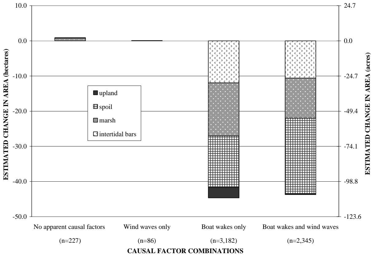
Fig.14: 1970/1971 to 2002 change in area estimated from rates of lateral movement (n = number of points exposed to each causal factor combination)
