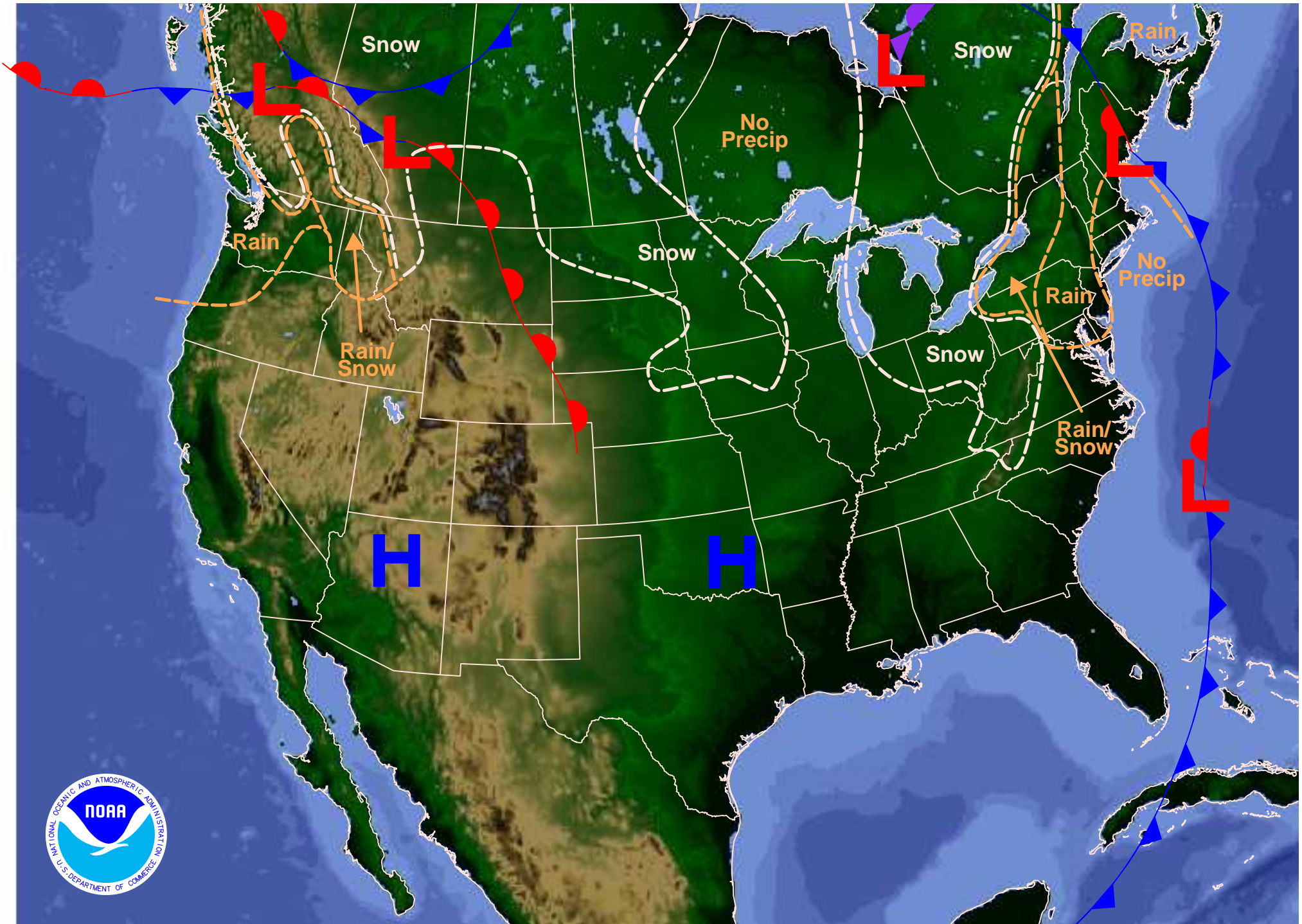
Weather Forecast for Wed, Mar 13, 2013, issued 4:35 AM EDT Tue, Mar 12, 2013 DOC/NOAA/NWS/NCEP/Weather Prediction Center Prepared by McCreynolds based on WPC, SPC and NHC forecasts
