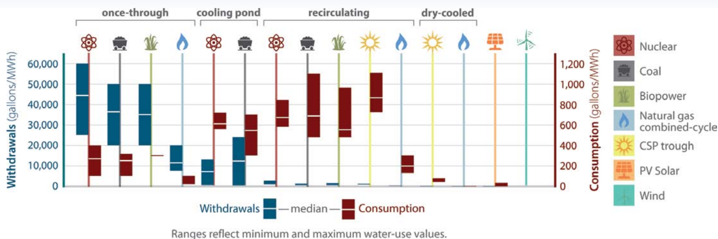
Figure 13. Water use by fuel and cooling technology
