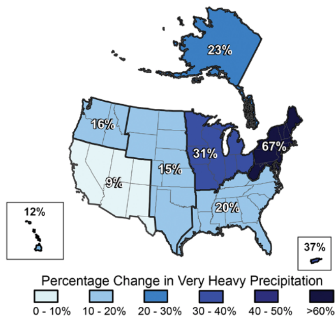
Figure 16. Percentage change in very heavy precipitation, 1958–2007
