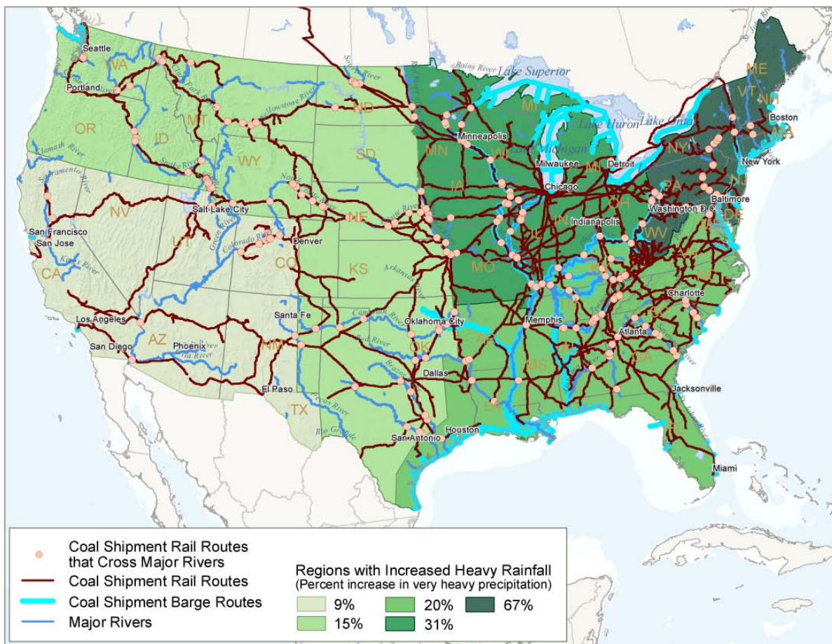
Figure 25. Regions with heavy rainfall events (1958–2007) and coal shipment routes that cross major rivers
