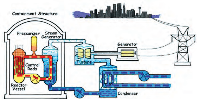
Light Water Reactor
