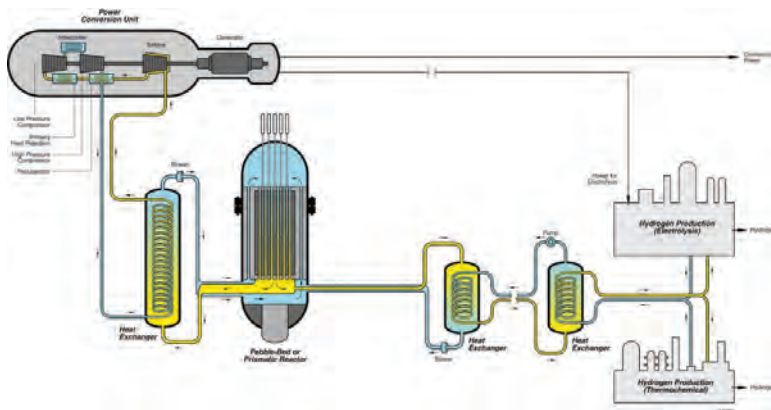
Conceptual diagram for a Very High Temperature Reactor (VHTR).
