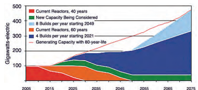
Nuclear Electricity Generation Capacity
