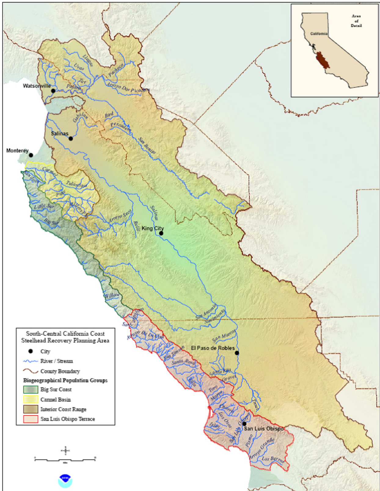
Figure 3. Four Biogeographic Population Groups (BPGs) making up the South-Central California Coast Steelhead DPS.
