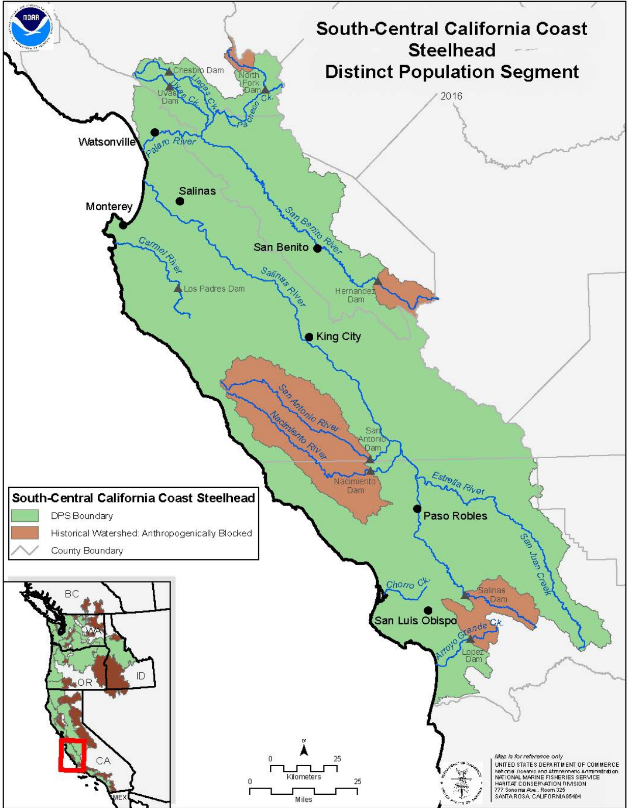
Figure 1. South-Central California Coast Steelhead DPS.
