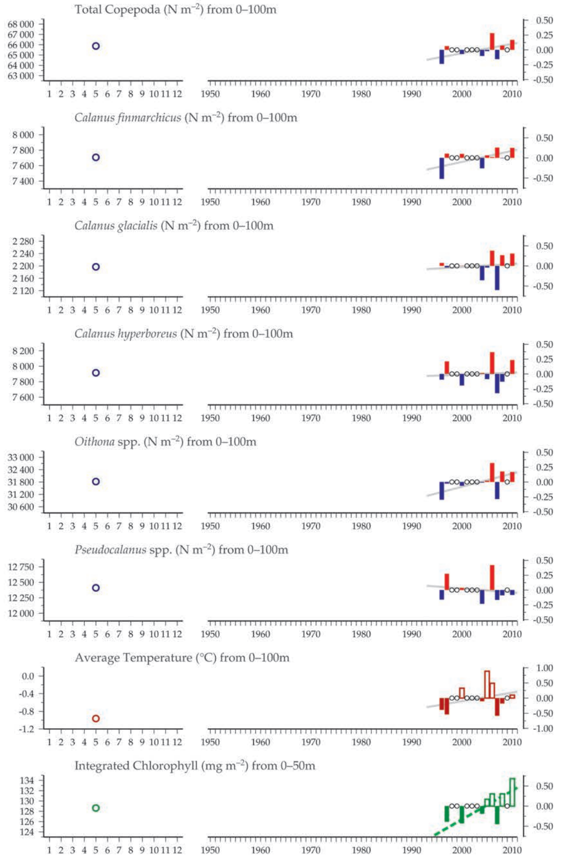
Figure 4.2.2 Multiple-variable comparison plot (see Section 2.2.2) showing the seasonal and interannual properties of select cosampled variables at the AR7W Labrador Shelf zooplankton monitoring area (data collected in late May only).
