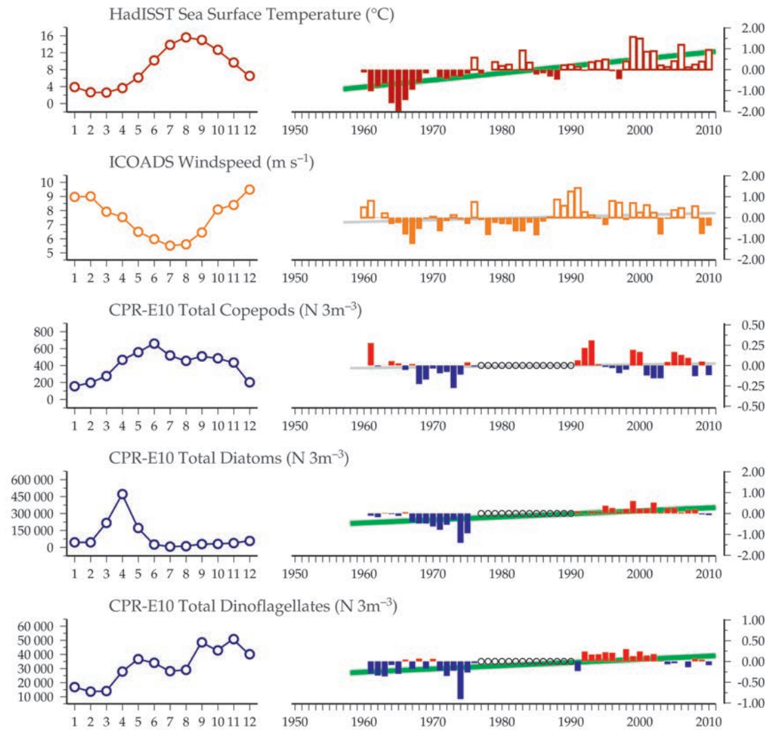
Figure 3.3.3 Regional overview plot (see Section 2.2.3) showing long-term sea surface temperatures and wind speeds in the general region surrounding the Halifax Line 2 monitoring area, along with data from the adjacent CPR E10 Standard Area.
