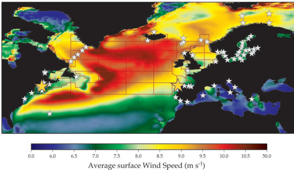
Figure 2.3.3 Map of ICOADS surface windspeed (see Section 2.3.3) overlaid with zooplankton time-series site locations (white and yellow stars) and CPR standard areas (red boxes). The lower subpanel shows examples of seasonal and interannual properties (see Section 2.2.2) of ICOADS surface windspeed from the Scotian Shelf (left-most yellow star, see also Site 6 in Section 3.3) and Northwest Iberian Coast (right-most yellow star, see also Site 52 in Section 8.4).
