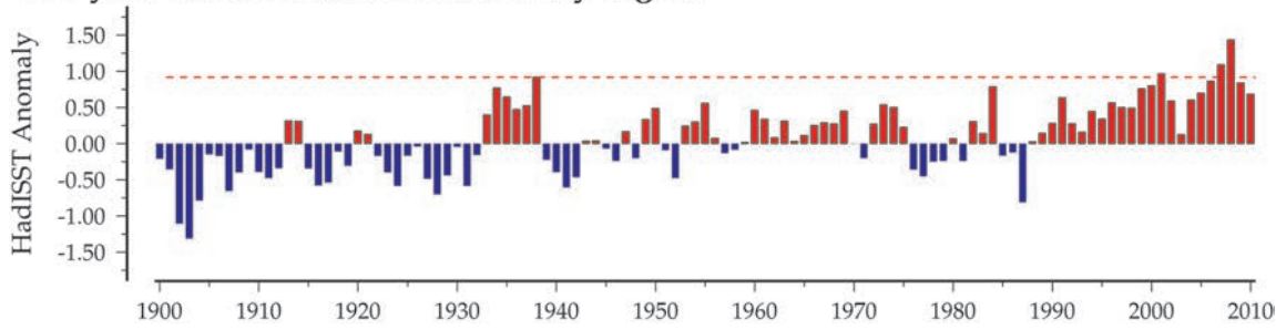
Figure 6.1.11 Regional overview plot (see Section 2.2.3) showing 100-year sea surface temperatures in the general region surrounding the Northern Baltic Sea monitoring areas.
