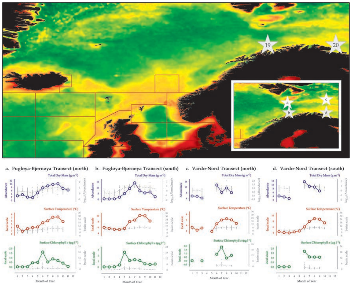
Figure 5.4.1 Location of the Fugløya–Bjørnøya and Vardø–Nord transects (Sites 19 and 20) zooplankton monitoring areas, plotted on a map of average chlorophyll concentration, and their corresponding environmental summary plots (see Section 2.2.1).
