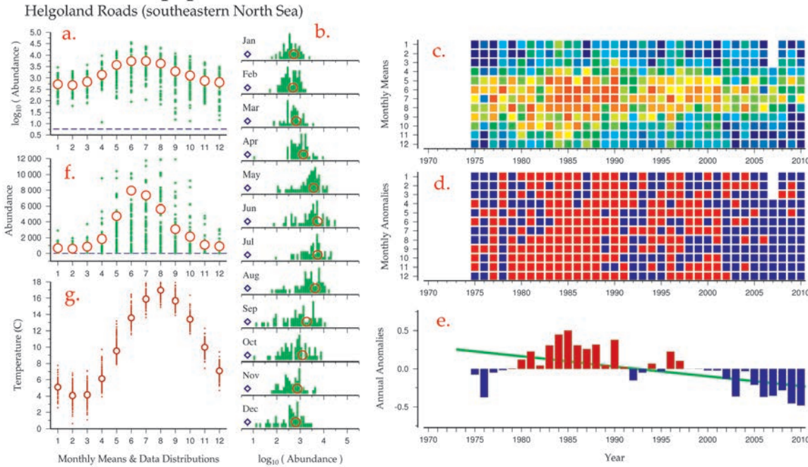
Figure 2.1.1 A collection of standard WGZE time-series visualization figures illustrating the steps and components used in the WGZE analysis for creating annual anomalies of total small copepod abundance from the Helgoland Roads time-series (Site 45, see Section 7.2 for more information on this site).
