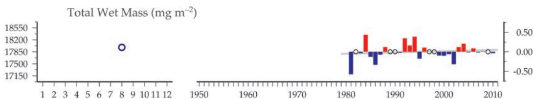
Figure 6.1.5 Multiple-variable comparison plot (see Section 2.2.2) showing the seasonal and interannual properties of total zooplankton wet mass values within the four northern Baltic Sea monitoring regions.
