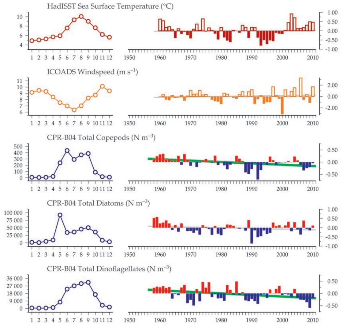
Figure 5.2.7 Regional overview plot (see Section 2.2.3) showing long-term sea surface temperatures and wind speeds in the general region surrounding the Faroe Islands monitoring area.
