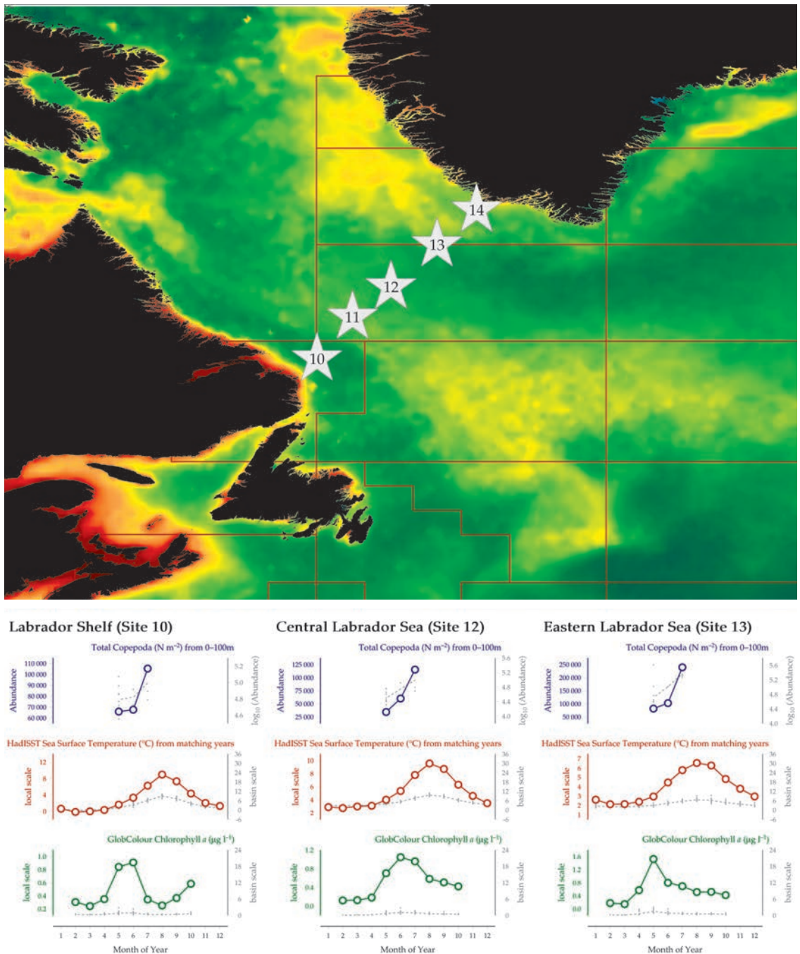
Figure 4.2.1 Location of the AR7W Section monitoring areas (Sites 10–14), plotted on a map of average chlorophyll concentration, with corresponding seasonal summary plots (only for sites 10, 12, and 13) shown in the lower panel (see also Section 2.2.1).
