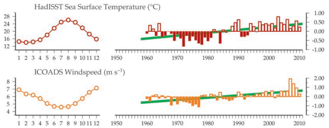
Figure 9.2.3 Regional overview plot (see Section 2.2.3) showing long-term sea surface temperatures and windspeeds in the general region surrounding the Balears Station monitoring area.
