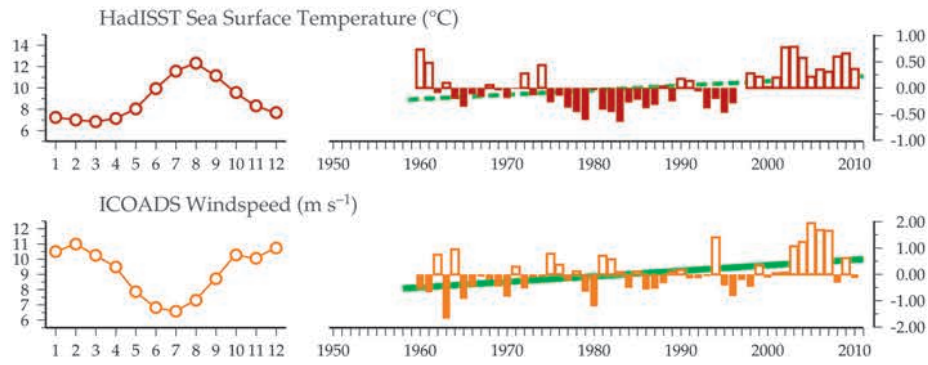
Figure 5.3.3 Regional overview plot (see Section 2.2.3) showing long-term sea surface temperatures and wind speeds in the general region surrounding the Svinøy transect, along with data from the adjacent CPR B01 Standard Area.
