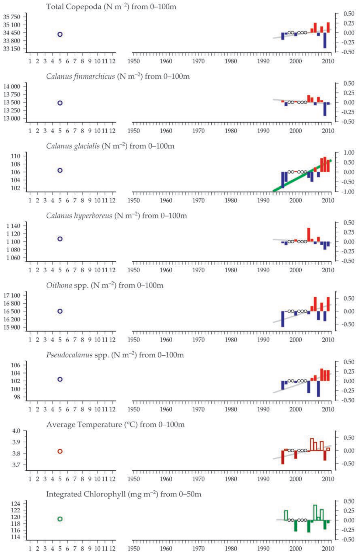
Figure 4.2.4 Multiple-variable comparison plot (see Section 2.2.2) showing the seasonal and interannual properties of select cosampled variables at the AR7W Central Labrador Sea zooplankton monitoring area (data collected in late May only).
