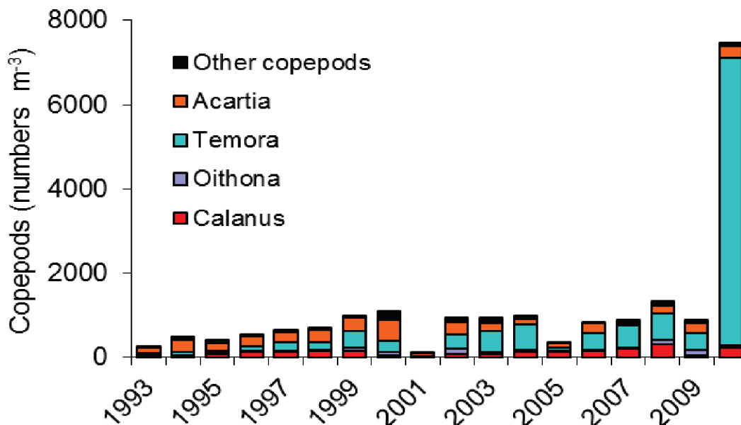
Figure 5.2.6 Mean abundance of copepods on the Faroe Shelf in late June.
