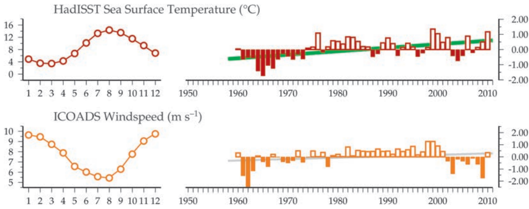
Figure 3.2.3 Regional overview plot (see Section 2.2.3) showing long-term sea surface temperatures and wind speeds in the general region surrounding the Prince 5 monitoring area.
