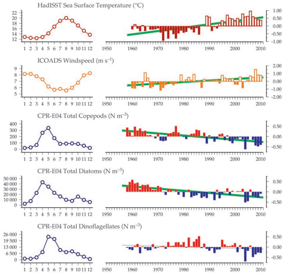
Figure 8.3.3 Regional overview plot (see Section 2.2.3) showing long-term sea surface temperatures and windspeeds in the general region surrounding the Gijón/Xixón Transect monitoring area, along with data from the adjacent CPR E04 Standard Area.
