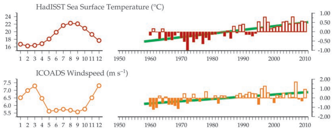
Figure 8.7.3 Regional overview plot (see Section 2.2.3) showing long-term sea surface temperatures and wind speeds in the general region surrounding the Guadiana Lower Estuary monitoring area.
