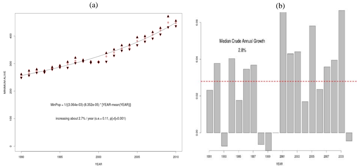
Figure 1. Minimum number alive (a) and crude annual growth rate (b) for catalogued North Atlantic right whales. Minimum number ( N ) of catalogued individuals known to be alive in any given year includes all whales known to be alive prior to that year and seen in that year or subsequently plus all whales newly catalogued that year. Catalogued whales may include some but not all calves produced each year. Bracketing the minimum number of catalogued whales is the number without calves (below) and that plus calves above, the latter which yields N_{min} for purposes of stock assessment. Mean crude growth rate (dashed line) is the exponentiated mean of \log_e [(N_{t+1}-N_t)/N_t] for each year ( t ).
