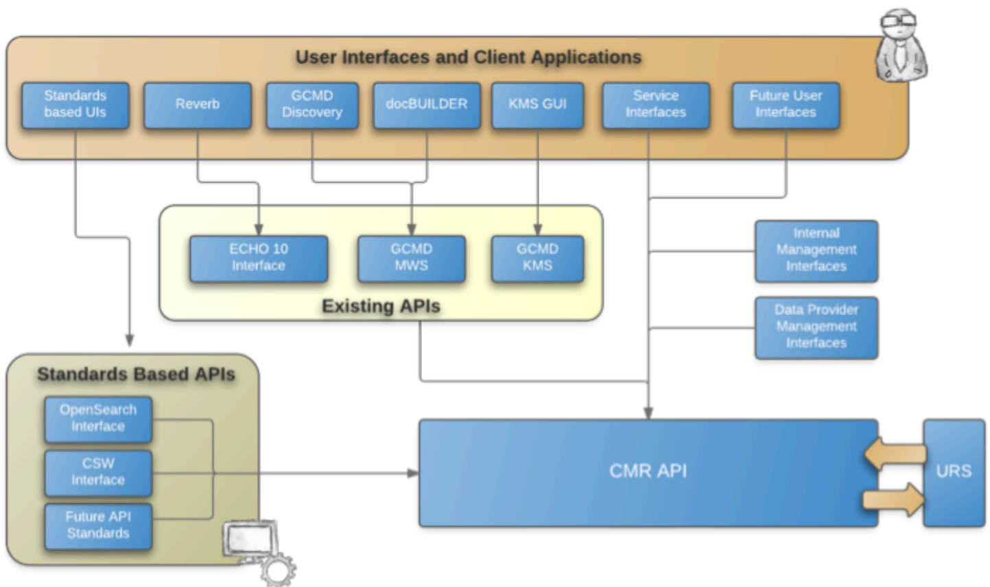
Figure 8: High level overview of key CMR interfaces
