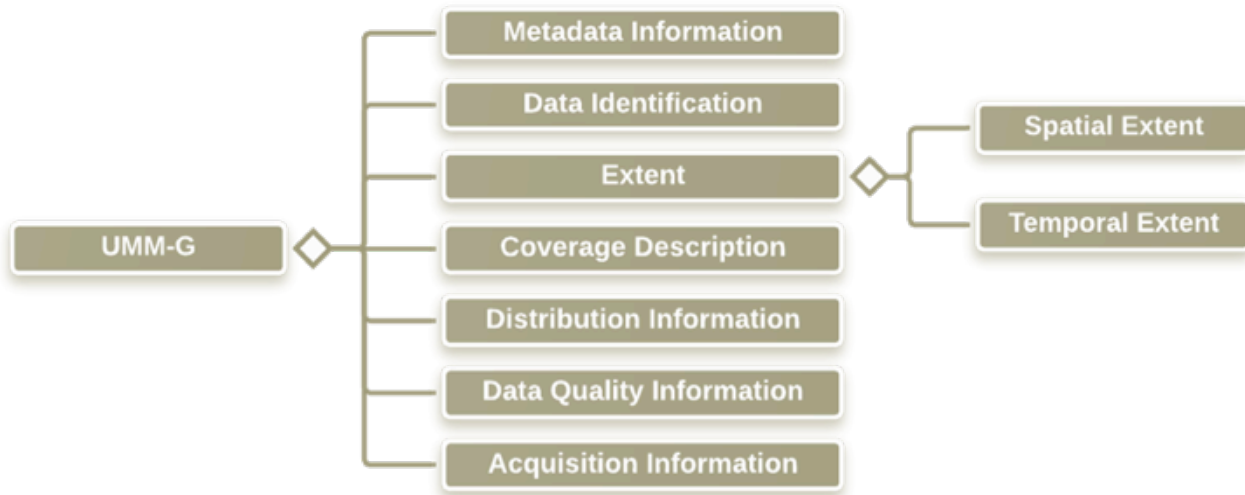
Figure 18: Top level elements of a Granule in UMM-G
