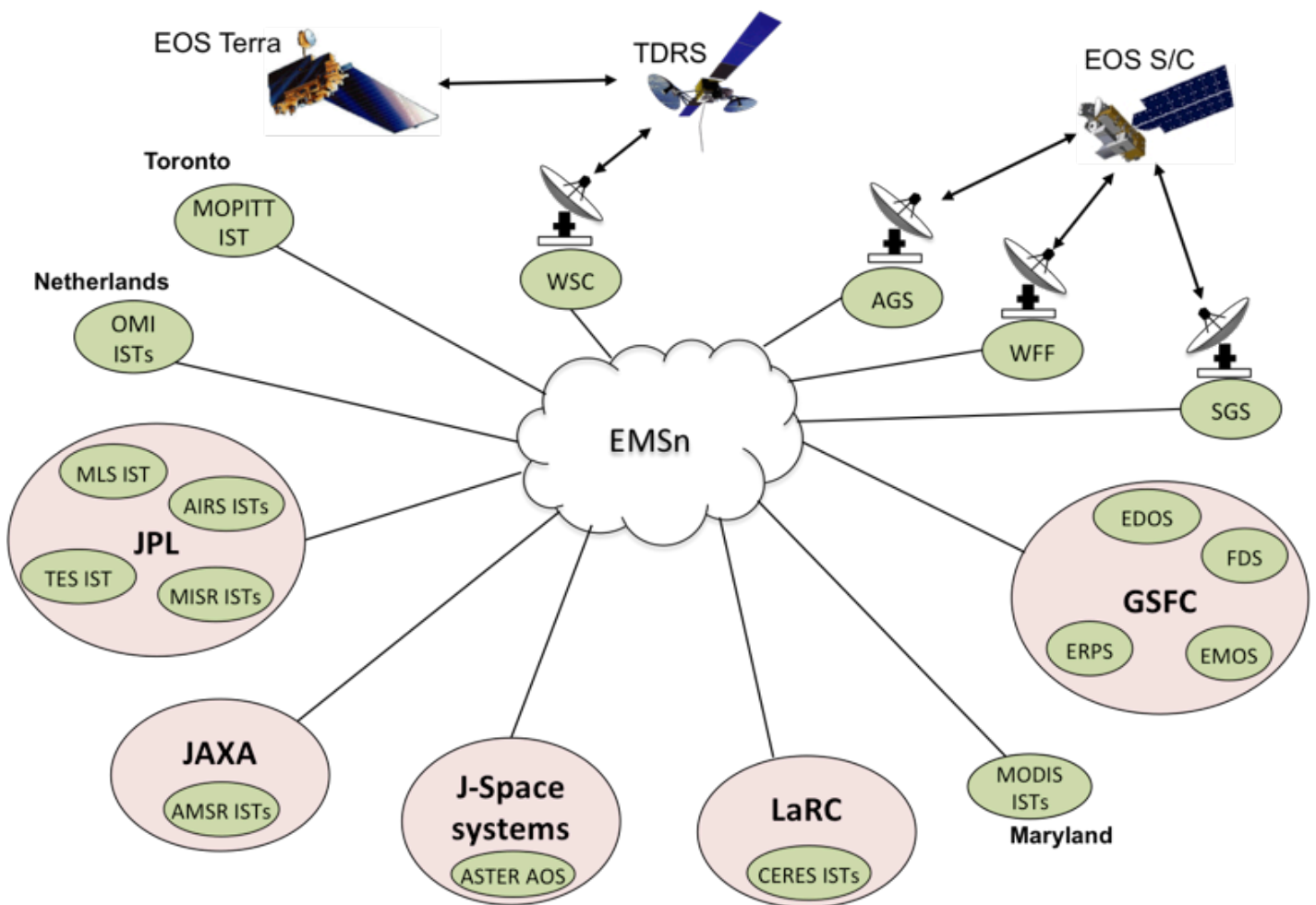
Figure 5: EMSn Logical Network. The EMSn provides mission operations and critical data transfer for EOSDIS
