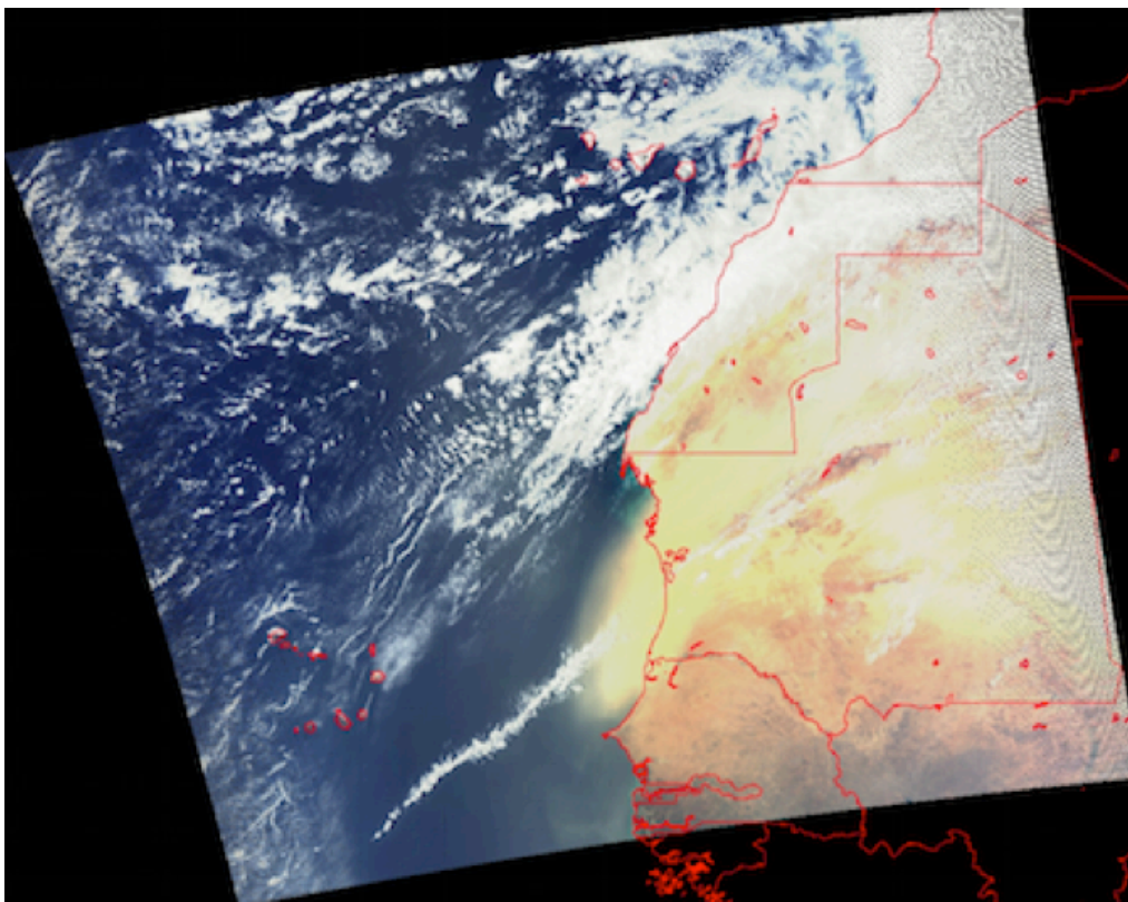
Figure 14: Level 1B Calibrated Radiance from MODIS on Aqua, 28 March 2008. The image approximates true color, using MODIS Band 1 for Red, band 4 for Green, and band 3 for Blue.
