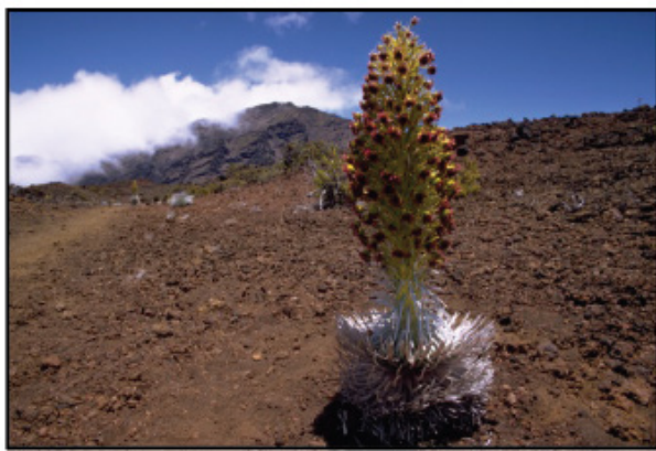
Figure 23.5. Warming at high elevations could alter the distribution of native plants and animals in mountainous ecosystems and increase the threat of invasive species. The threatened, endemic 'ahinahina, or Haleakalā silversword ( Argyroxiphium sandwicense subsp. macrocephalum ), shown here in full bloom on Maui, Hawaiian Islands, is one example. (Photo credit: Forest and Kim Starr).
