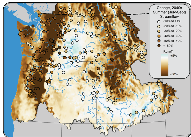
Figure 21.2. (Left) Projected increased winter flows and decreased summer flows in many Northwest rivers will cause widespread impacts. Mixed rain-snow watersheds, such as the Yakima River basin, an important agricultural area in eastern Washington, will see increased winter flows, earlier spring peak flows, and decreased summer flows in a warming climate. Changes in average monthly streamflow by the 2020s, 2040s, and 2080s (as compared to the period 1916 to 2006) indicate that the Yakima River basin could change from a snow-dominant to a rain-dominant basin by the 2080s under the A1B emissions scenario (with eventual reductions from current rising emissions trends). (Figure source: adapted from Elsner et al. 2010) 24 .
