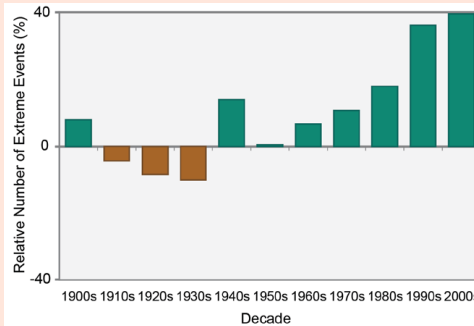
Figure 2.16: One measure of a heavy precipitation event is a 2-day precipitation total that is exceeded on average only once in a five-year period, also known as a once-in-five-year event. As this extreme precipitation index for 1901-2012 shows, the occurrence of such events has become much more common in recent decades. Changes are compared to the period 1901-1960, and do not include Alaska or Hawai'i. The 2000s decade (far right bar) includes 2001-2012. (Figure source: adapted from Kunkel et al. 2013 52 ).
