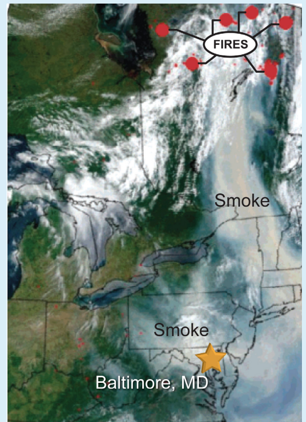
Figure 9.3. Wildfires, which are projected to increase in some regions due to climate change, have health impacts that can extend hundreds of miles. Shown here, forest fires in Quebec, Canada, during July 2002 (red circles) resulted in up to a 30-fold increase in airborne fine particle concentrations in Baltimore, Maryland, a city nearly a thousand miles downwind. These fine particles, which are extremely harmful to human health, not only affect outdoor air quality, but also penetrate indoors, increasing the long-distance effects of fires on health. 41 An average of 6.4 million acres burned in U.S. wildfires each year between 2000 and 2010, with 9.5 and 9.1 million acres burned in 2006 and 2012, respectively. 42 Total global deaths from the effects of landscape fire smoke have been estimated at 260,000 to 600,000 annually between the years 1997 and 2006. 37 (Figure source: Moderate Resolution Imaging Spectroradiometer (MODIS) instrument on the Terra satellite, Land Rapid Response Team, NASA/GSFC).
