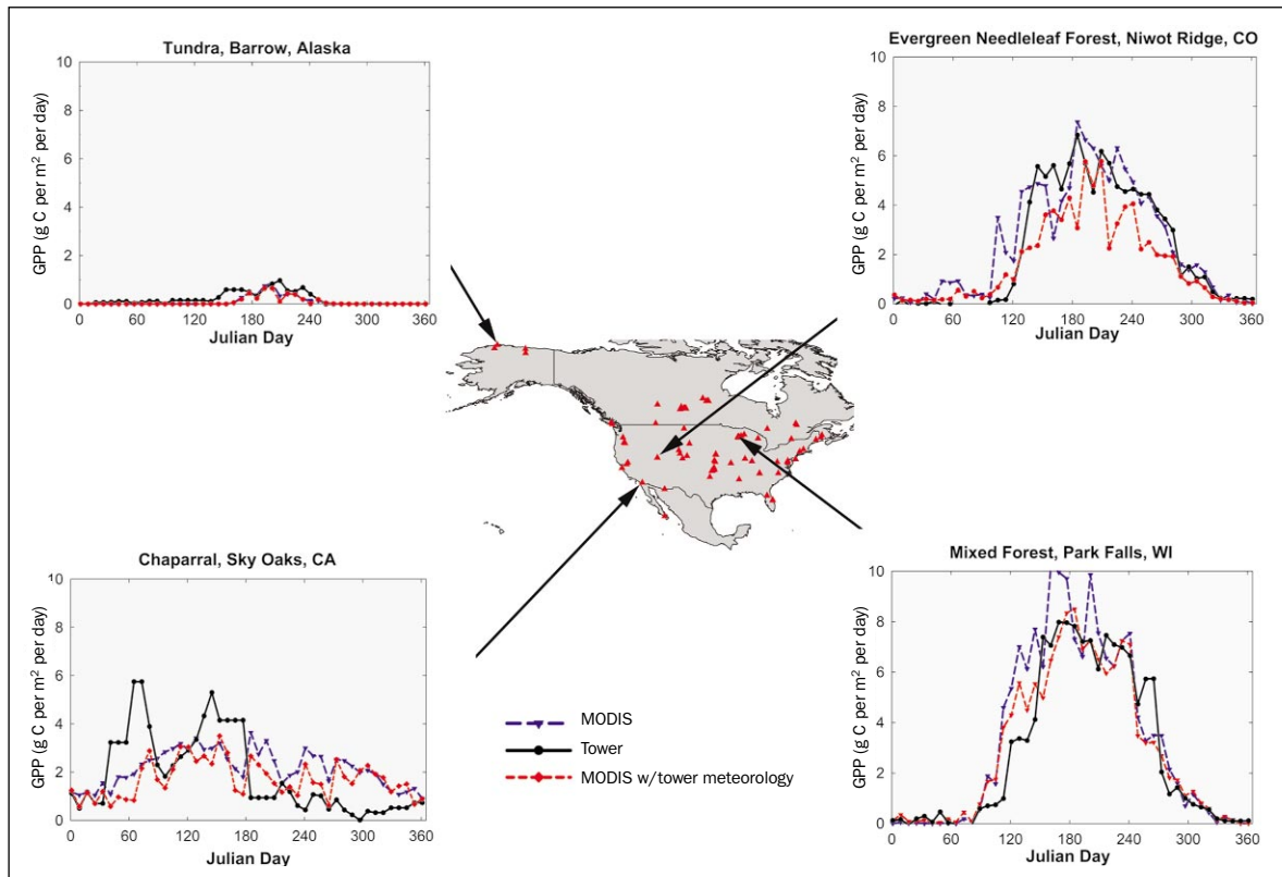
Figure 7. Intercomparison of gross primary production (GPP) computed from daily MODIS (Moderate Resolution Imaging Spectroradiometer) data summed at 8-day intervals with GPP measurements from flux towers at sites in the AmeriFlux network that represent different biomes and climatic regimes for 2001. Substituting higher-resolution (1 to 5 km) daily local tower meteorology data for the lower-resolution ( 1^\circ by 1.25^\circ ) global meteorology data in a replicated calculation of GPP allows separation of error sources in the MODIS algorithms.
