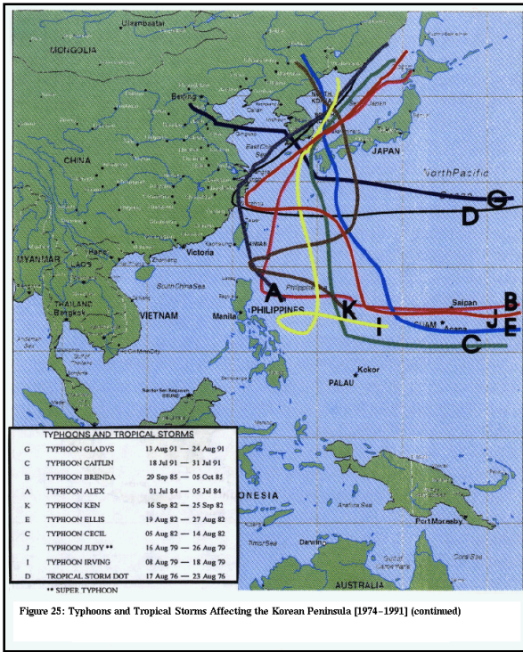
Typhoons and Tropical Storms Affecting the Korean Peninsula [1974 – 1991] (Figure 25)
