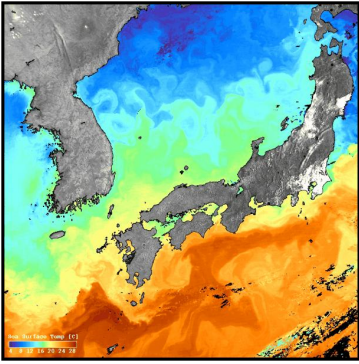
Kuroshio Current (warm) and Oyashio Current (Cold) (Figure 14)
