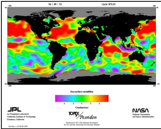
Sea Surface Variability – 09/15/94 (Figure 20B)
