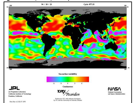
Sea Surface Variability – 10/25/94 (Figure 20C)
