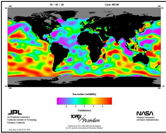
Sea Surface Variability – 01/28/95 (Figure 20E)
