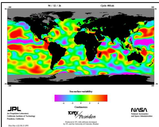
Sea Surface Variability – 12/26/94 (Figure 20D)
