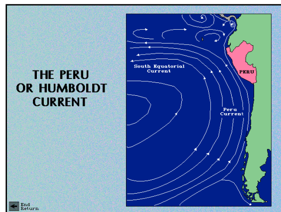
The Peru or Humboldt Current (Figure 1)
