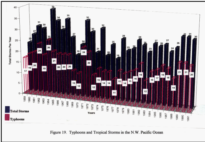
Typhoons and Tropical Storms in the N.W. Pacific Ocean (Figure 19)
