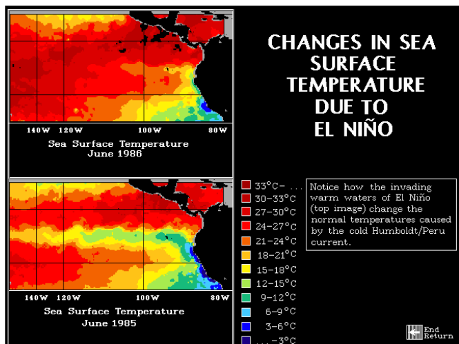
Changes in Sea Surface Temperature due to El Niño (Figure 2)
