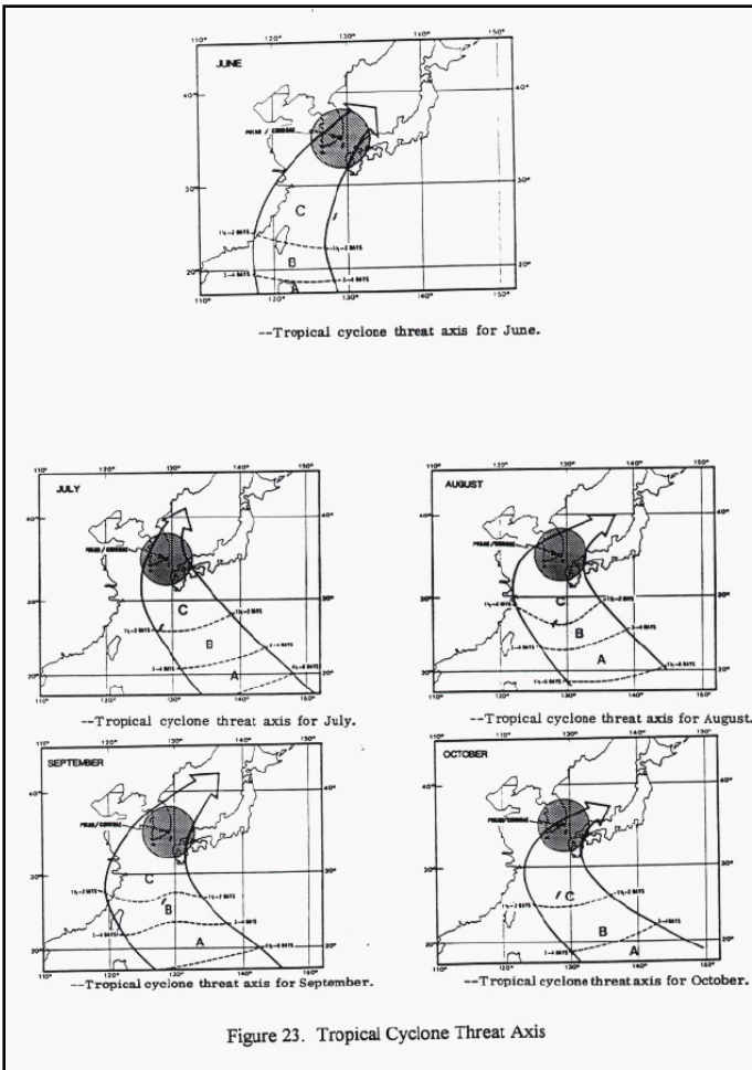
Tropical Cyclone Threat Axis (June, July, August, September, and October) (Figure 23)
