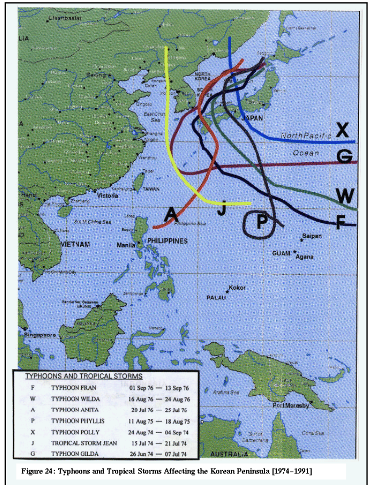
Typhoons and Tropical Storms Affecting the Korean Peninsula [1974 – 1991] (Figure 24)
