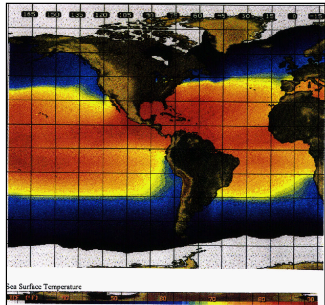
Global Sea Surface Temperature Maps – 07/23/95 (Figure 21B)
