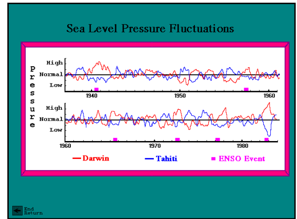
Darwin – Tahiti Annual Pressure Change (Figure 4)
