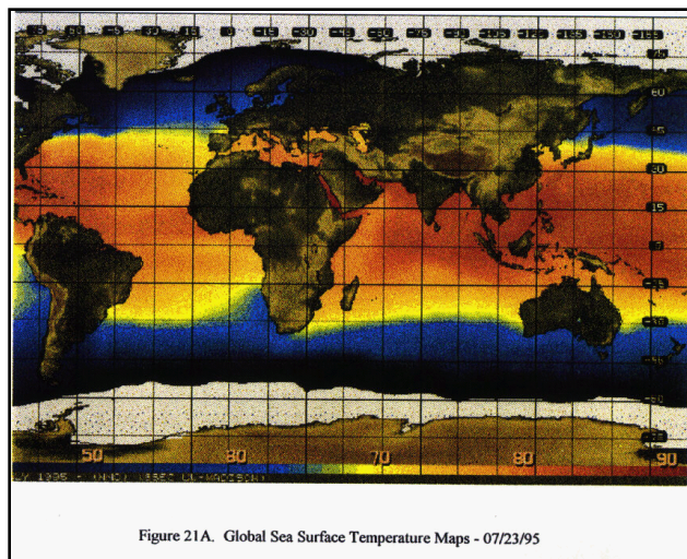
Global Sea Surface Temperature Maps – 07/23/95 (Figure 21A)
