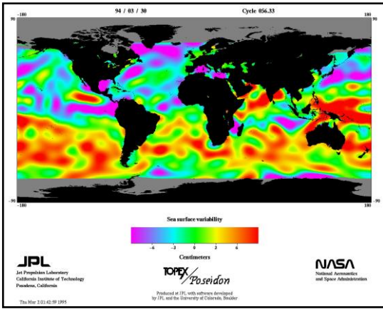
Sea Surface Variability – 03/30/94 (Figure 20A)
