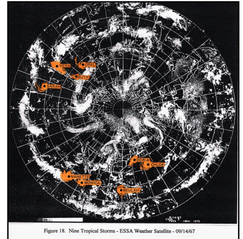
Nine Tropical Storms ESSA Weather Satellite 09/14/67 (Figure 18)
