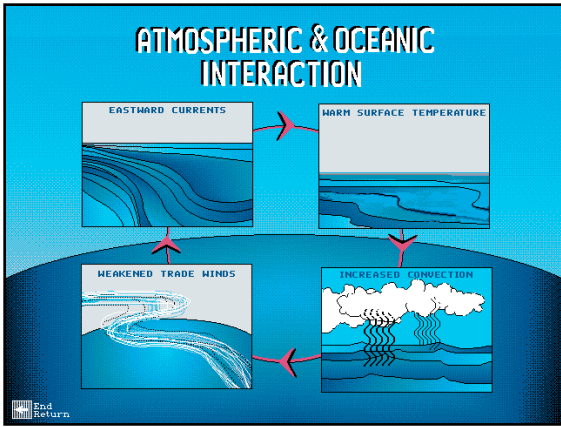
Atmospheric and Oceanic Interaction (Figure 3)
