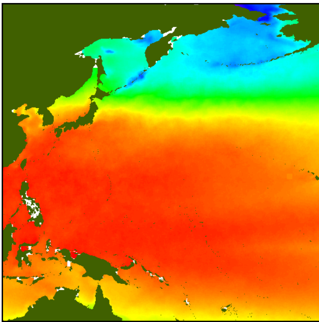
Modern Average Global Sea Surface Temperature in the N.W. Pacific Ocean (Figure 22)
