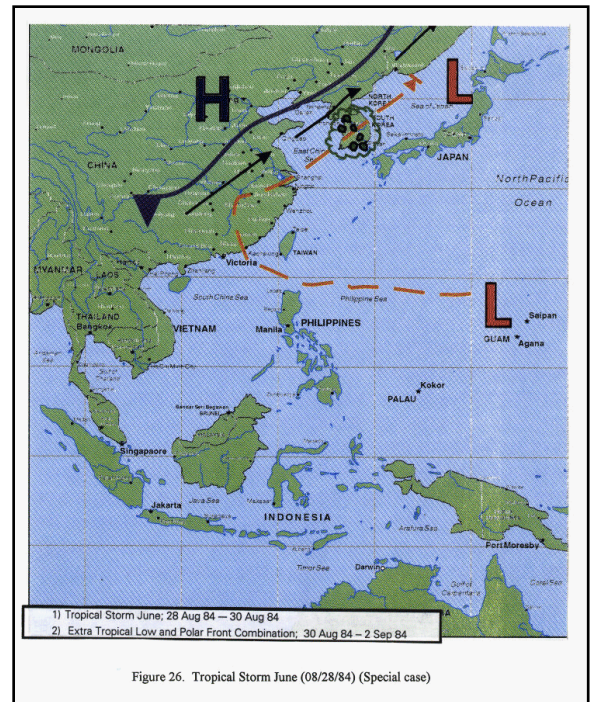
Tropical Storm June [08/28/84] (Figure 26)
