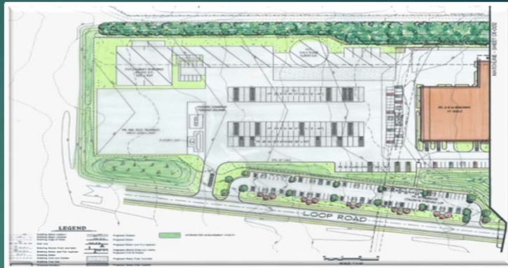
Ft. Detrick Hazardous Material Storage Building
