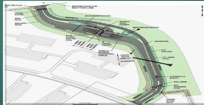
East Campus Vehicle Control Point 'M'
