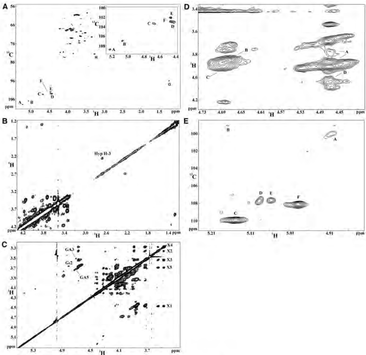
Figure 3. NMR Spectra of YS1-HP2627 Collected at 25°C on a Varian VNMRs 800 Instrument.
