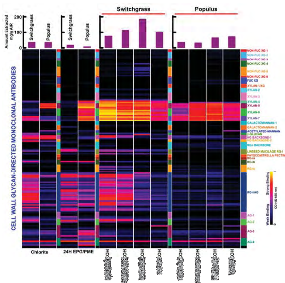
Figure 3. Glycome Profiling of single step extracts of poplar and switchgrass cell wall samples. Individual chemical (0.1M KOH/24 hr, 0.25M KOH/24 hr, 0.5M KOH/24 hr, and 1M KOH/1 hr) and enzymatic (EPG/PME) extractions were carried out on AIR from both biomass samples as described in Materials & Methods. In order to characterize which cell wall glycans were released from the cell walls by each of these extractions, the solubilized extracts were loaded onto the ELISA plates and screened against an array of plant glycan-directed monoclonal antibodies (Supplemental Information, Table S1). Antibody binding is represented as colored heat maps, with black signifying no binding, pink/red representing intermediate binding, and bright yellow representing the strongest binding. The bar graphs at the top indicate the amount of material recovered in the solubilized extracts per gram of AIR.
