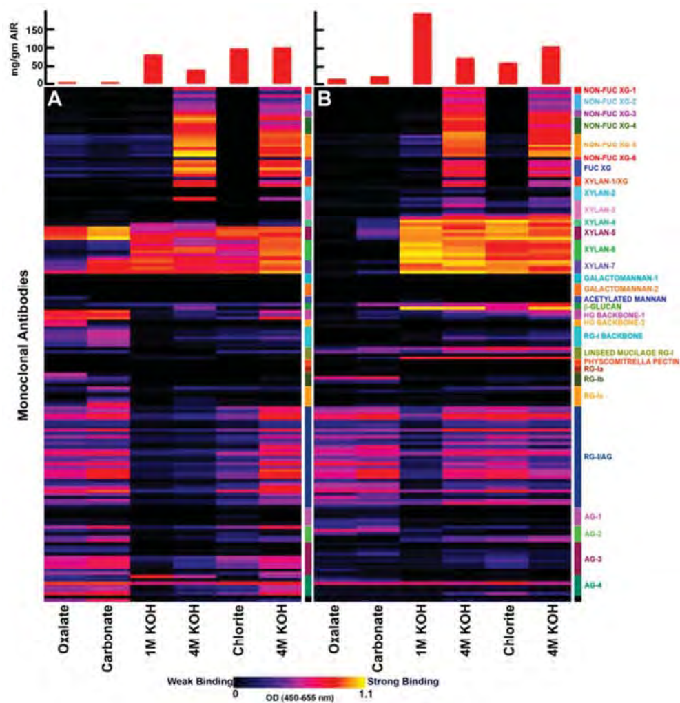
Figure 2. Glycome Profiling of unpretreated poplar and switchgrass biomass. Sequential extracts of alcohol insoluble residues (AIR) of each biomass were prepared by treatment with various reagents (as labeled at the bottom of each heatmap). Extracts were loaded onto ELISA plates and screened against an array of plant glycan-directed monoclonal antibodies (see Supplemental Information, Table S1). The legend panel on the right of the figure displays the identity of the polysaccharides predominantly recognized by each group of mAbs. Antibody binding is represented as colored heat maps, with black signifying no binding, pink/red representing intermediate binding, and bright yellow representing the strongest binding. The bar graphs at the top indicate the amount of soluble material recovered at each extraction step per gram of alcohol insoluble residue (AIR).
