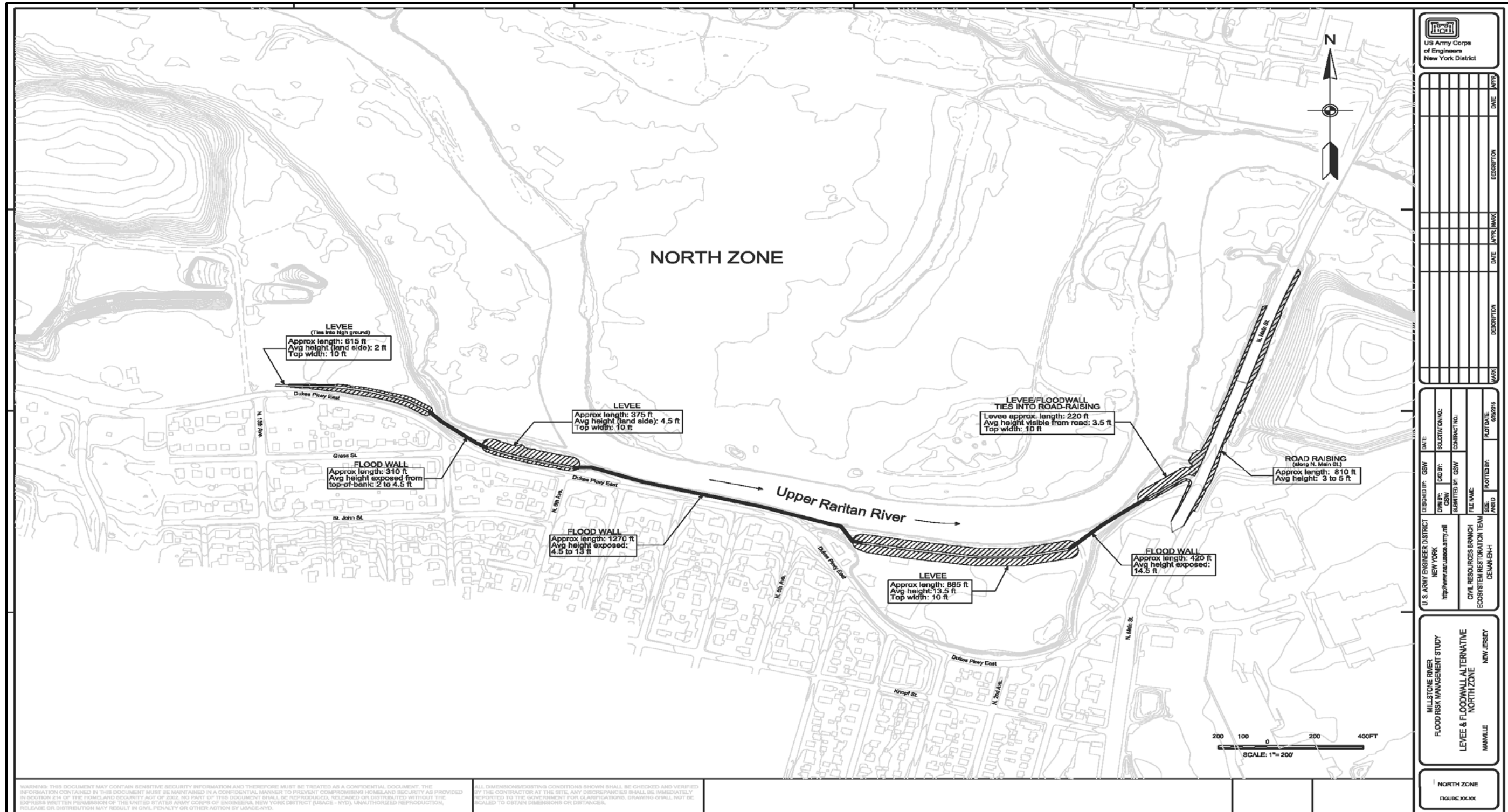
FIGURE 58:LEVEE & FLOODWALL PLAN LAYOUT (SHEET 2 OF 4)
