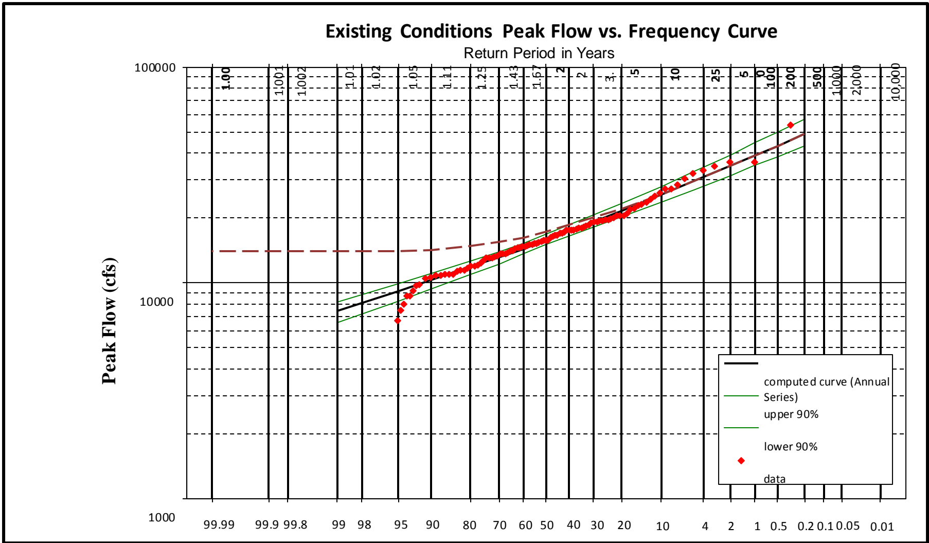
FIGURE 8: PEAK DISCHARGE VS. FREQUENCY CURVE FOR RARITAN RIVER AT MANVILLE, NJ (D.A. = 490 MI 2 )
