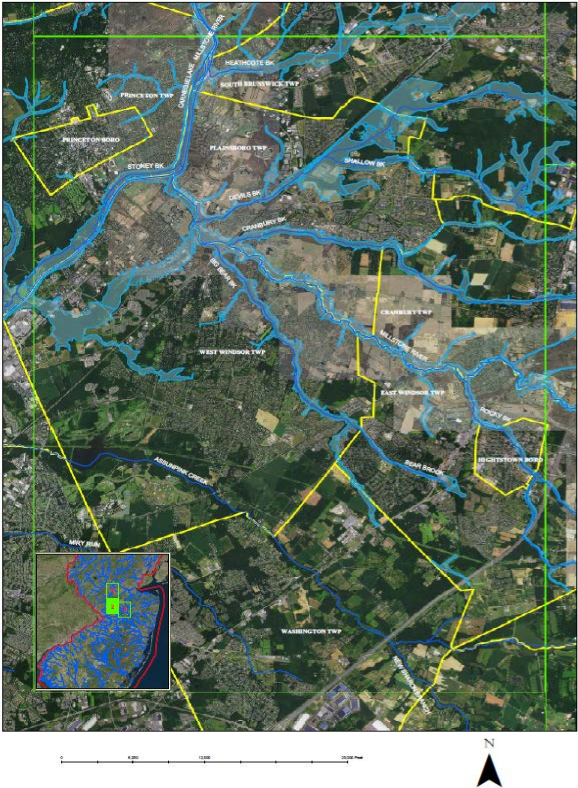
Figure 2: Millstone River Basin with 1% Annual Chance Exceedance Floodplain
