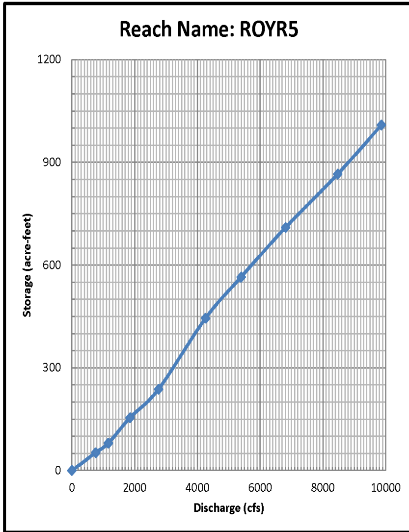
FIGURE 4 (C): MODIFIED PULS ROUTING RELATIONS
