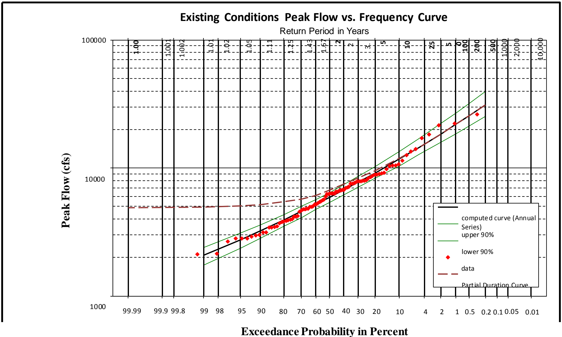
FIGURE 9: PEAK DISCHARGE VS. FREQUENCY CURVE FOR MILLSTONE RIVER AT BLACKWELLS MILLS, NJ (D.A. = 258 m 2 )
