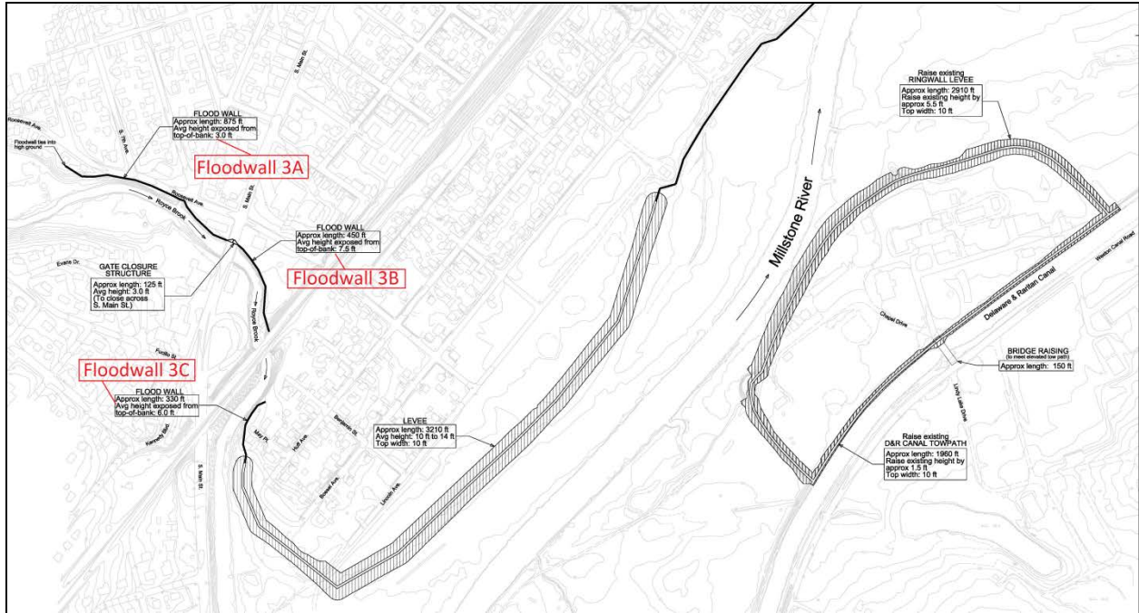
Figure 4: Site contents of the South Zone
