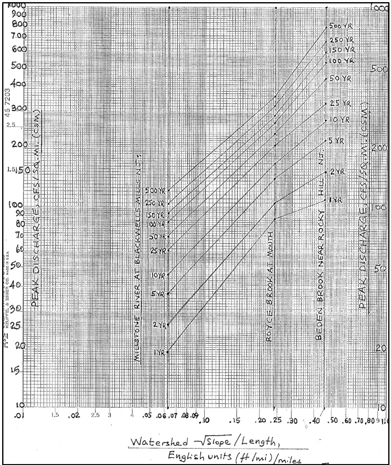
FIGURE 12: INTERPOLATION OF PEAK DISCHARGE VS. FREQUENCY FOR ROYCE BROOK AT MOUTH
