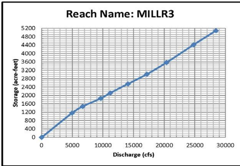
FIGURE 4 (B): MODIFIED PULS ROUTING RELATIONS
