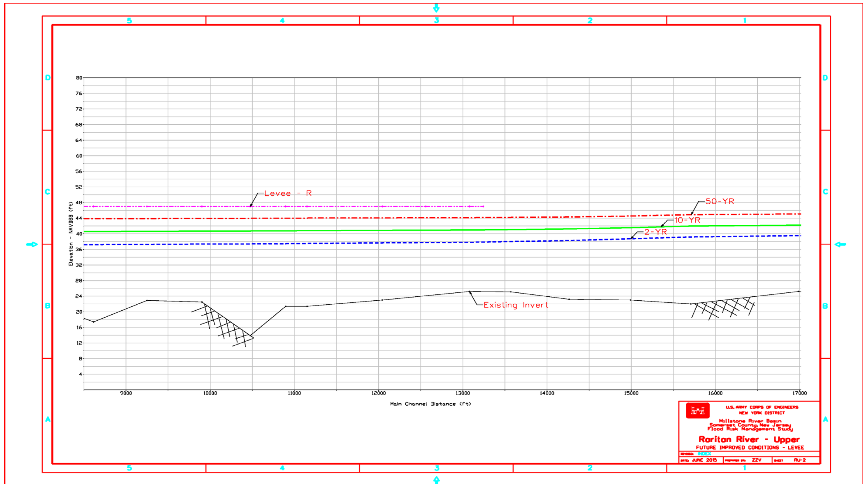
FIGURE 63: MAXIMUM WATER SURFACE PROFILE FOR LEVEE & FLOODWALL PLAN - FUTURE IMPROVED CONDITIONS (RARITAN RIVER UPPER)
