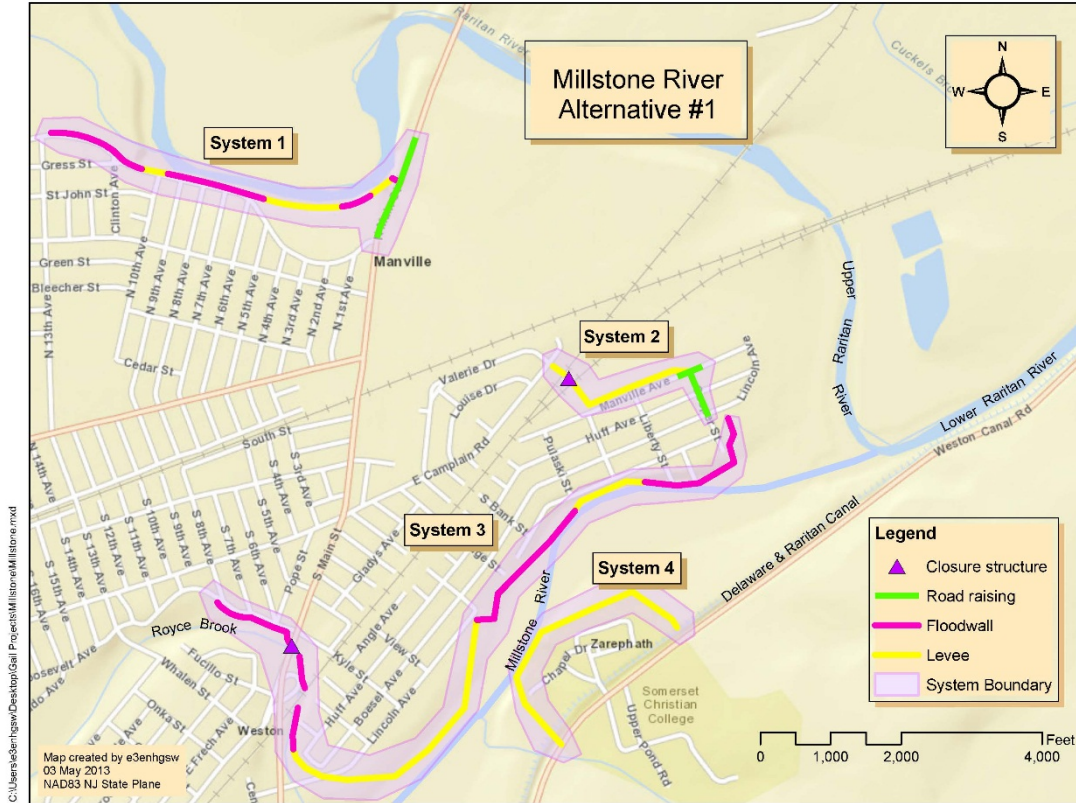
Figure 1: Alternative 1 – Levee/Floodwall System
