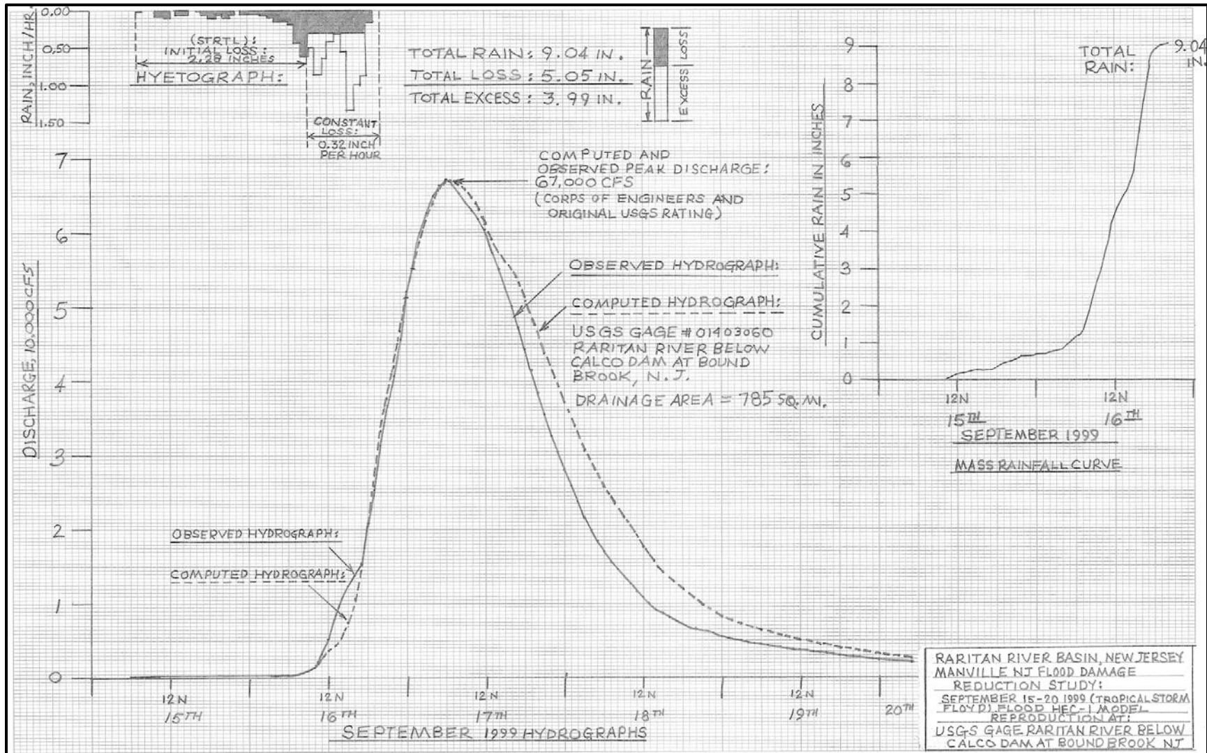
FIGURE 6: SEPTEMBER 15 – 16 1999 (TS FLOYD) FLOOD MODEL REPRODUCTION AT THE CALCO DAM GAGE.
