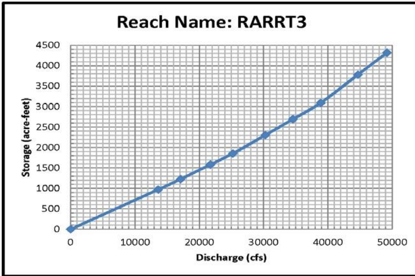
Figure 4 (A): Modified Puls Routing Relations
