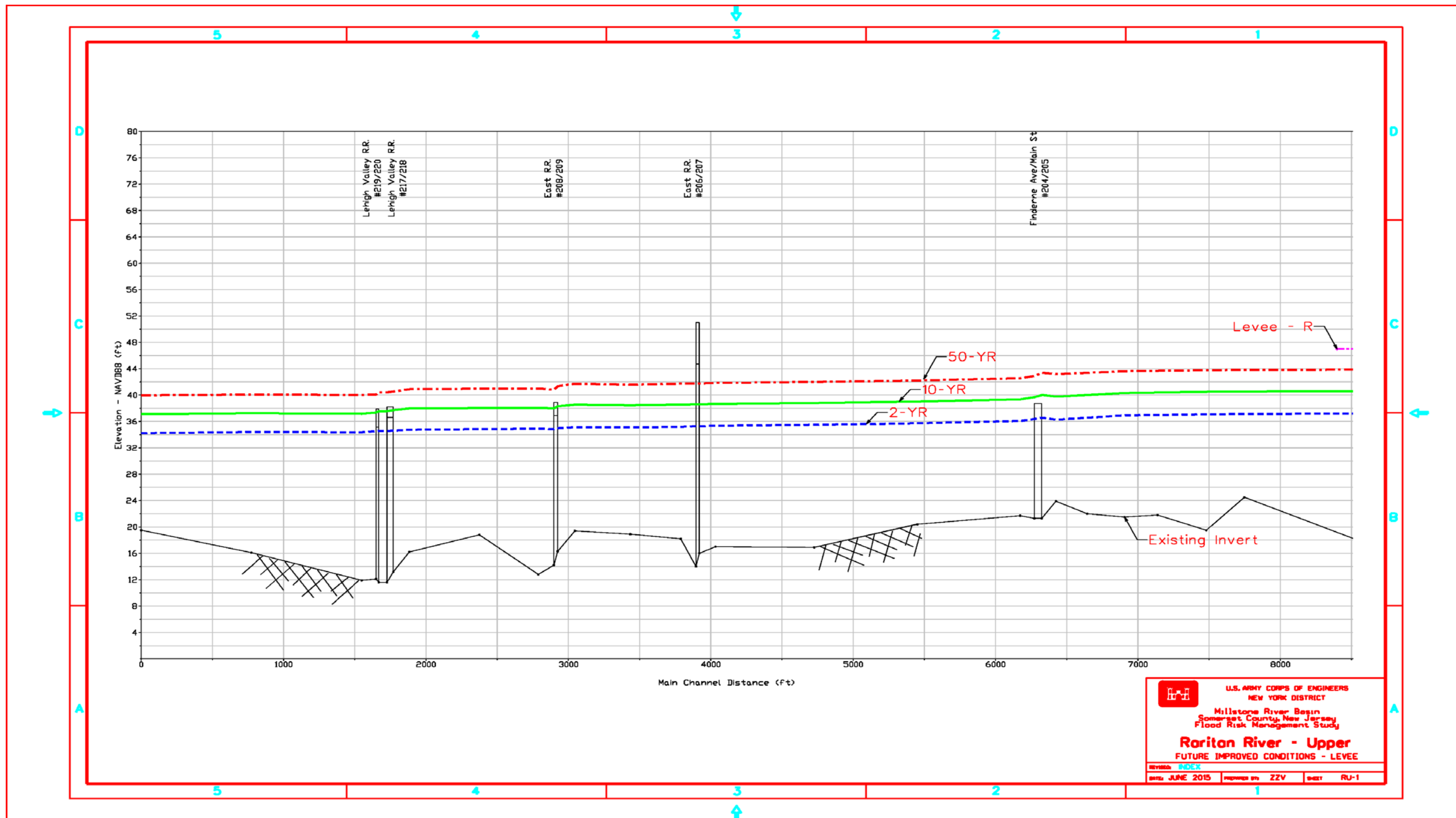
FIGURE 64: MAXIMUM WATER SURFACE PROFILE FOR LEVEE & FLOODWALL PLAN - FUTURE IMPROVED CONDITIONS (RARITAN RIVER UPPER)
