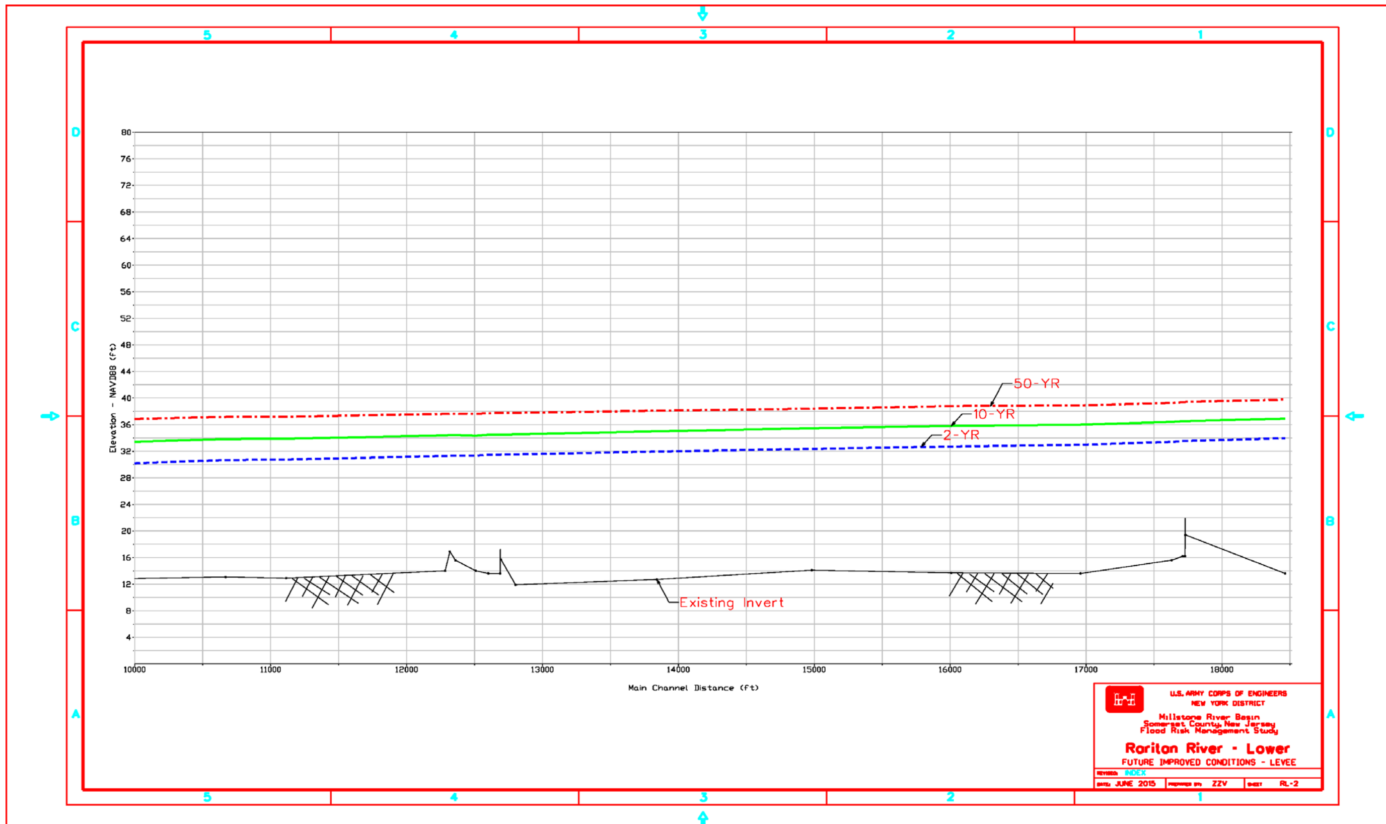
FIGURE 65: MAXIMUM WATER SURFACE PROFILE FOR LEVEE & FLOODWALL PLAN - FUTURE IMPROVED CONDITIONS (RARITAN RIVER LOWER)
