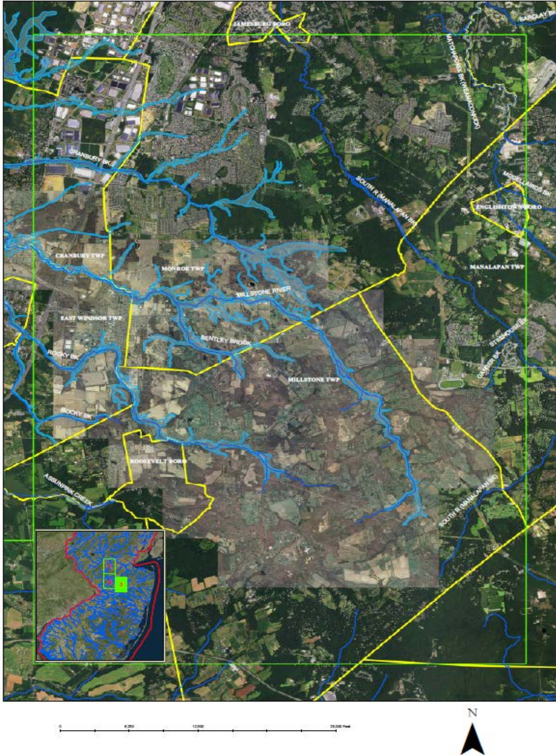
Figure 3: Millstone River Basin with 1% Annual Chance Exceedance Floodplain
