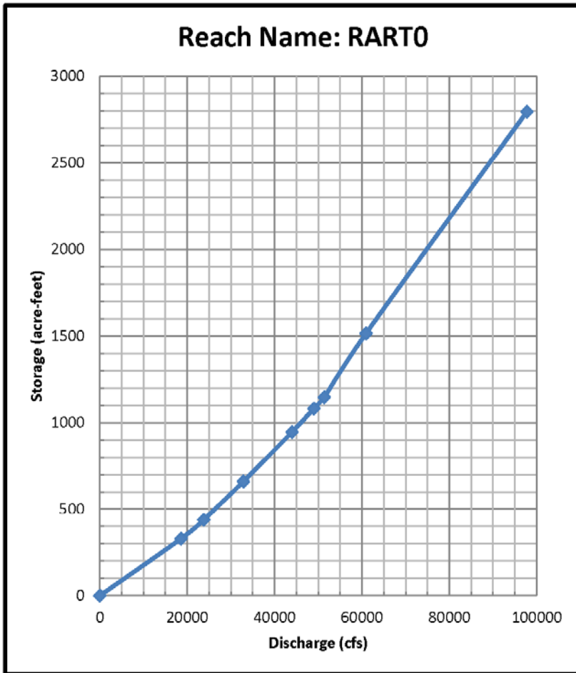
FIGURE 4 (D): MODIFIED PULS ROUTING RELATIONS
