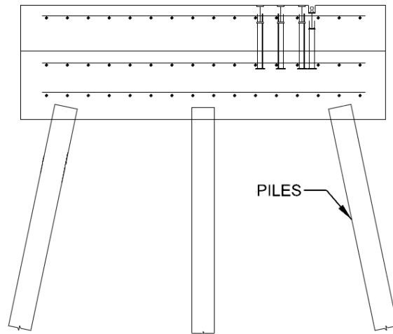
Figure 8: Typical Elevation of a Foundation for a Closure Gate
