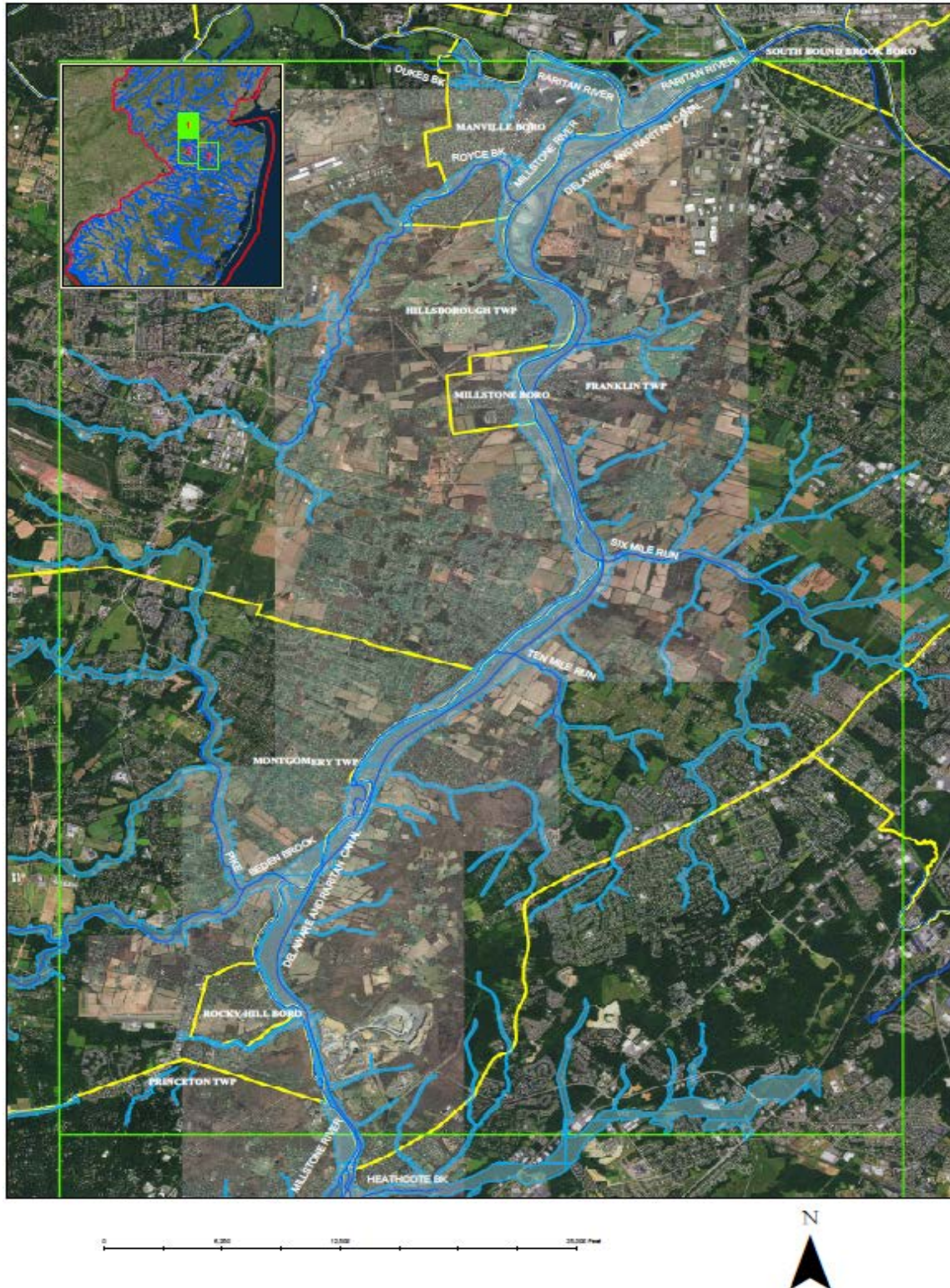
Figure 1. Millstone River Basin with 1% Annual Chance Exceedance Floodplain
