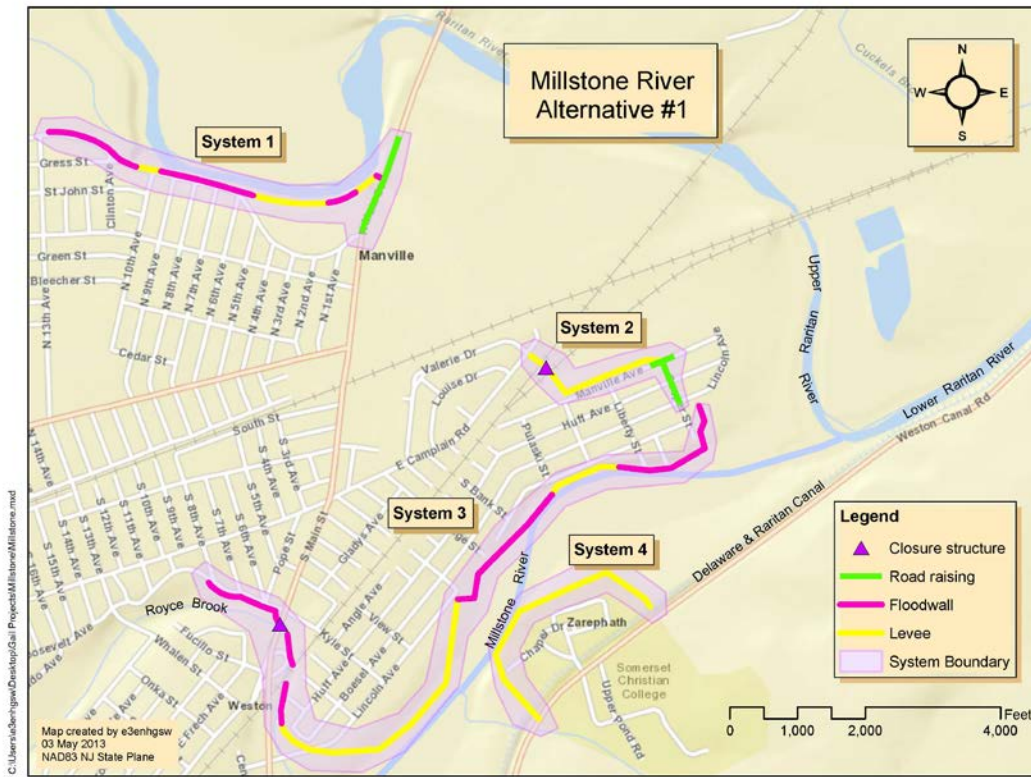
Figure 7: Alternative 1 – Levees and Floodwalls
