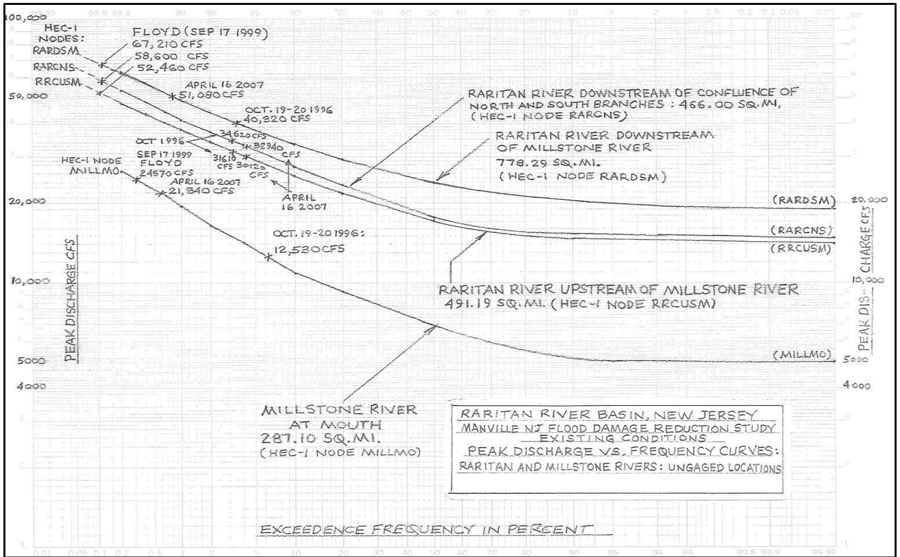
FIGURE 16: PEAK DISCHARGE VS. FREQUENCY CURVE AT NODES ALONG RARITAN AND MILLSTONE RIVERS
