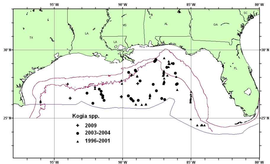
Figure 1. Distribution of pygmy and dwarf sperm whale sightings from SEFSC vessel surveys during spring 1996-2001, summer 2003 and spring 2004, and summer 2009. All the on-effort sightings are shown, though not all were used to estimate abundance. Solid lines indicate the 100m and 1,000m isobaths and the offshore extent of the U.S. EEZ.
