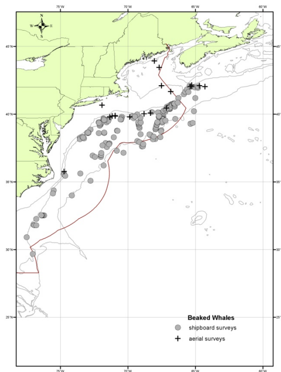
Figure 1. Distribution of beaked whale sightings from NEFSC and SEFSC shipboard and aerial surveys during the summers of 1995, 1998, 1999, 2002, 2004, 2006 and, 2007, 2008, 2010 and 2011. Isobaths are the 100-m, 1000-m and 4000-m depth contours.
